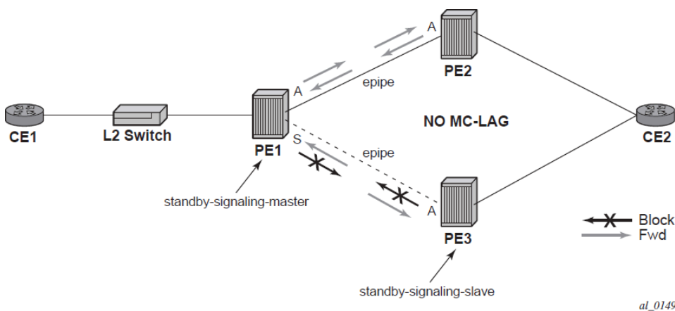
Figure 37: Master-slave pseudowire redundancy
