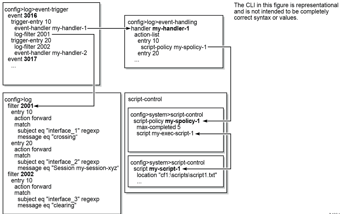
Figure 10: EHS object relationships
