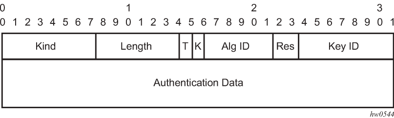
Figure 5: Packet format
