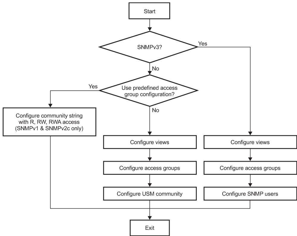
Figure 6: SNMPv1 and SNMPv2c configuration and implementation flow
