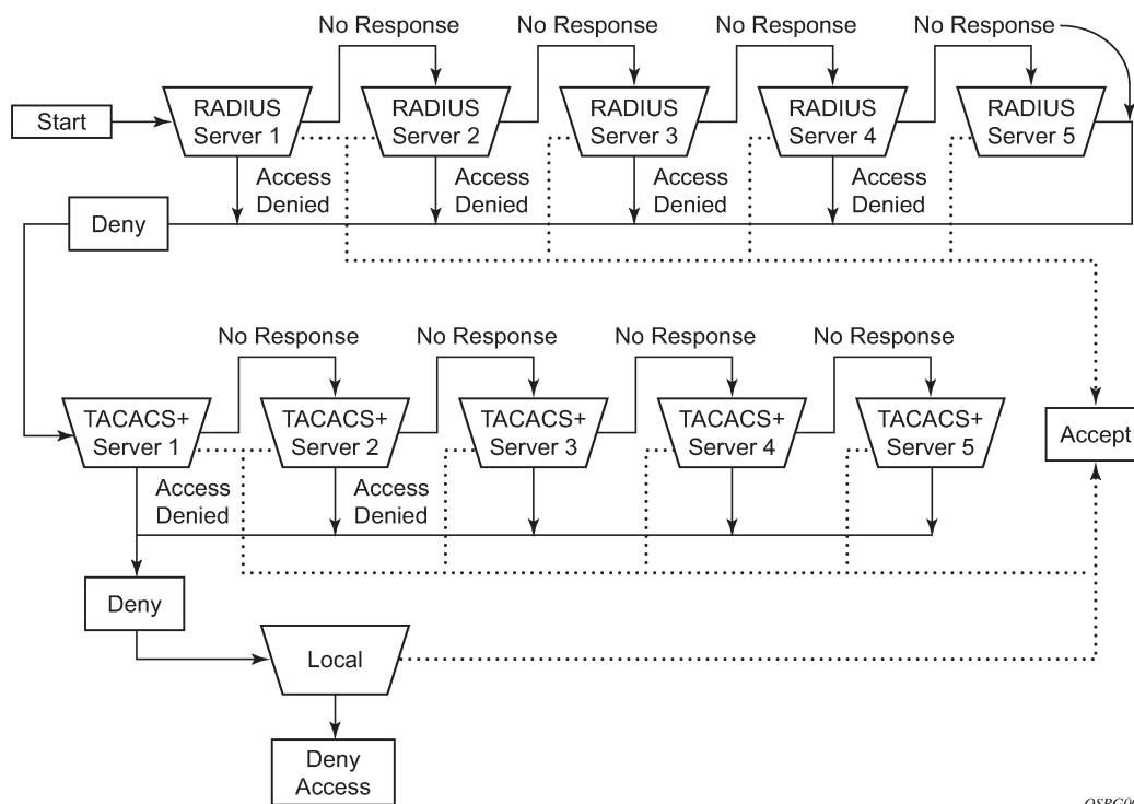
Figure 3: Security flow
