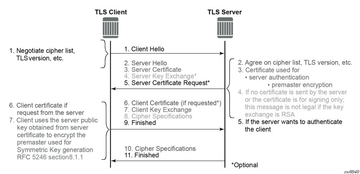
Figure 11: TLS handshake
