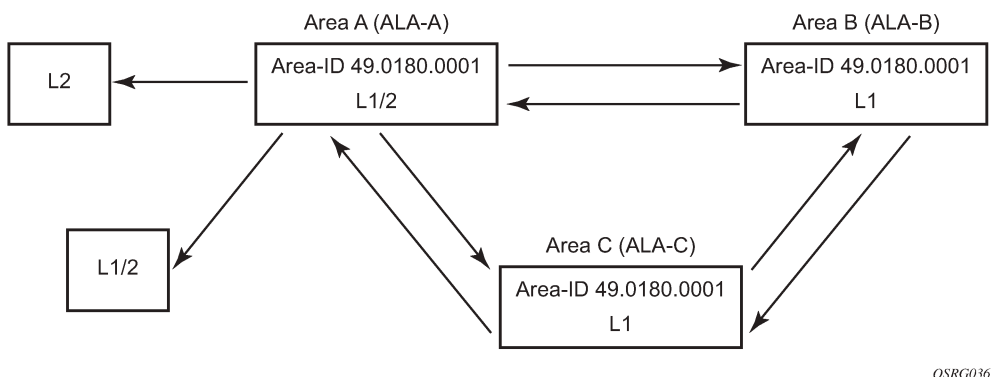
Figure 23: Configuring a Level 1/2 area
