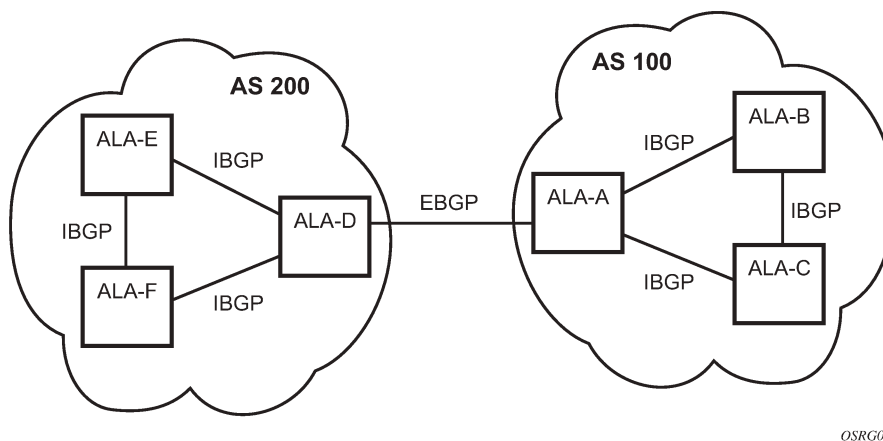
Figure 24: BGP configuration
