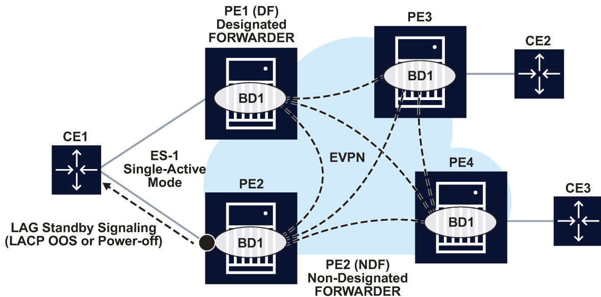
Figure 55: LACP standby signaling from the non-DF
