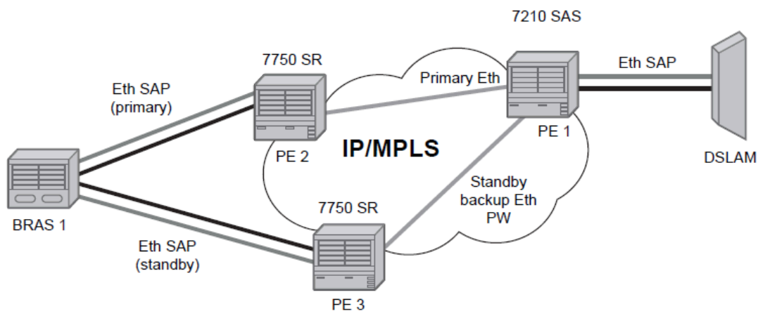
Figure 20: VLL resilience
