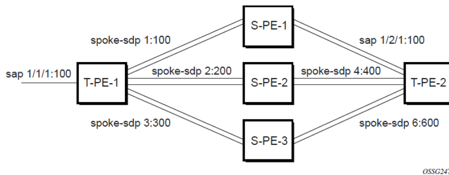
Figure 38: VLL resilience with pseudowire switching
