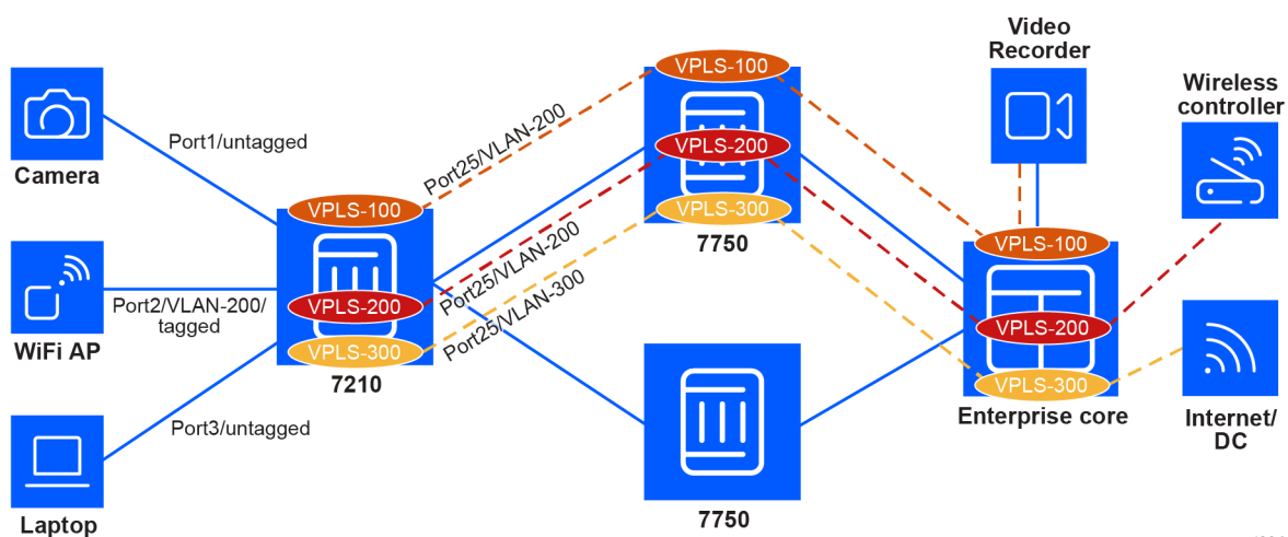
Figure 15: Dynamic VLAN assignment using dot1x in enterprise
