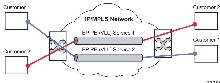
Figure 17: Epipe/VLL service
