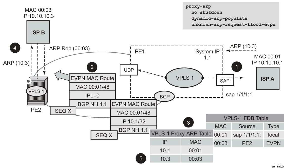
Figure 56: Proxy-ARP example usage in an EVPN network
