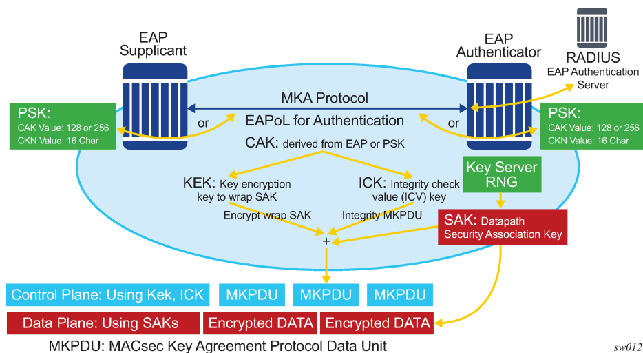
Figure 6: MACsec generating the CAK
