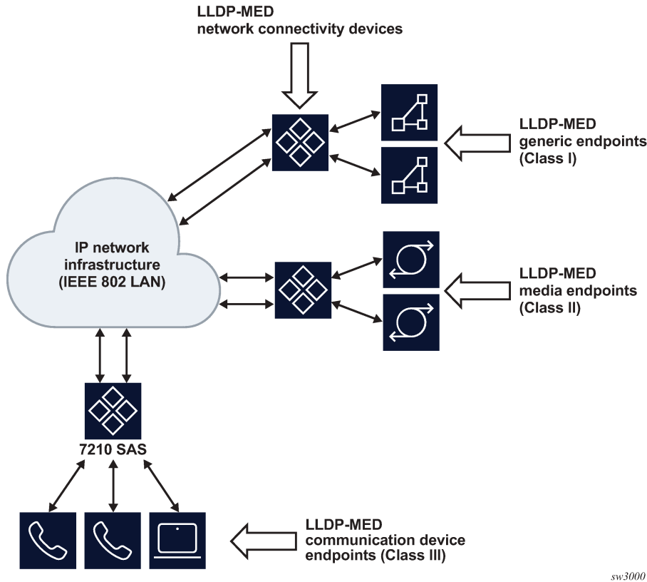
Figure 12: LLDP-MED reference model
