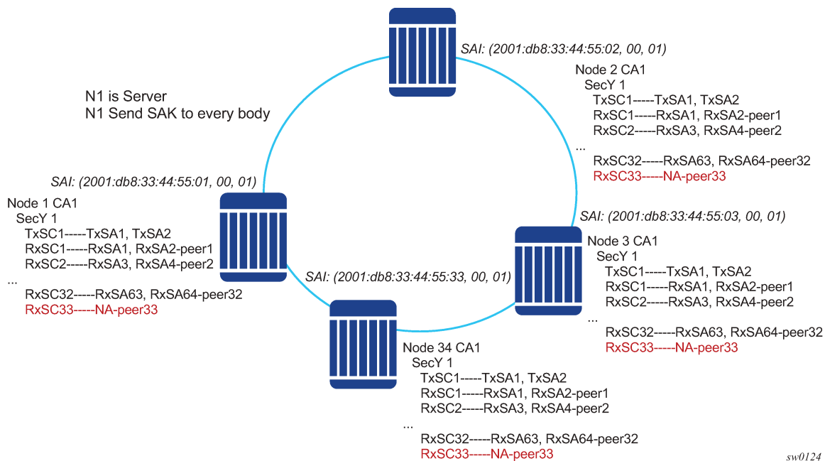
Figure 9: P2MP topology
