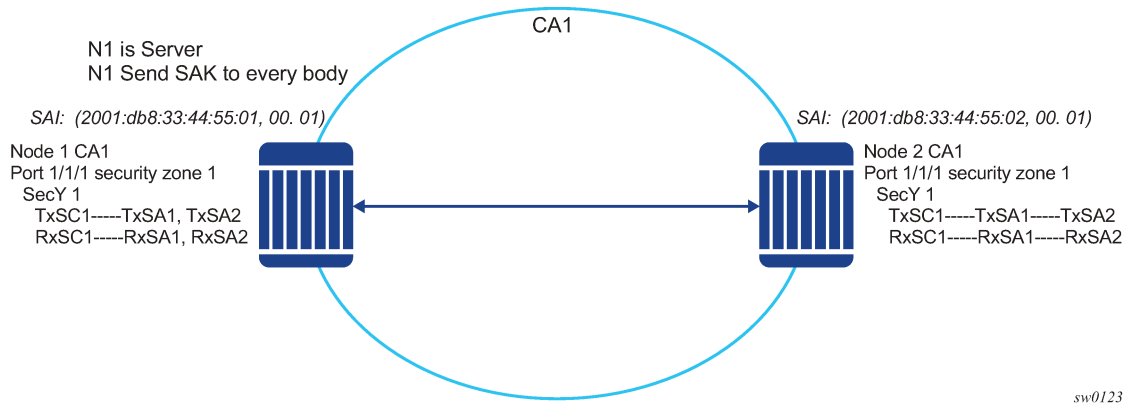
Figure 8: P2P (switch-to-switch) topology
