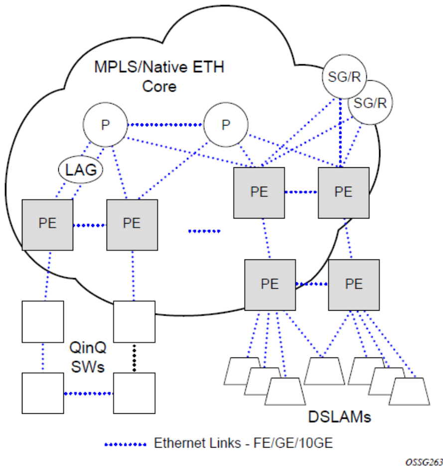
Figure 11: Generic customer use case for LLDP
