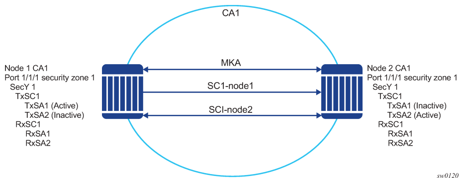
Figure 4: MACsec concepts for static-CAK
