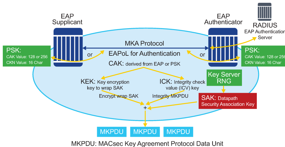
Figure 7: MACsec control plane
