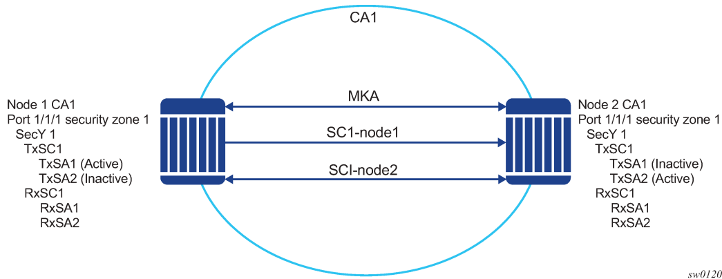
Figure 5: MACsec concepts for static CAK
