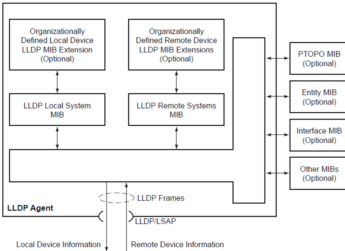
Figure 10: LLDP internal architecture for a network node
