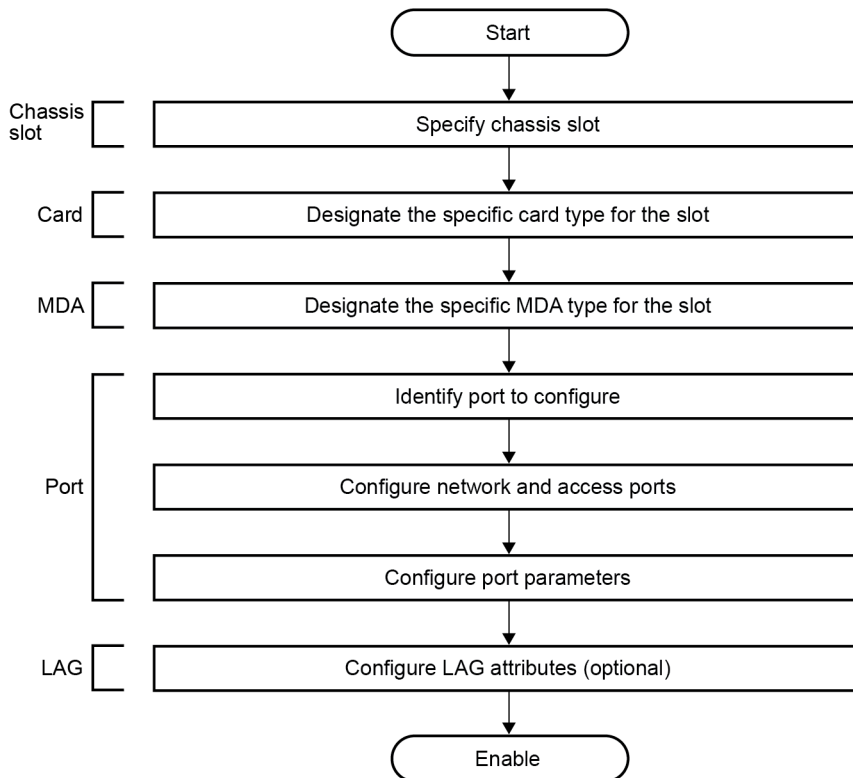
Figure 18: Slot, card, MDA, and port configuration and implementation flow
