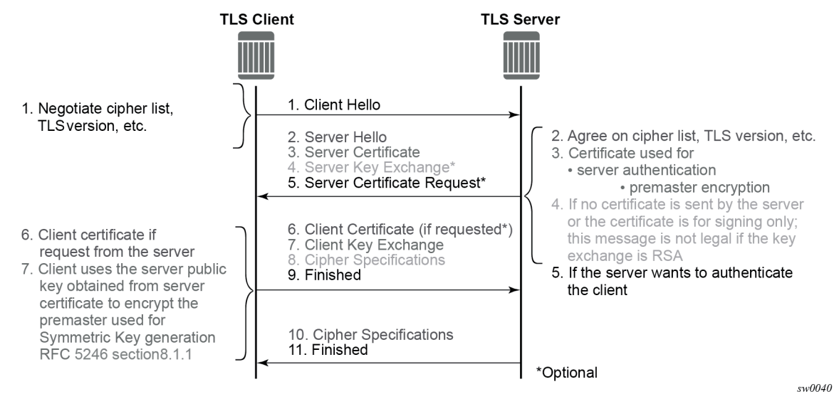
Figure 10: TLS handshake
