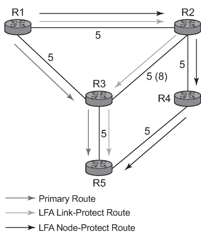
Figure 12: Topology with primary and LFA routes
