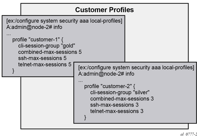
Figure 10: MD-CLI session groups for customer classes
