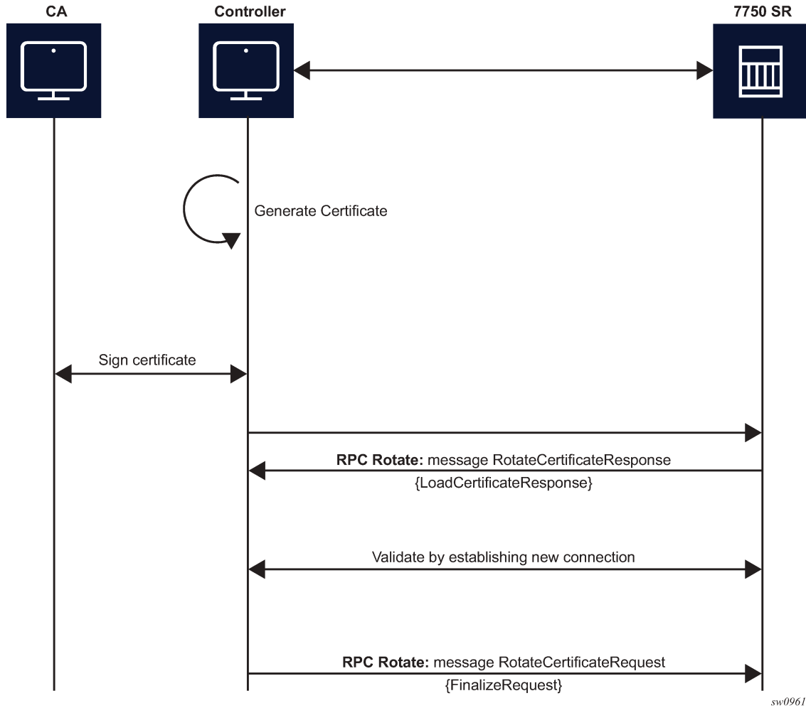
Figure 32: RPC Rotate message flow when CSRs are not generated on the SR OS node
