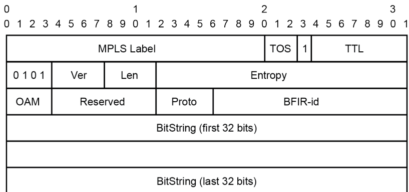
Figure 25: BIER MPLS encapsulation
