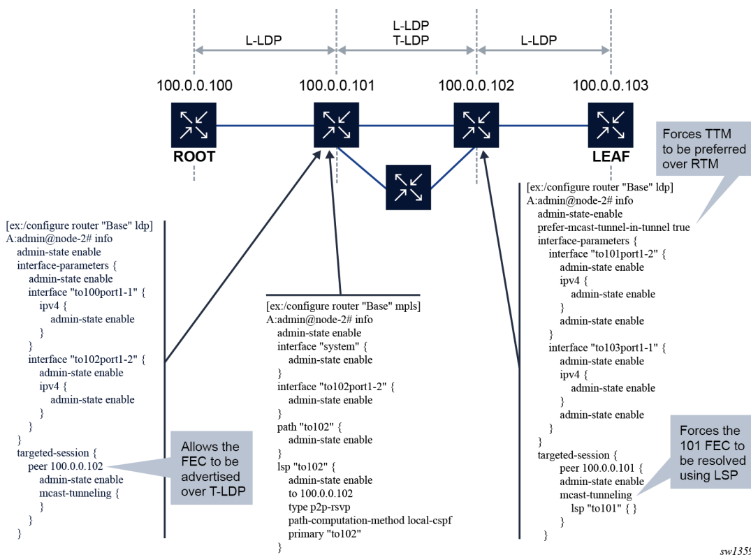
Figure 13: Configuring MLDP over RSVP P2P LSP (MD-CLI)
