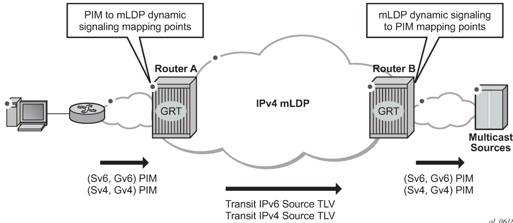
Figure 8: Dynamic MLDP signaling for IP multicast in GRT
