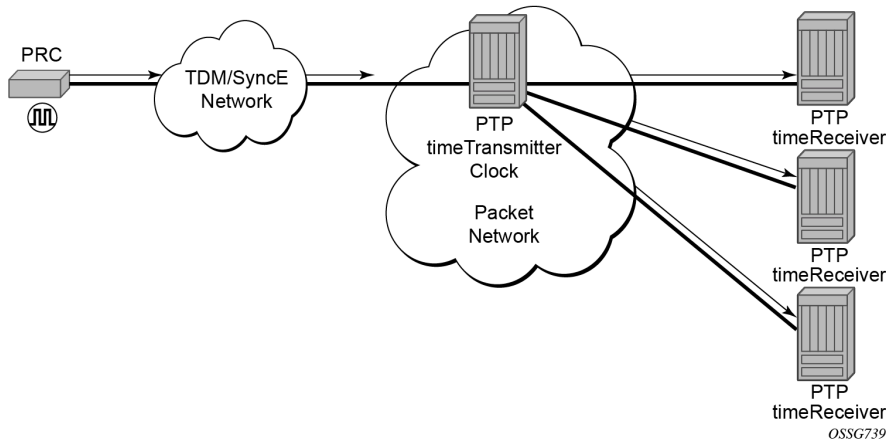
Figure 24: PTP timeTransmitter clock
