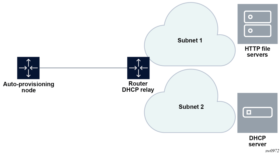
Figure 10: Auto-provisioning with all components in different subnets
