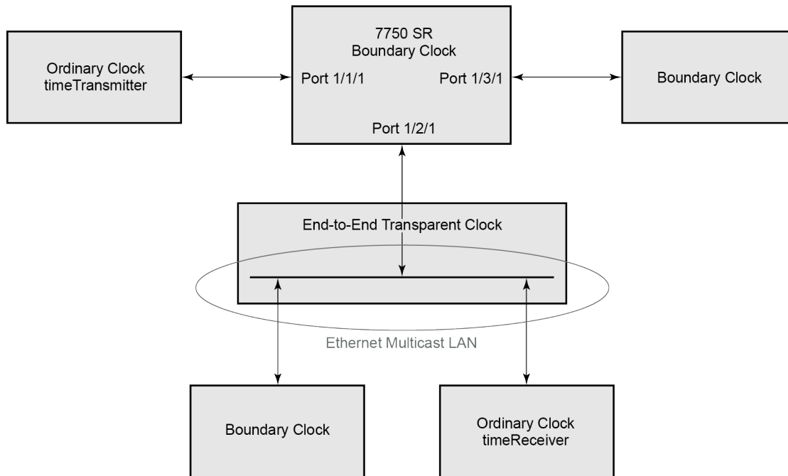
Figure 18: Ethernet multicast ports
