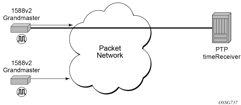
Figure 22: timeReceiver clock
