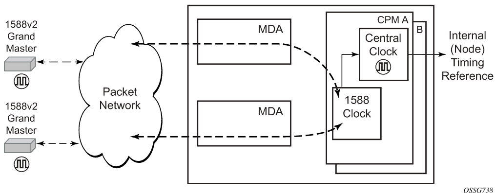
Figure 23: Ordinary timeReceiver clock operation
