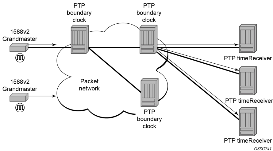
Figure 26: Boundary clock
