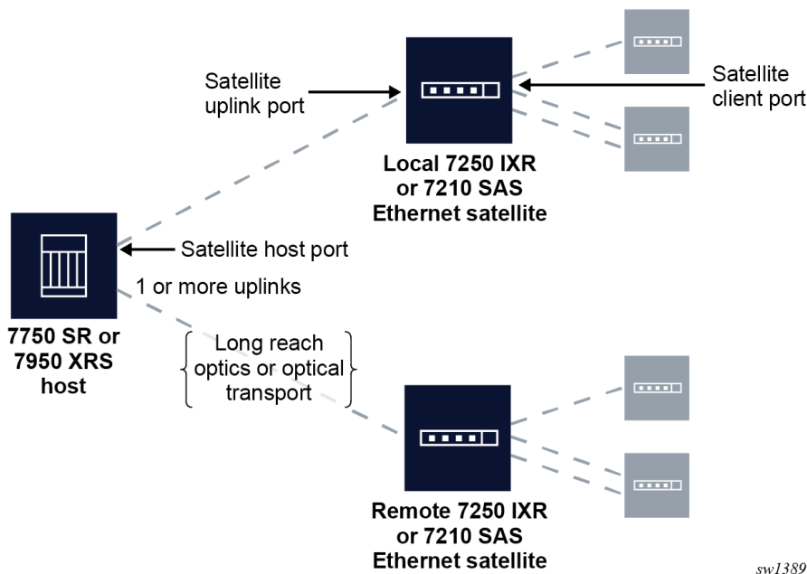
Figure 29: Satellite solution capabilities
