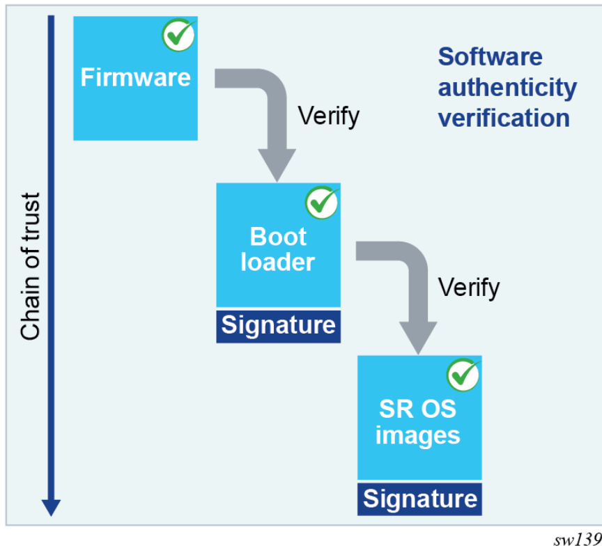
Figure 7: Secure boot chain of trust
