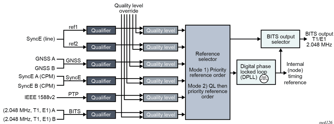
Figure 16: CPM clock synchronization reference selection
