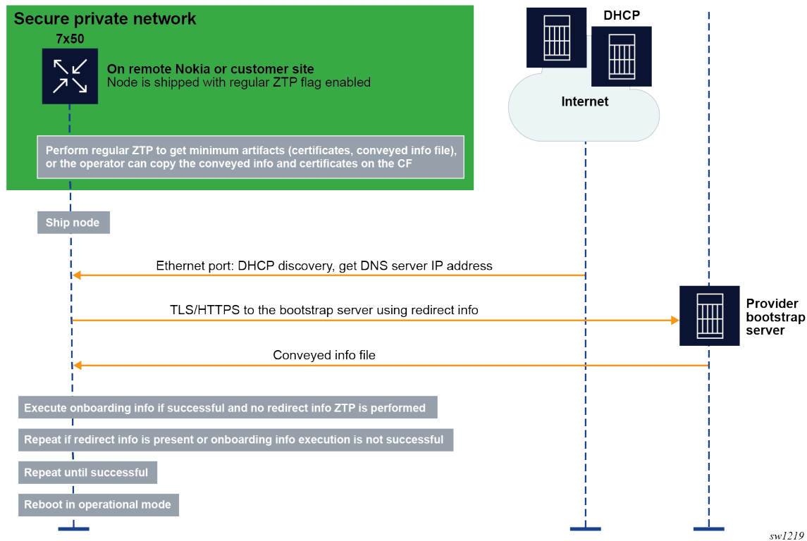
Figure 11: SZTP process
