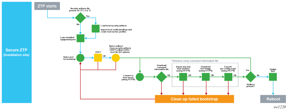
Figure 12: Installation site SZTP process
