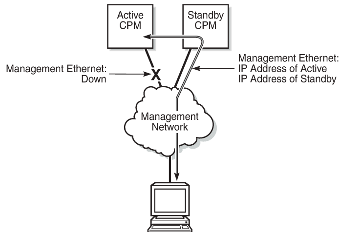
Figure 14: Management Ethernet: redundancy mode
