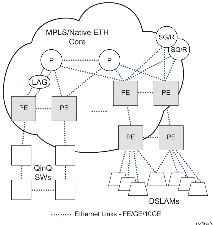
Figure 28: Customer use example for LLDP
