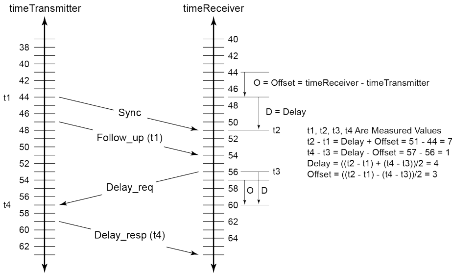
Figure 20: PTP timeReceiver and timeTransmitter time synchronization computation
