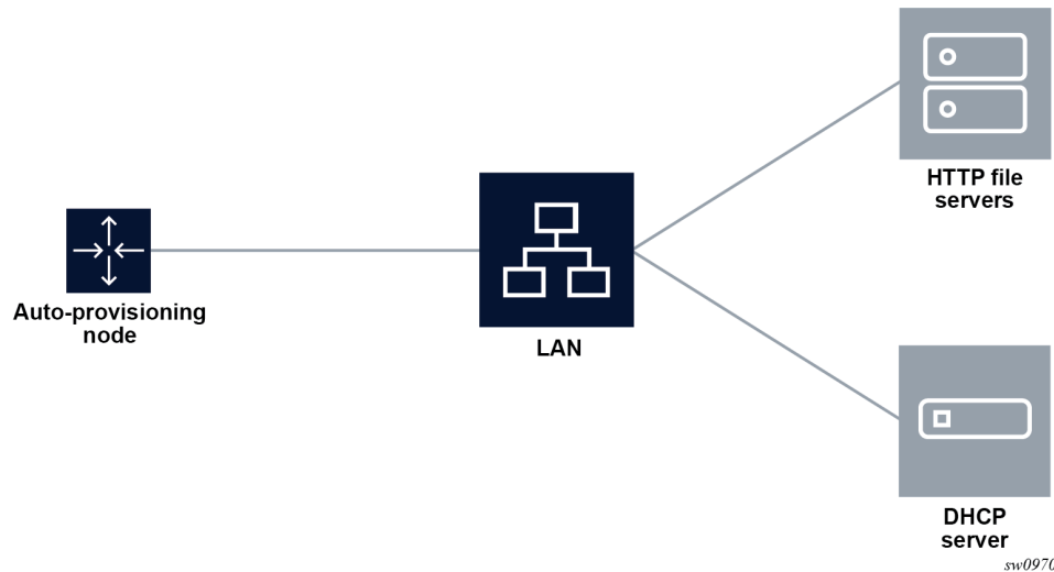
Figure 8: Auto-provisioning with all components in a Layer 2 broadcast domain
