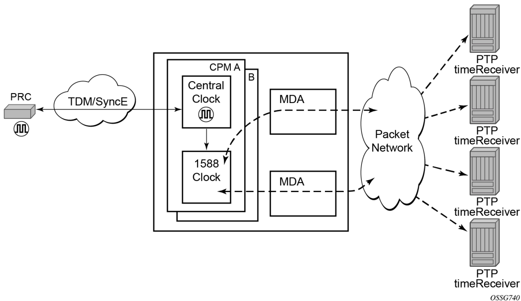
Figure 25: Ordinary timeTransmitter clock operation
