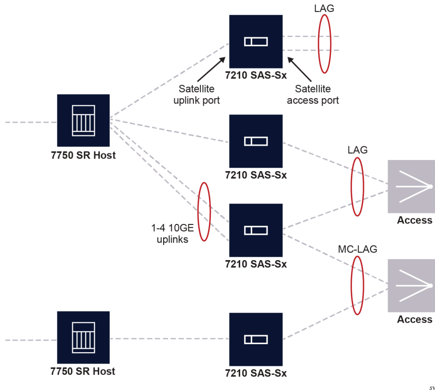
Figure 31: Ethernet LAGs with satellite member links
