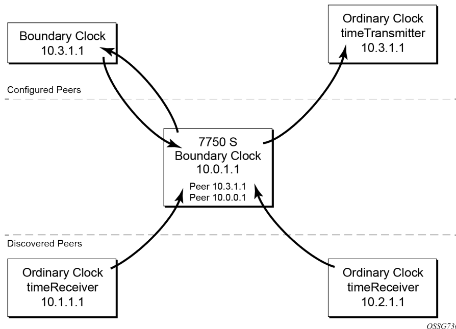
Figure 17: Peer clocks
