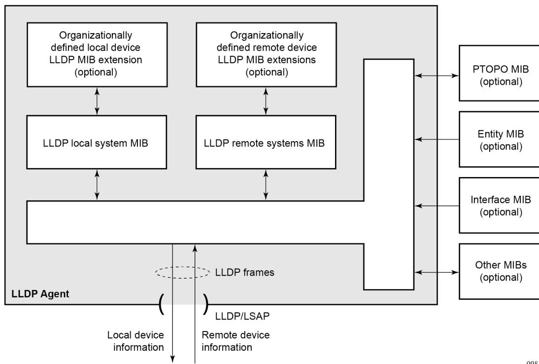
Figure 27: LLDP internal architecture for a network node
