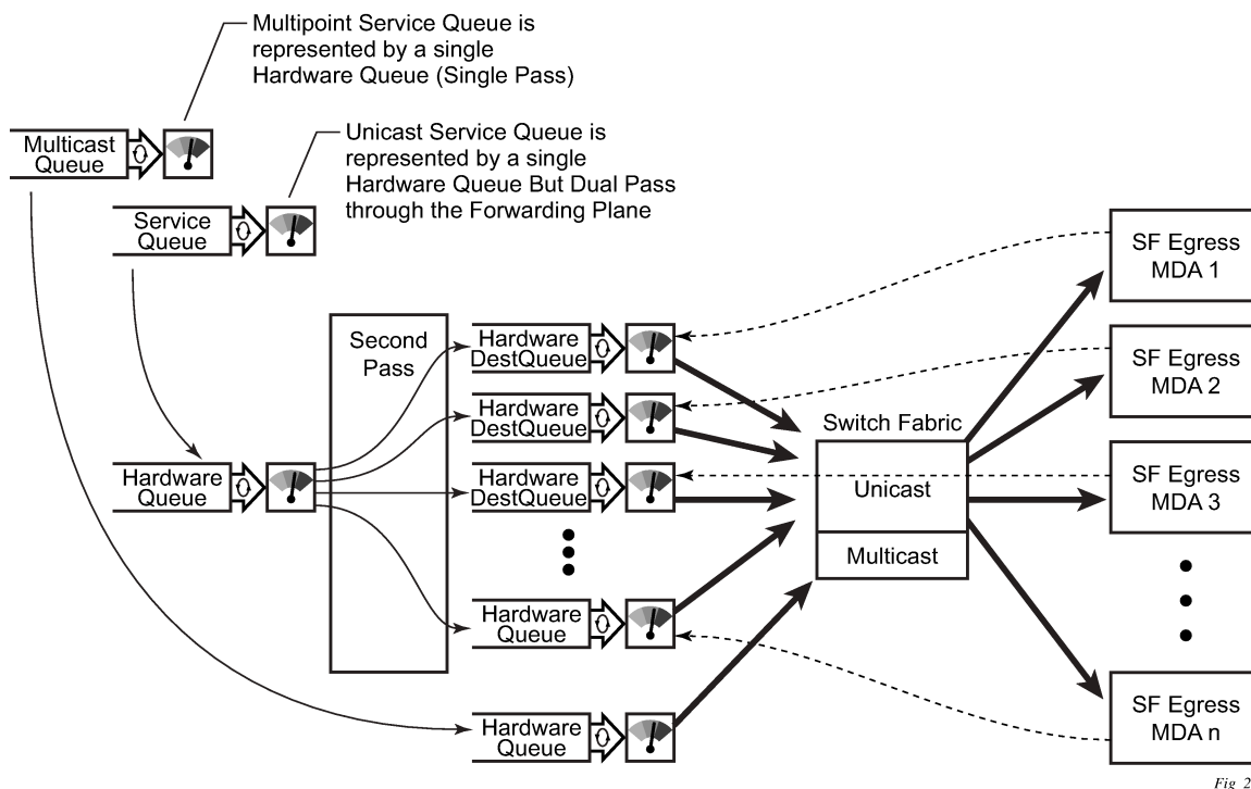
Figure 41: Multipoint queue behavior with shared queuing enabled
