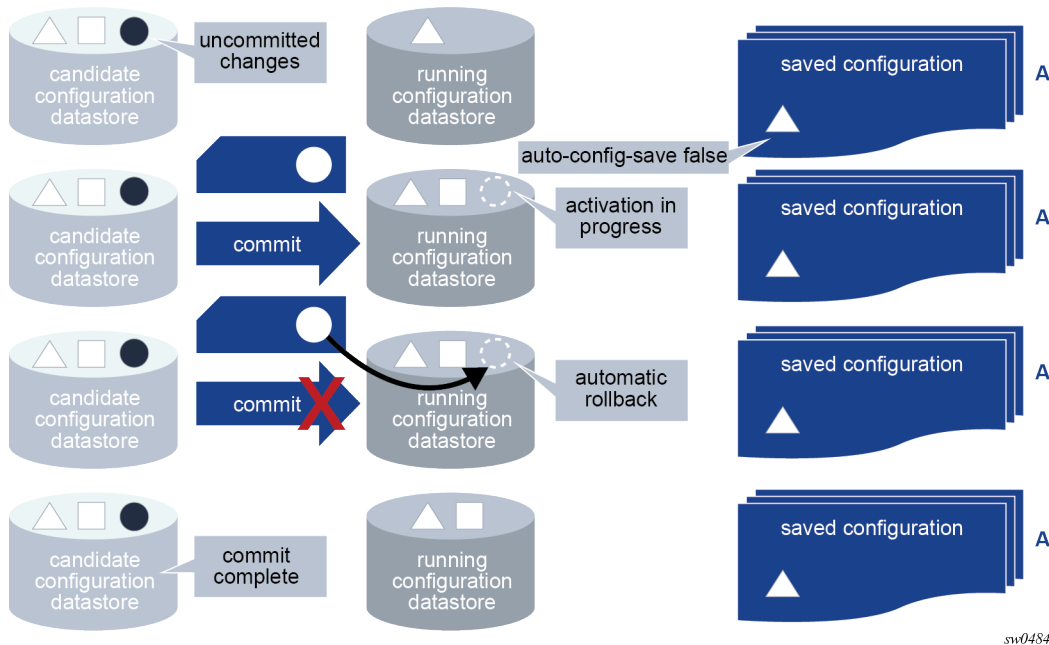
Figure 9: Failed commit
