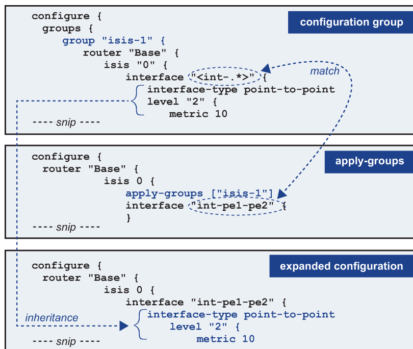
Figure 10: Configuration Groups
