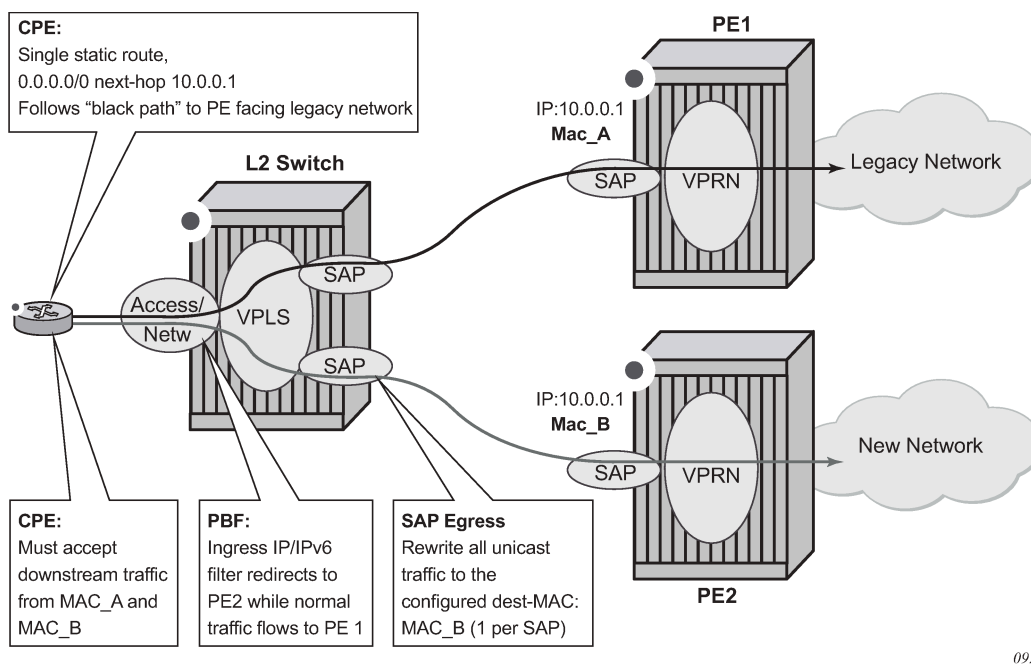
Figure 23: Layer 2 policy-based forwarding (PBF) redirect action
