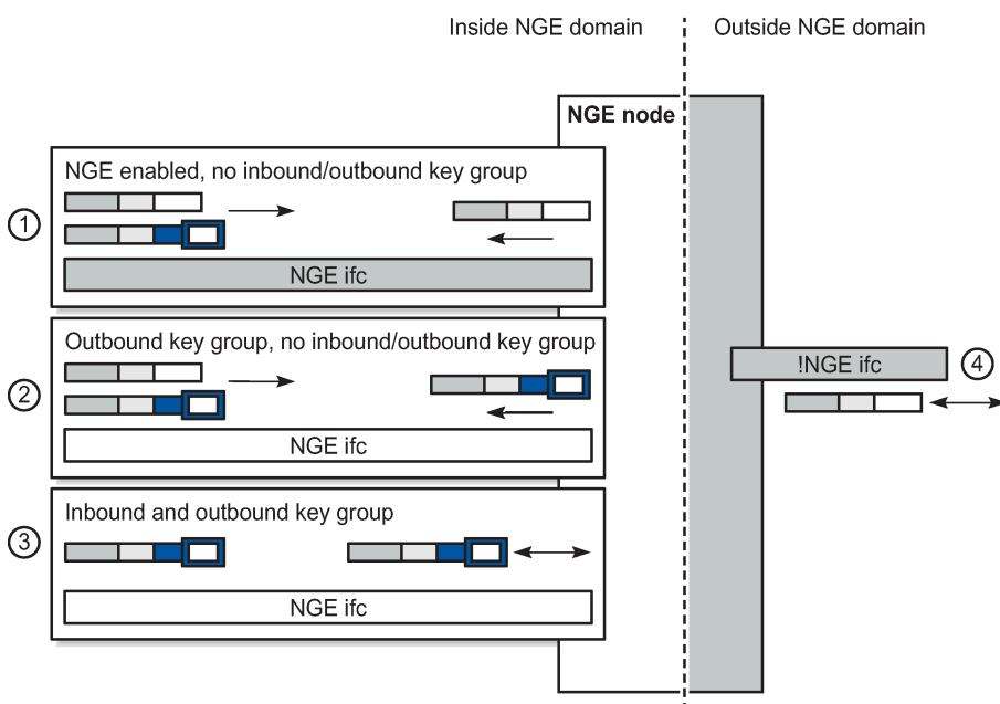
Figure 16: Inside and outside NGE domains
