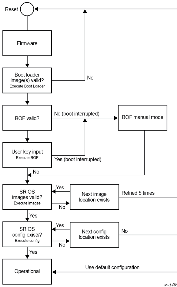
Figure 1: Boot process
