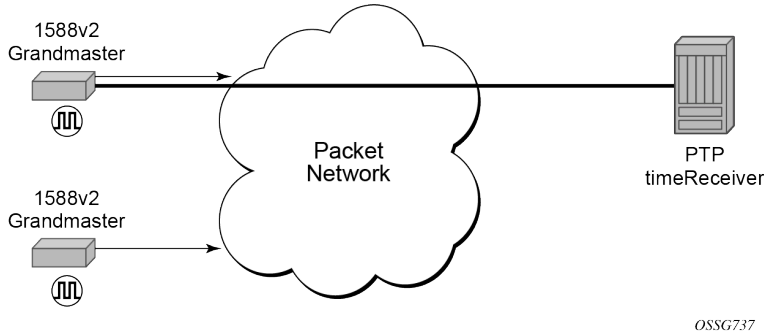
Figure 22: timeReceiver clock
