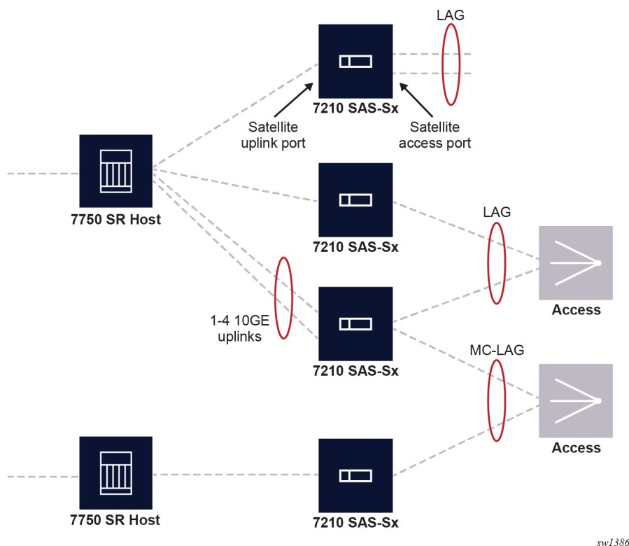
Figure 31: Ethernet LAGs with satellite member links
