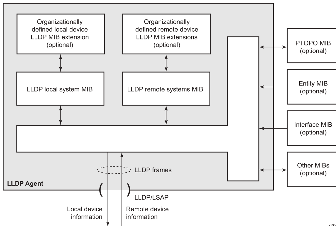
Figure 27: LLDP internal architecture for a network node
