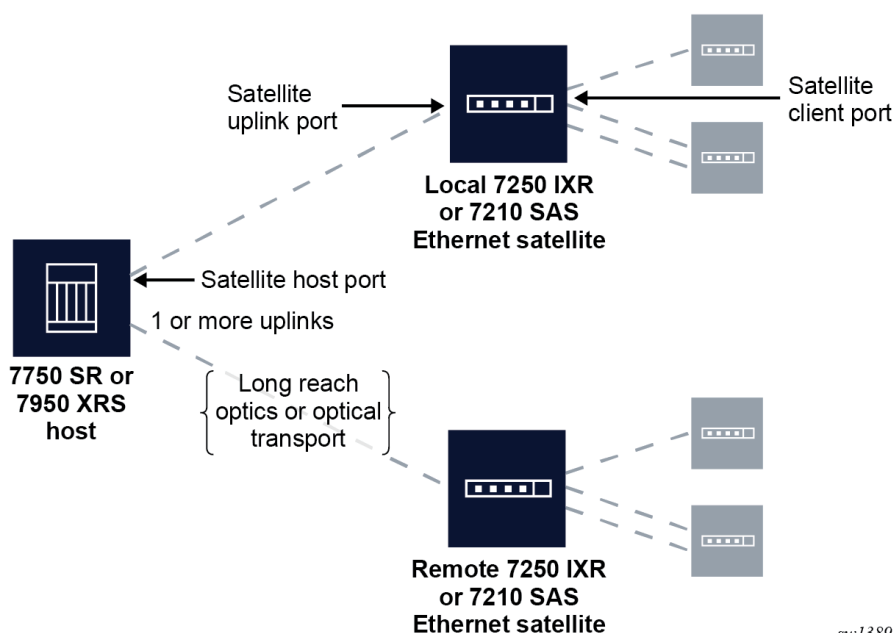
Figure 29: Satellite solution capabilities
