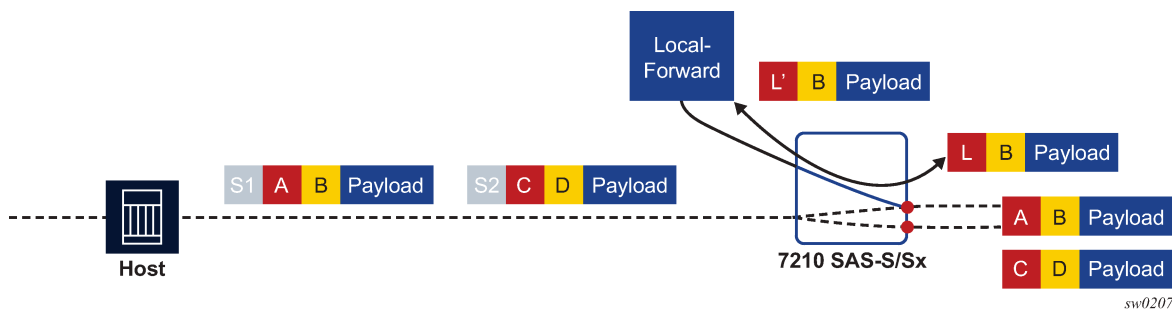
Figure 30: Local forwarding
