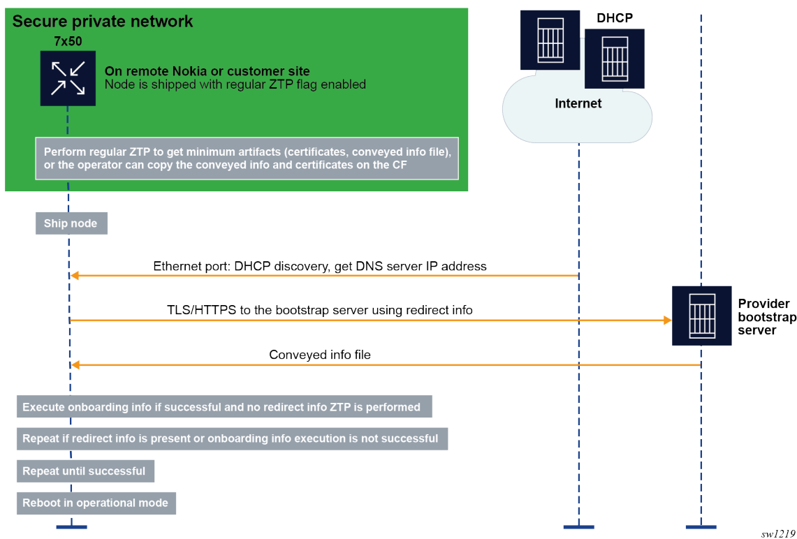
Figure 11: SZTP process
