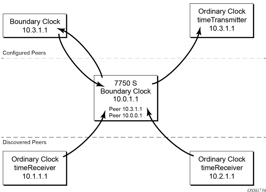
Figure 17: Peer clocks
