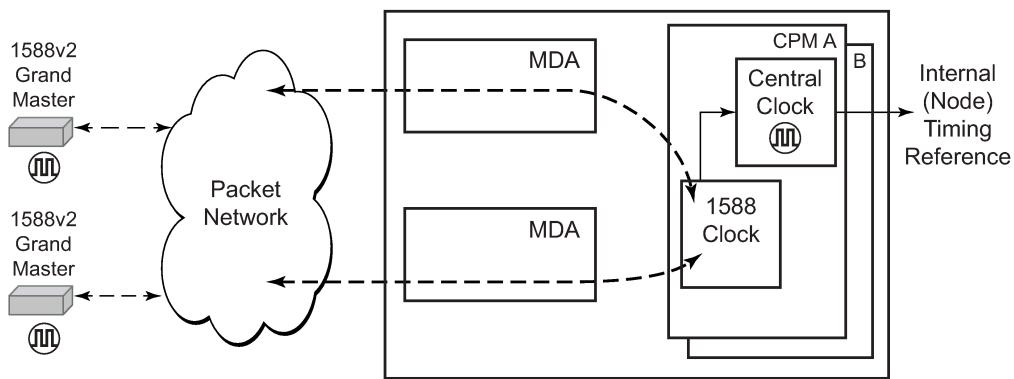
Figure 20: Ordinary timeReceiver clock operation
