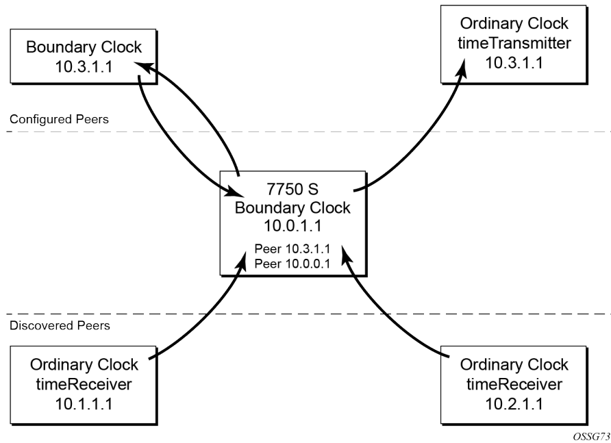
Figure 14: Peer clocks
