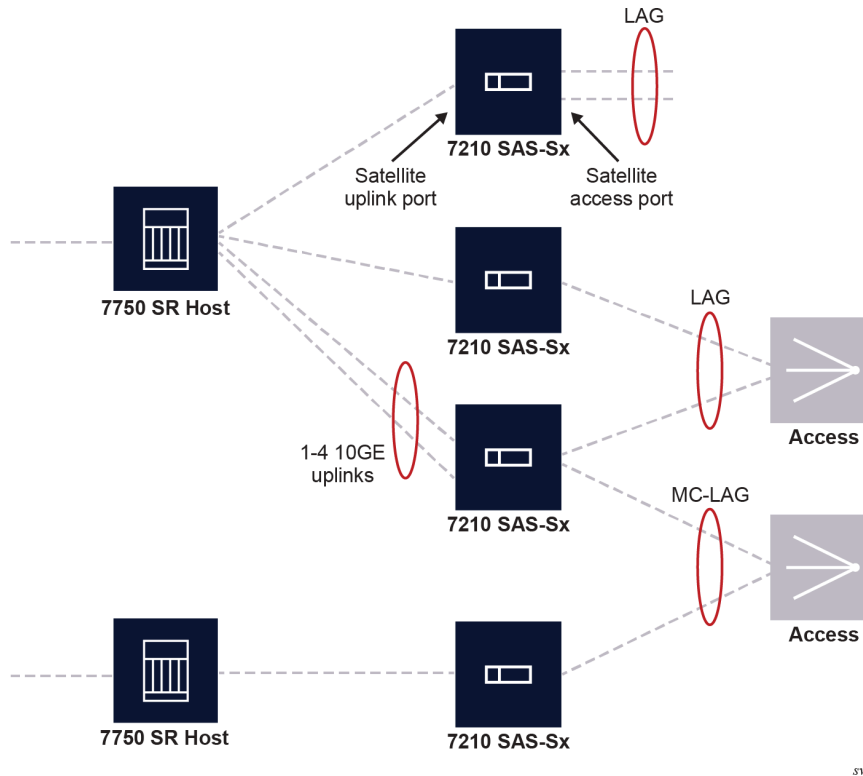
Figure 28: Ethernet LAGs with satellite member links
