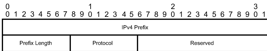
Figure 23: IPv4 IGP-prefix segment ID
