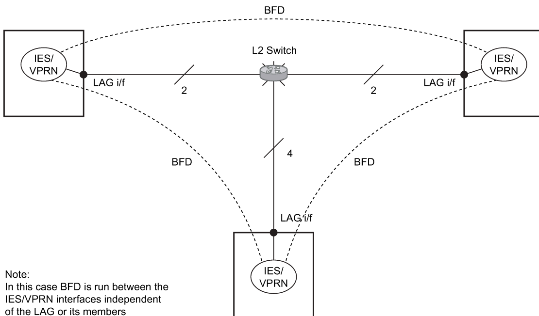
Figure 57: BFD over LAG and VSM interfaces
