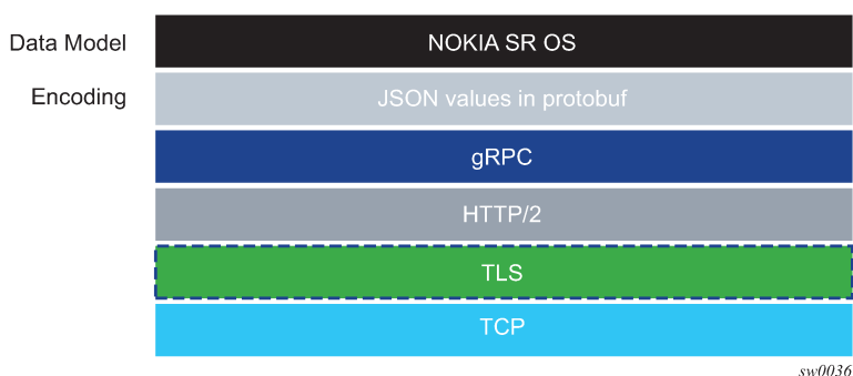
Figure 26: Protocol stack
