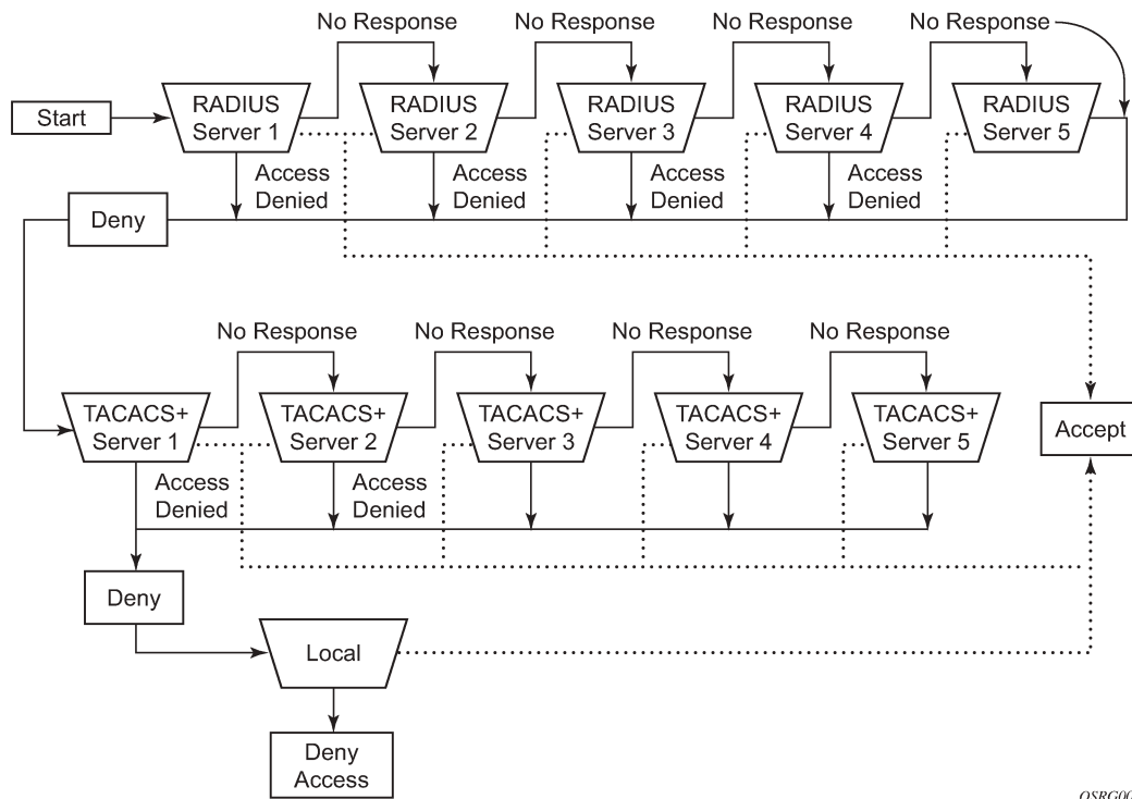
Figure 5: Security flow
