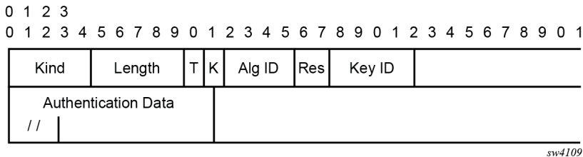
Figure 8: Packet format
