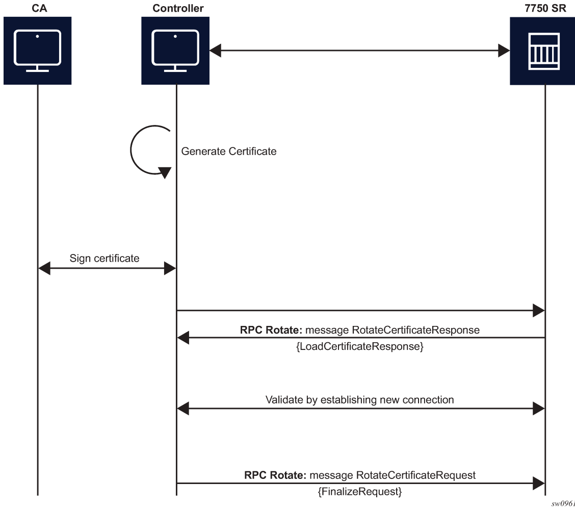
Figure 33: RPC Rotate message flow when CSRs are not generated on the SR OS node
