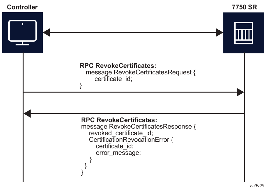
Figure 38: RPC RevokeCertificates message flow
