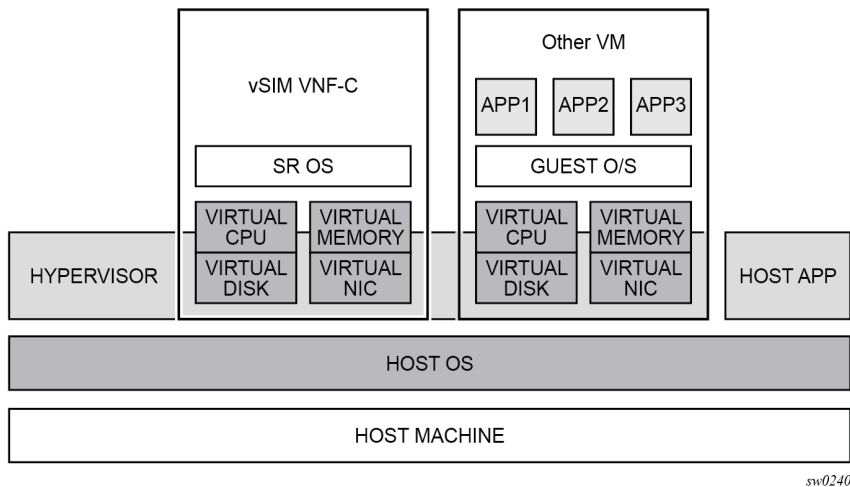
Figure 1: vSIM concept
