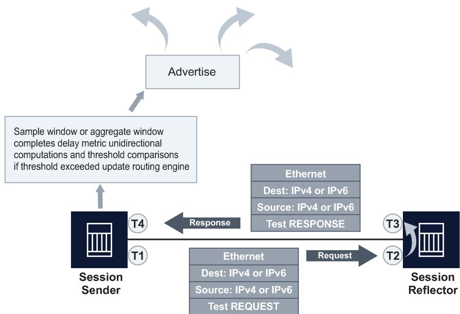
Figure 59: Link measurement interactions
