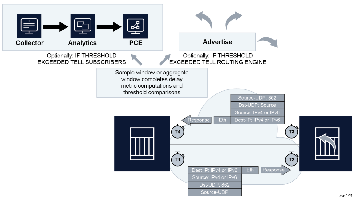
Figure 60: Link measurement interactions with reporting disabled
