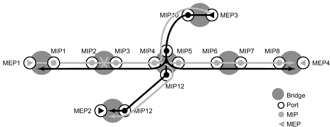
Figure 47: CFM CC
