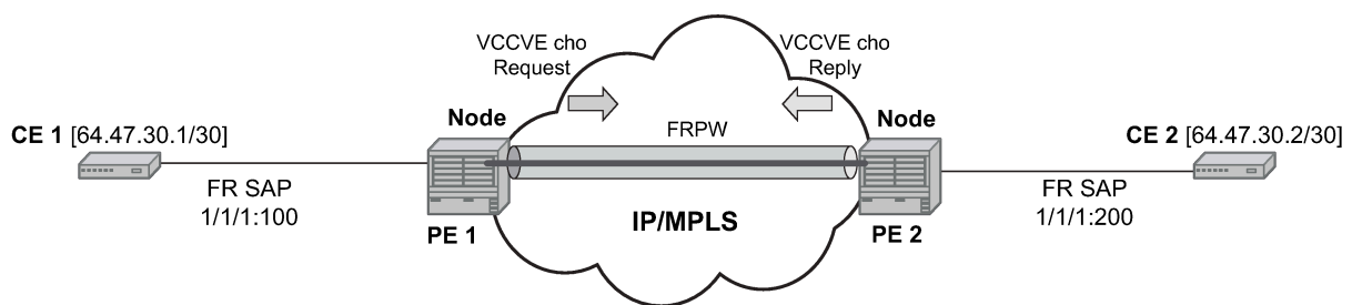
Figure 38: VCCV-ping application
