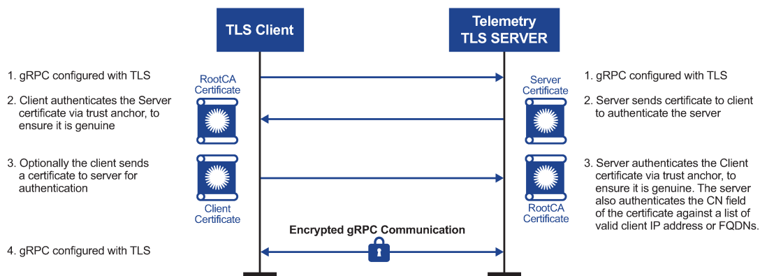
Figure 9: Session authentication using TLS
