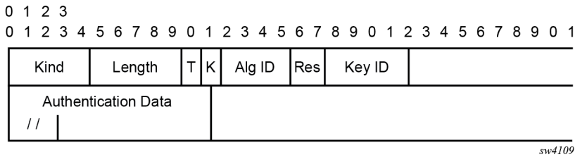
Figure 8: Packet format
