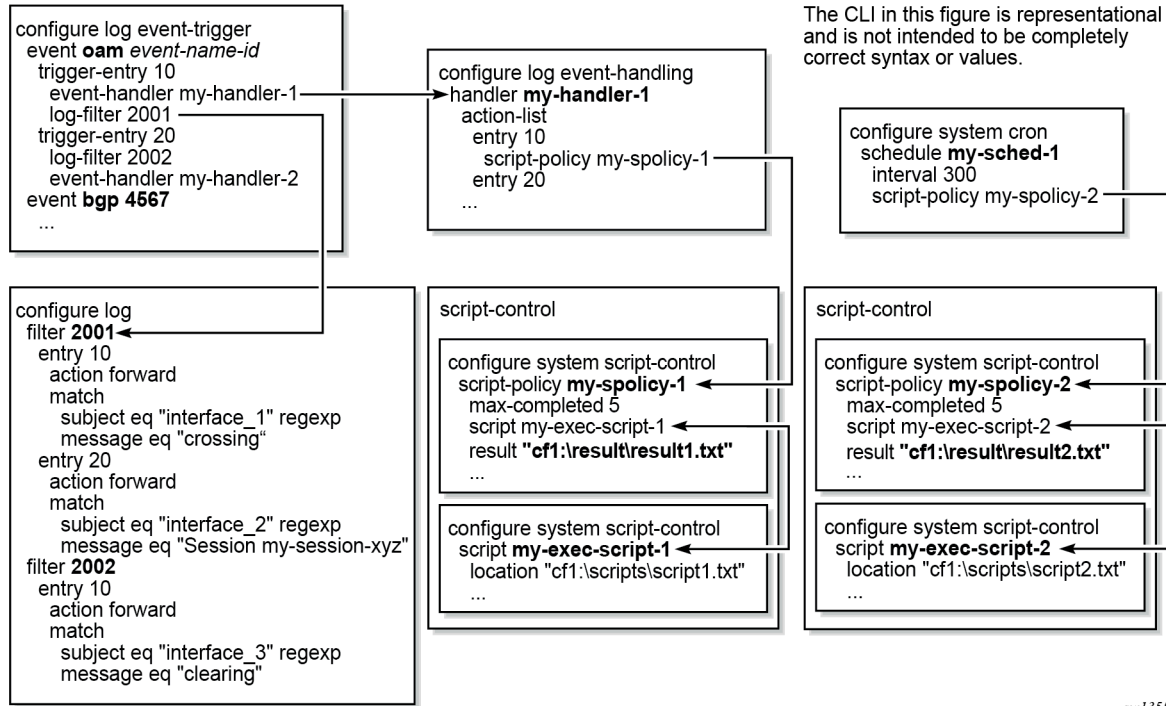
Figure 22: EHS object handling (classic CLI)
