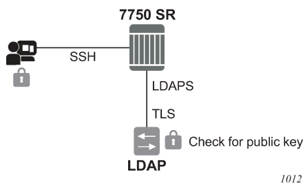
Figure 2: Key management
