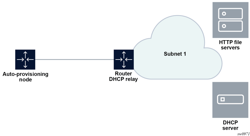
Figure 32: Auto-provisioning with only file and DHCP servers in the same subnet
