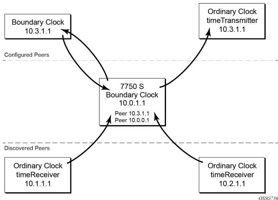
Figure 12: Peer clocks
