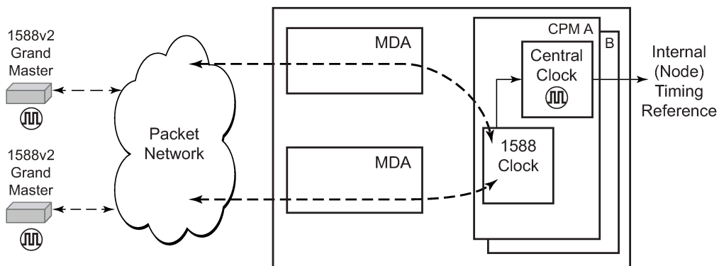
Figure 18: Ordinary timeReceiver clock operation
