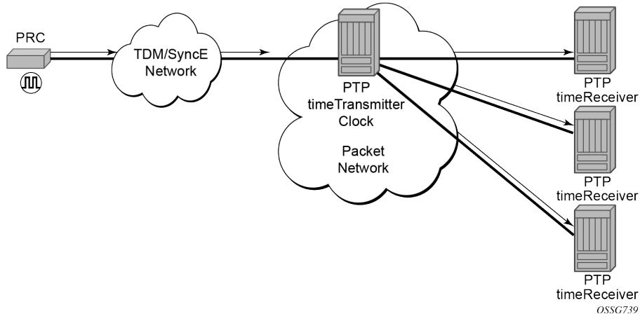
Figure 19: PTP timeTransmitter clock
