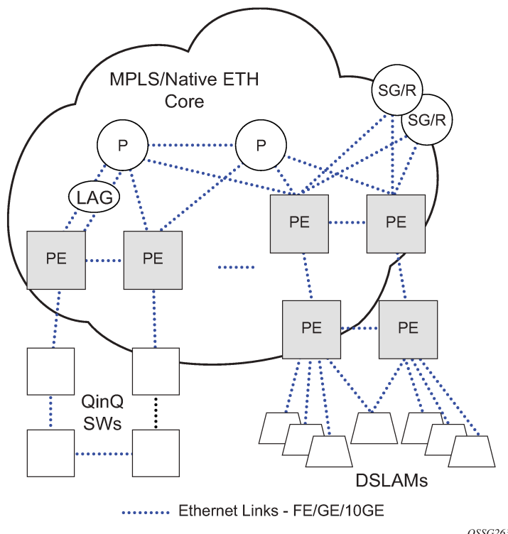
Figure 23: Customer use example for LLDP
