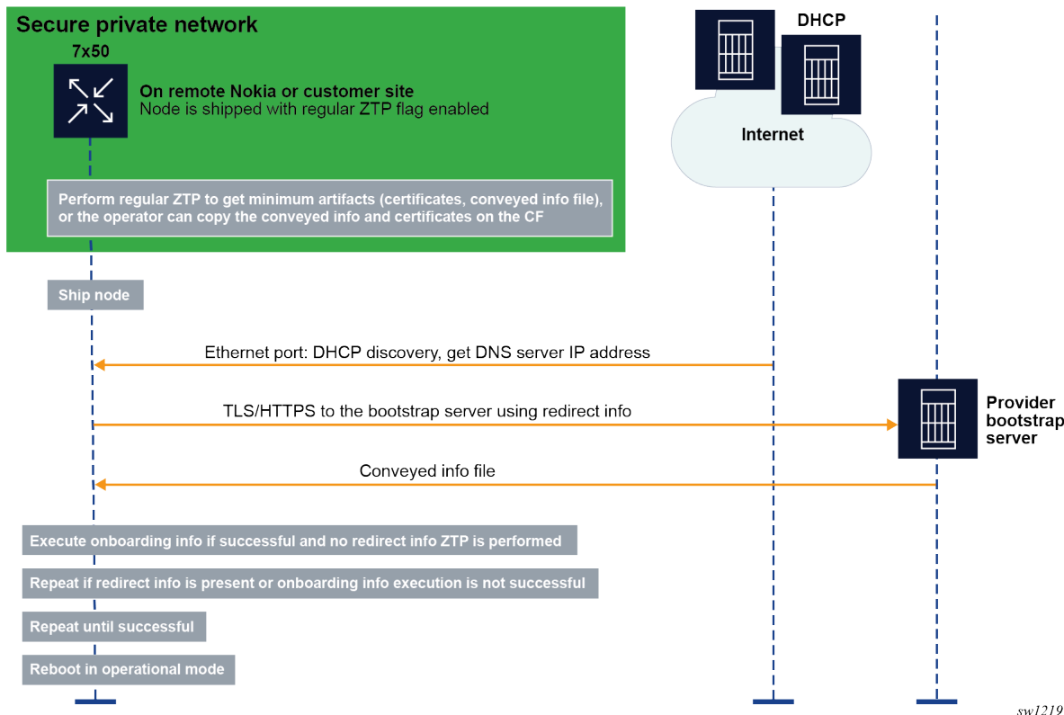
Figure 34: SZTP process
