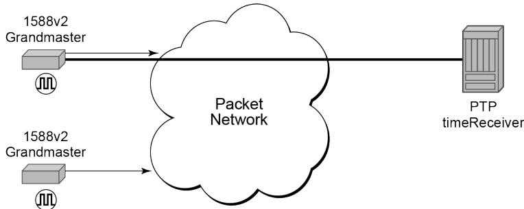
Figure 17: PTP ordinary timeReceiver clock for frequency
