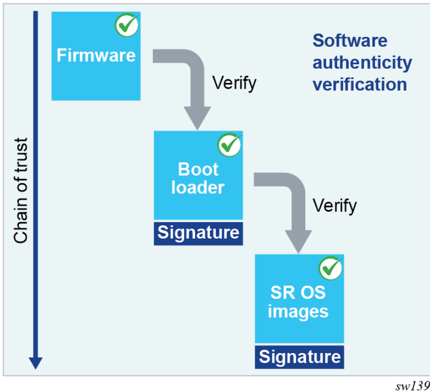
Figure 7: Secure boot chain of trust
