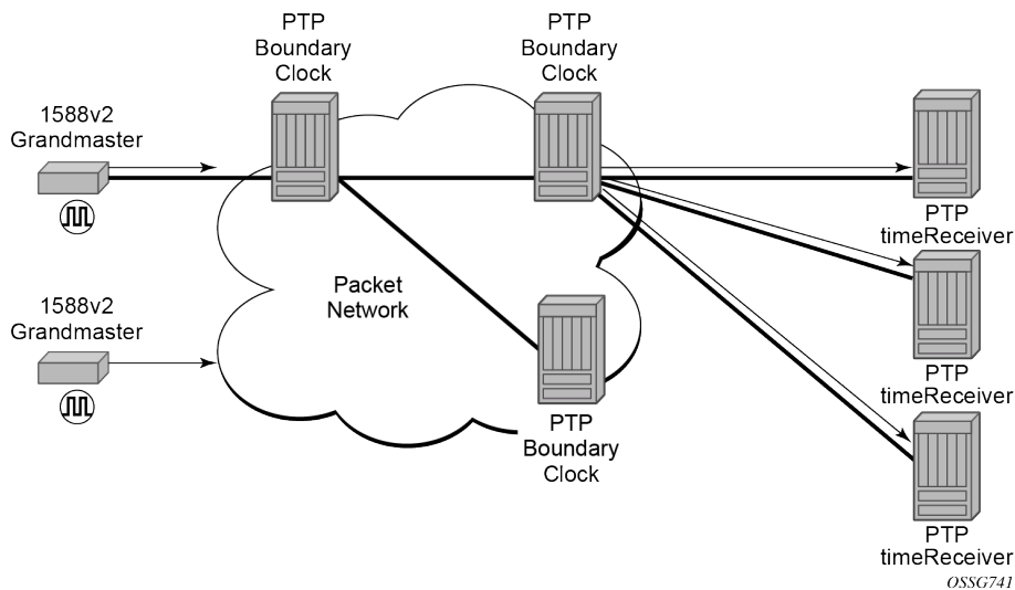
Figure 21: PTP boundary clock for frequency and time
