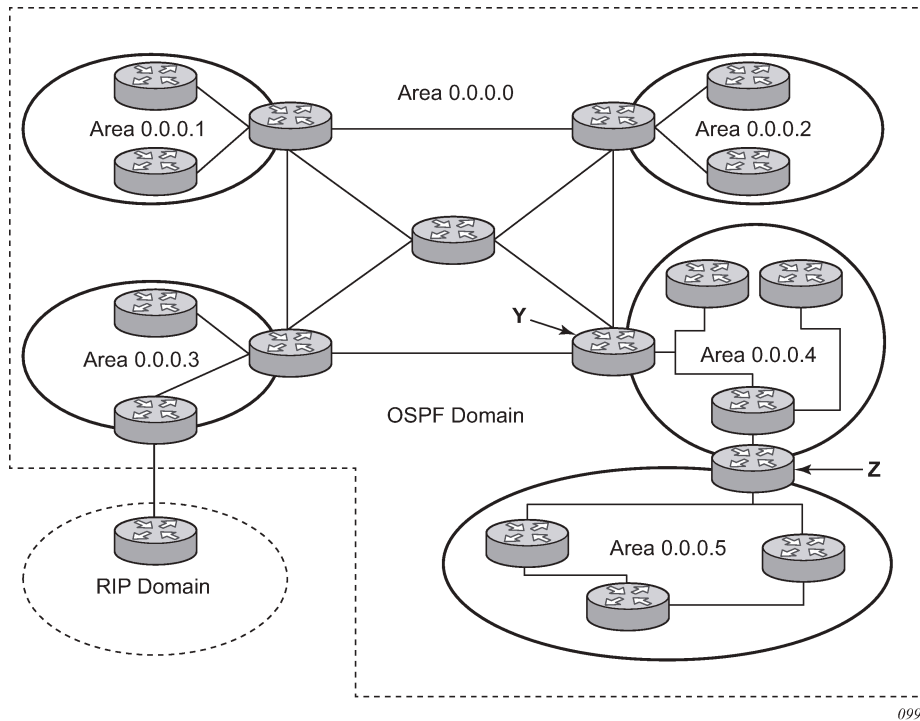
Figure 59: OSPF areas
