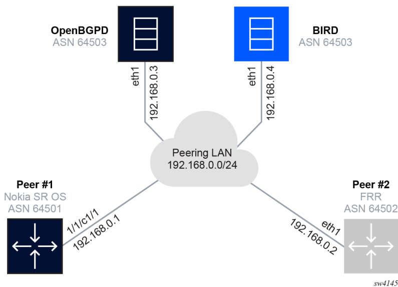
Figure 1: Peering topology
