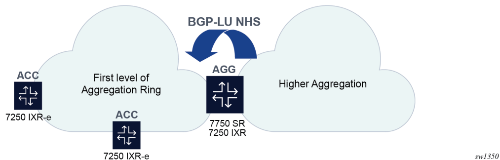
Figure 28: Next-hop-self for BGP-LU routes
