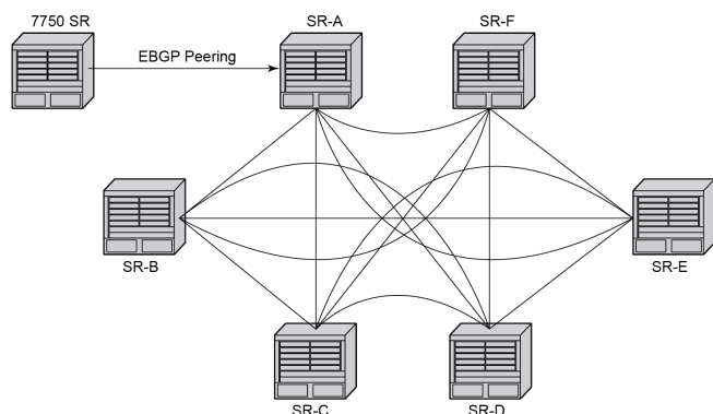
Figure 20: Fully meshed BGP configuration
