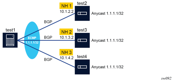
Figure 23: Sticky ECMP flow distribution as next hops are removed part 2
