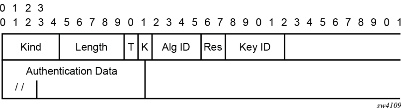
Figure 10: Packet format
