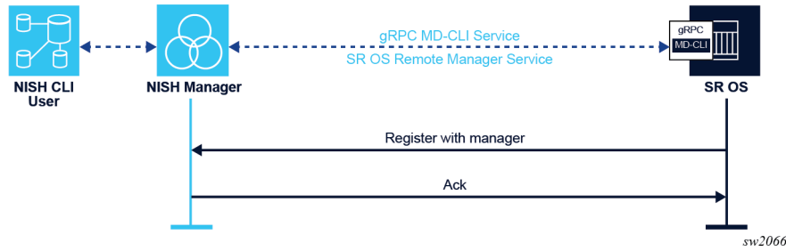
Figure 6: SR OS remote management communication with the NISH manager
