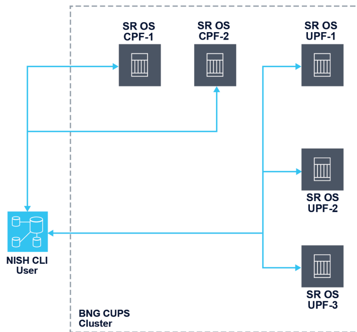
Figure 1: NISH management of BNG CUPS cluster
