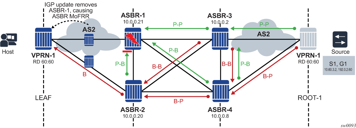
Figure 74: Failure scenario 2
