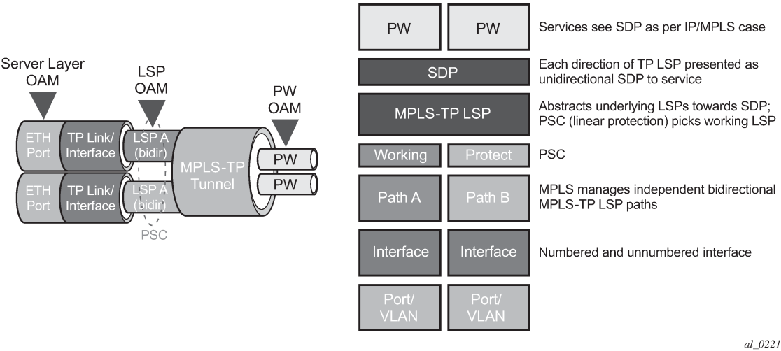
Figure 7: MPLS-TP model
