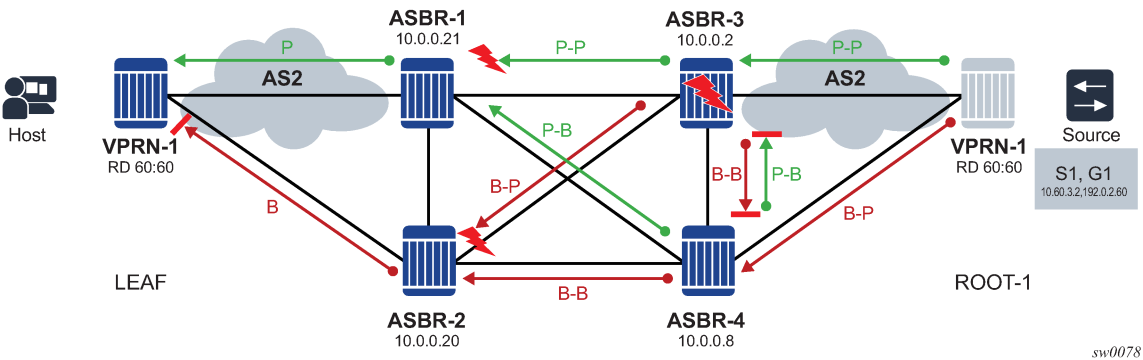
Figure 76: ASBR-3 failure
