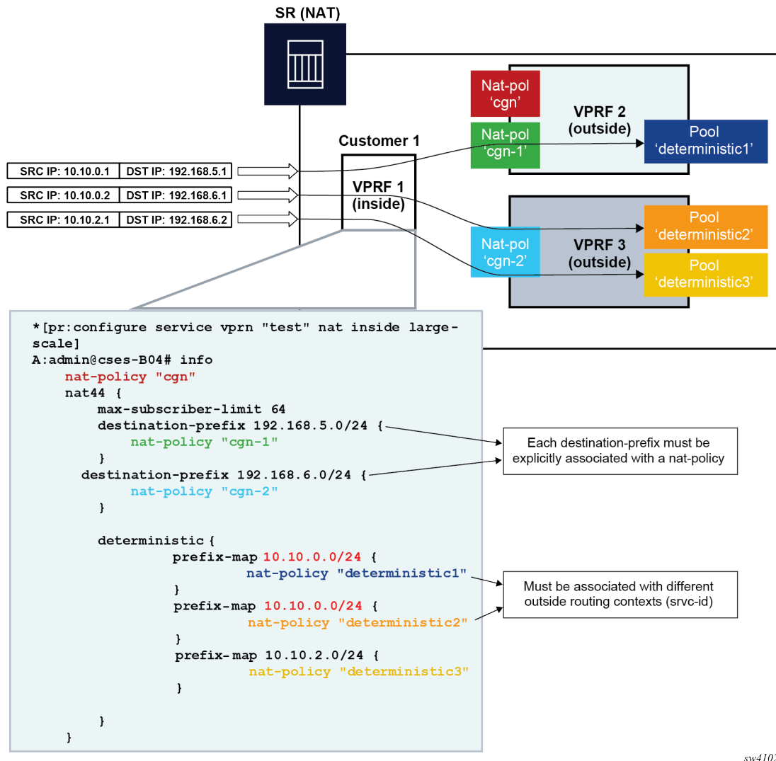
Figure 84: MNP and deterministic NAT44 (MD-CLI)
