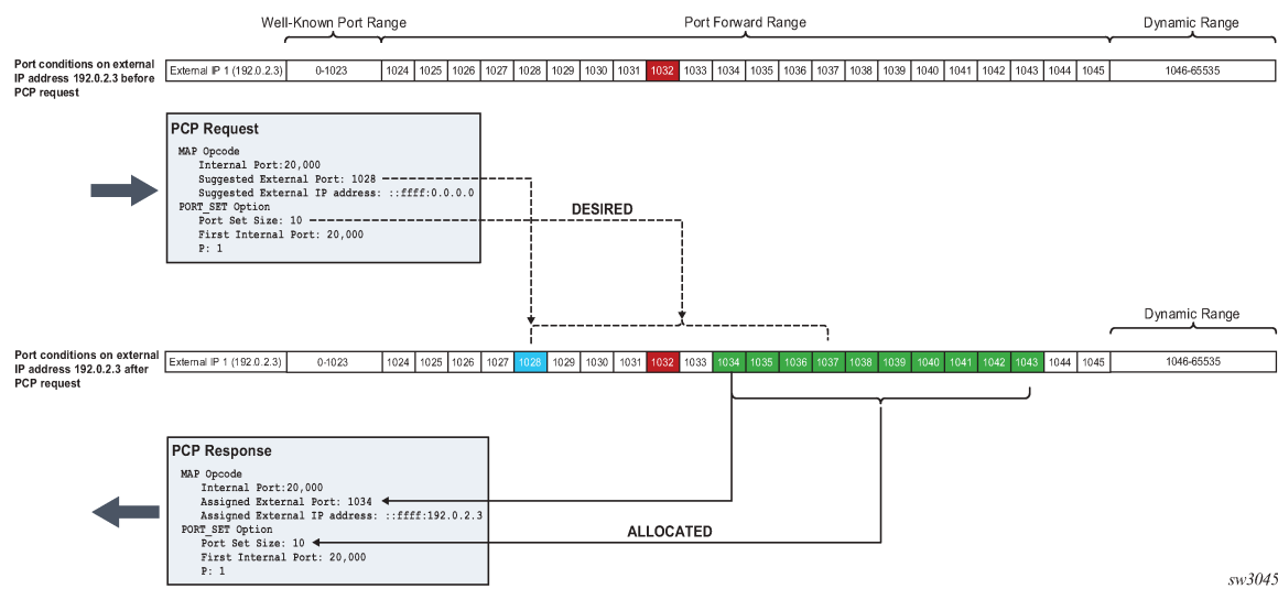
Figure 89: PORT_SET example
