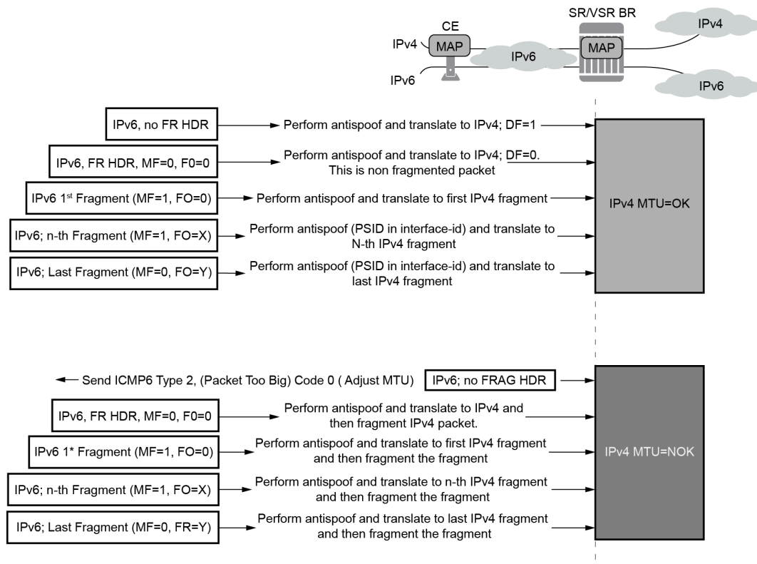
Figure 120: Fragmentation in the upstream direction
