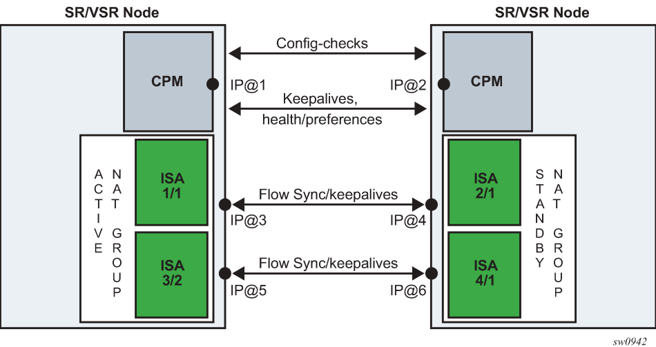
Figure 110: NAT synchronization
