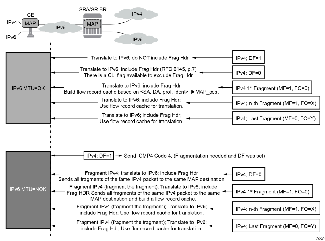
Figure 119: Fragmentation in the downstream direction
