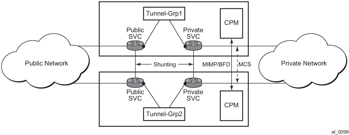
Figure 44: MC-IPsec architecture
