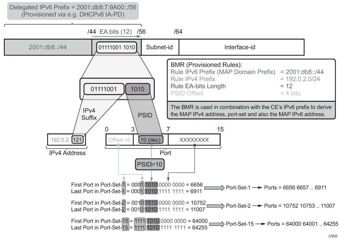
Figure 113: A+P mapping
