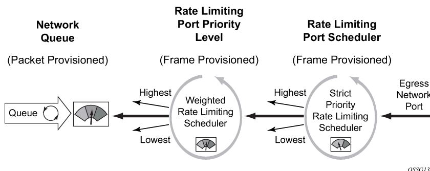
Figure 12: Bandwidth distribution on network port with port-based scheduling
