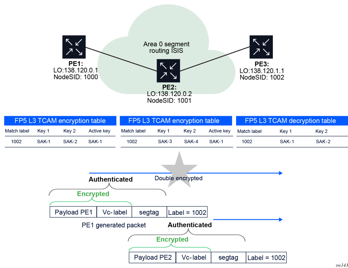
Figure 87: ANYsec double-encryption scenario
