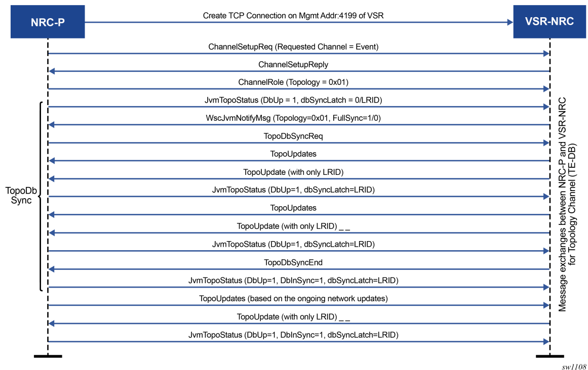
Figure 69: TE-DB partial synchronization message sequence
