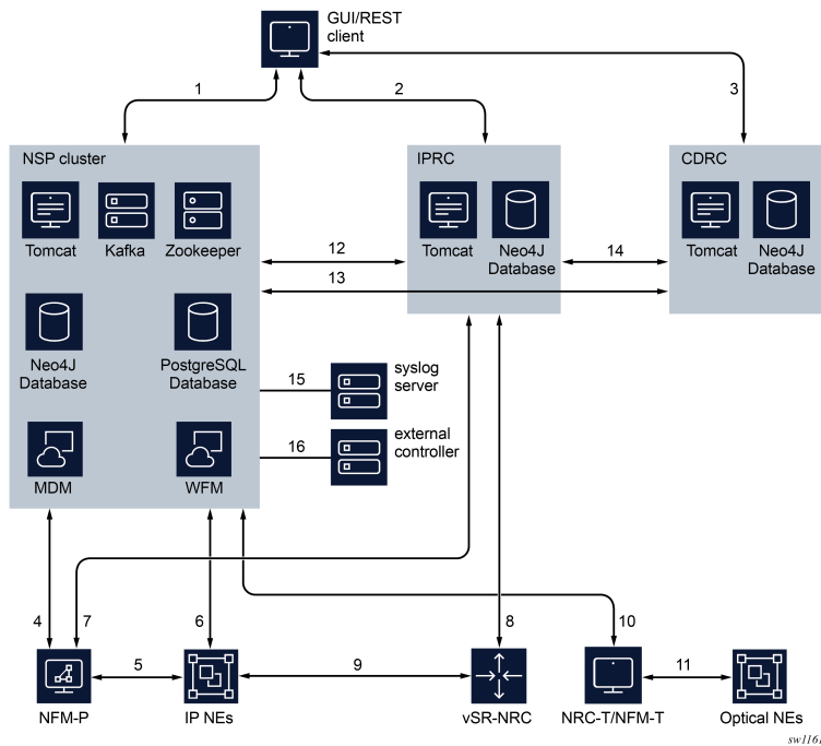
Figure 63: NSP architecture
