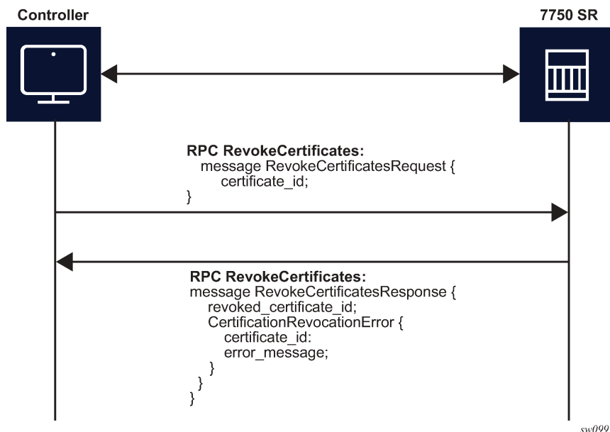
Figure 41: RPC RevokeCertificates message flow
