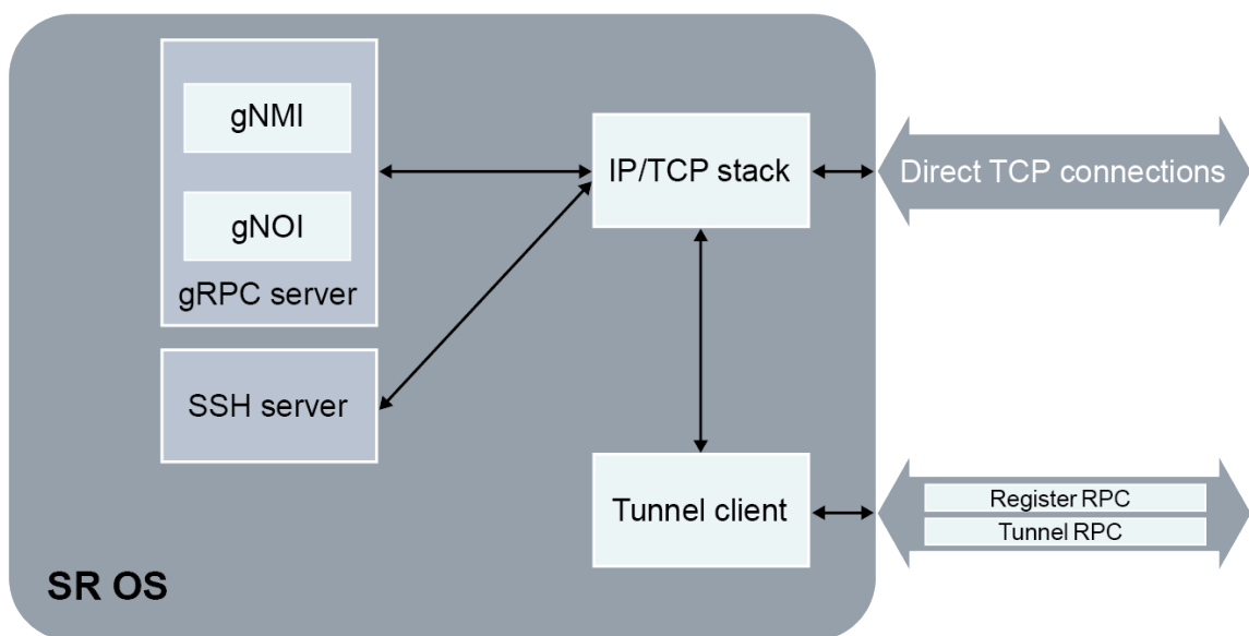
Figure 44: Internal SR OS architecture
