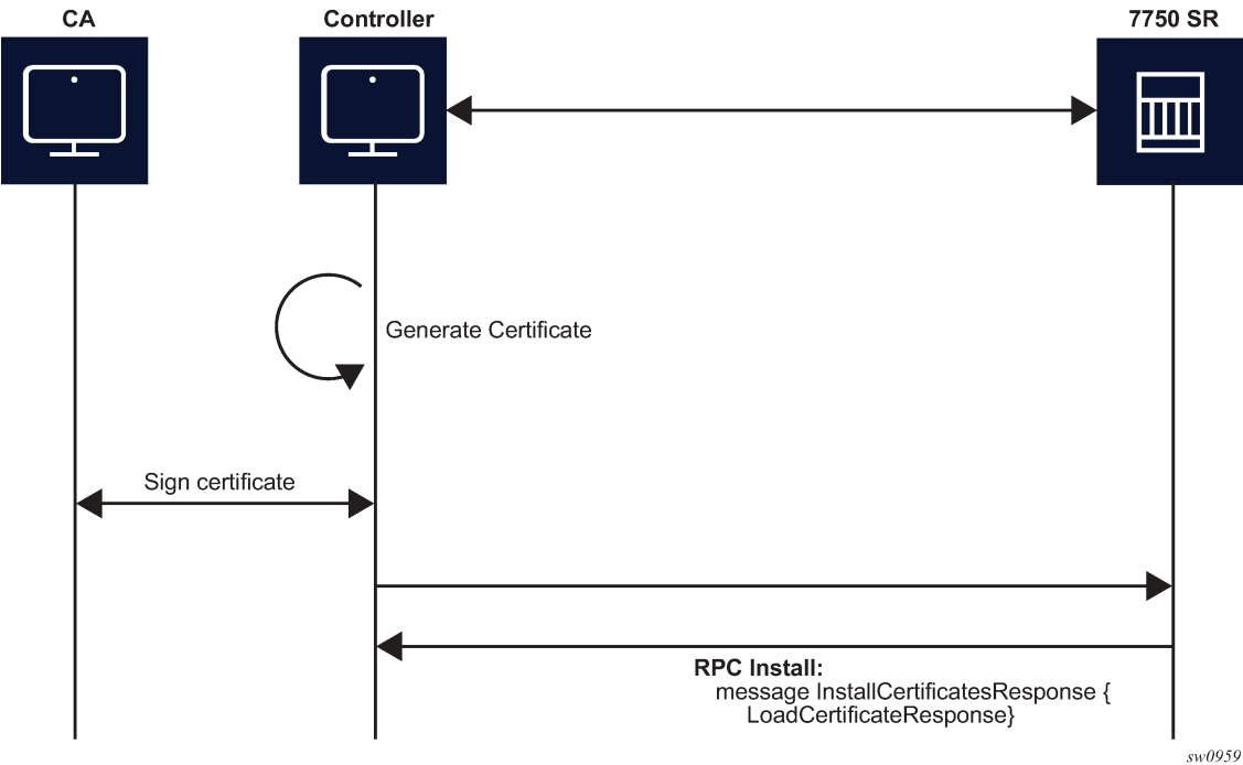
Figure 40: RPC install message flow if CSRs are not generated on the SR OS node
