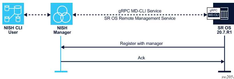
Figure 42: Remote management service initiation
