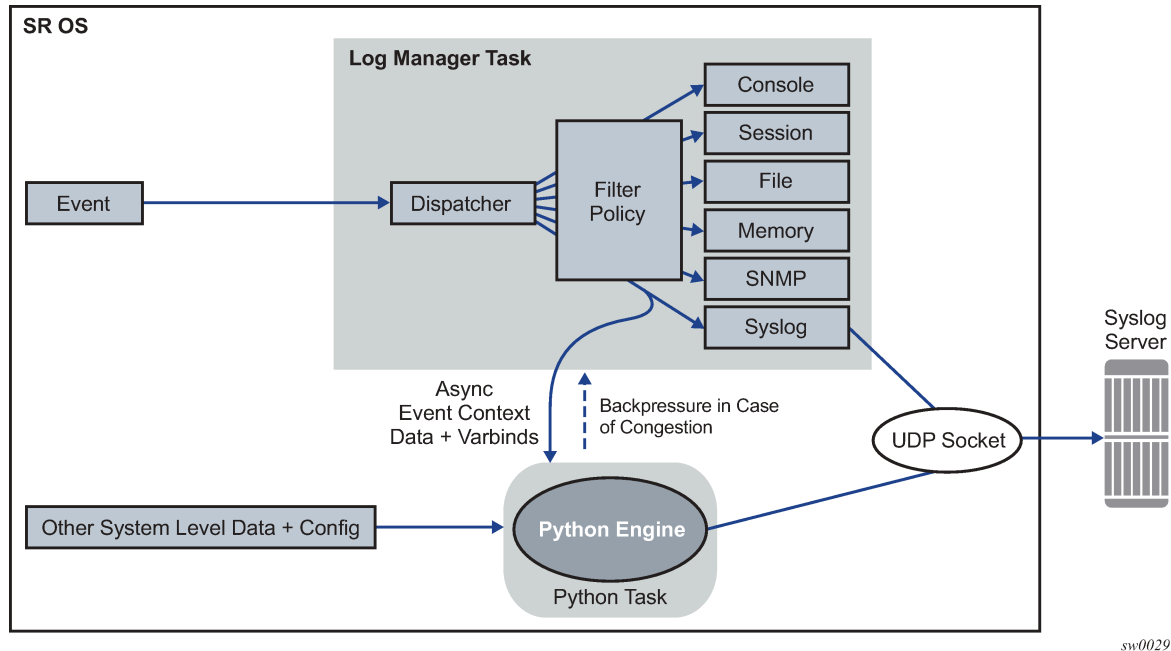
Figure 26: Interaction between the logger and the Python engine
