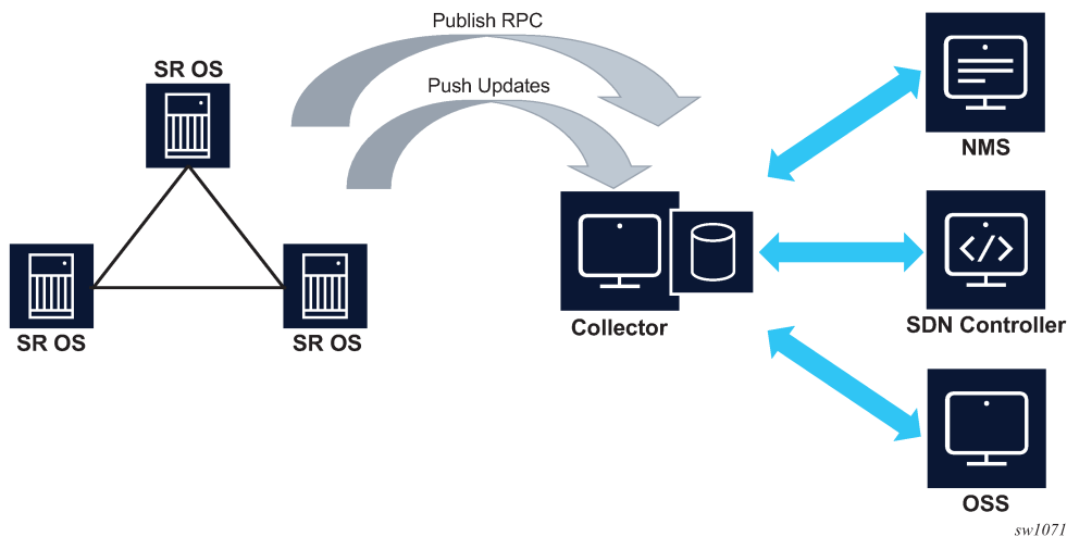
Figure 31: Dial-out telemetry session
