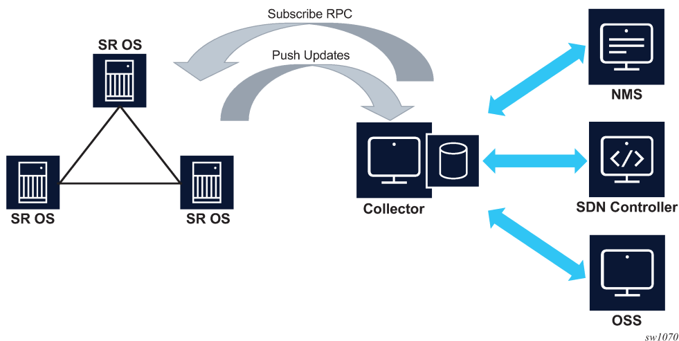
Figure 30: Dial-in telemetry session
