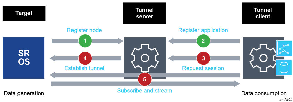
Figure 43: gRPC tunnel service concept
