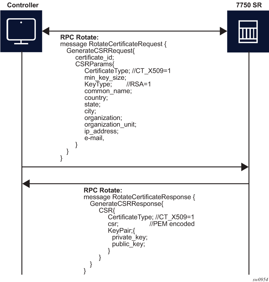
Figure 37: GenerateCSR message flow
