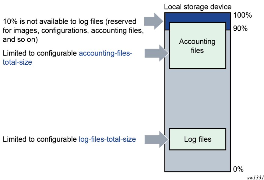
Figure 22: Accounting and log file storage limits
