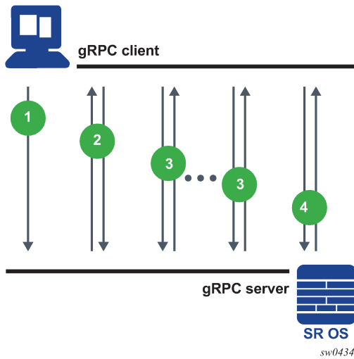
Figure 32: NE configuration and information retrieval using gNMI service
