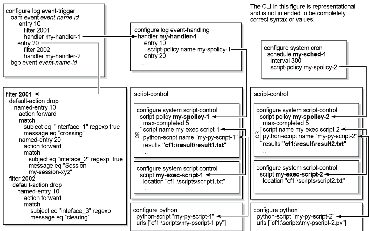
Figure 24: EHS object handling (MD-CLI)
