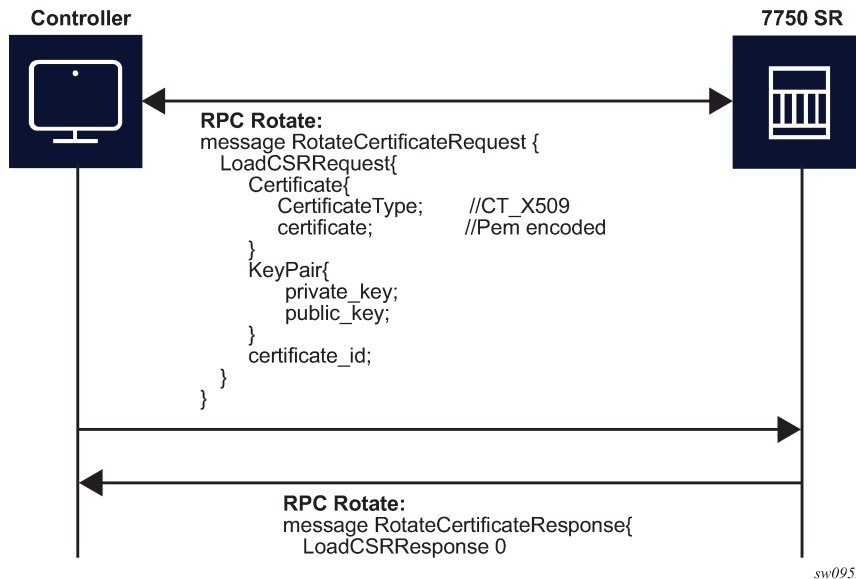
Figure 38: LoadCSRRequest/Response message flow
