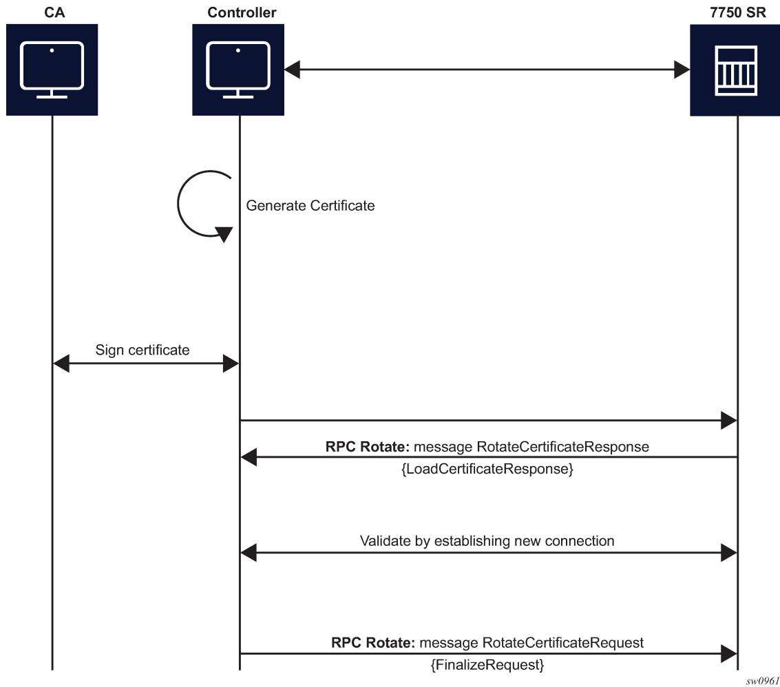
Figure 36: RPC Rotate message flow when CSRs are not generated on the SR OS node
