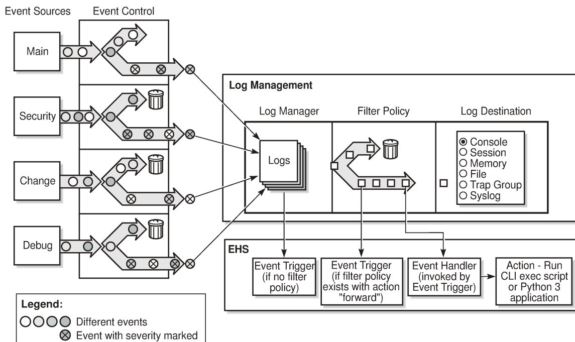
Figure 23: Event logging block diagram
