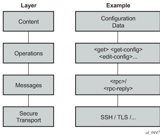
Figure 20: NETCONF layers (RFC 6241)
