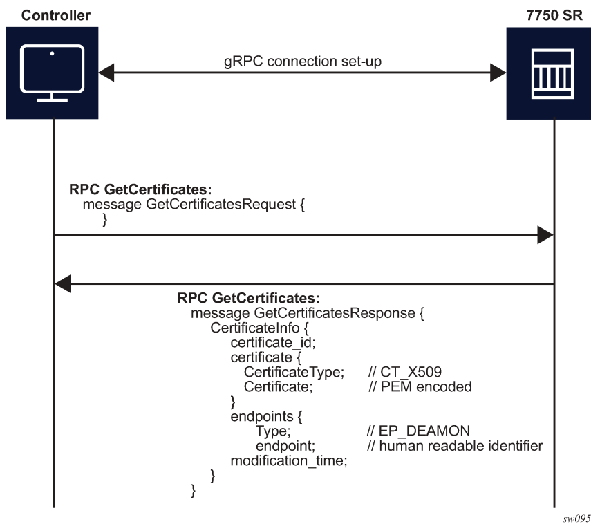
Figure 33: RPC GetCertificates message flow
