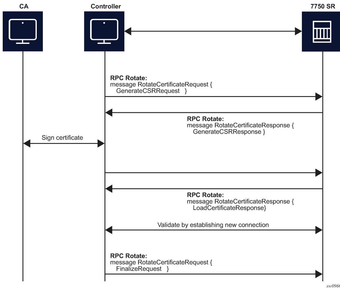
Figure 35: RPC Rotate message flow for CSRs generated on the SR OS node
