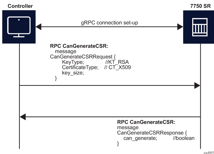
Figure 34: RPC CanGenerateCSR message flow
