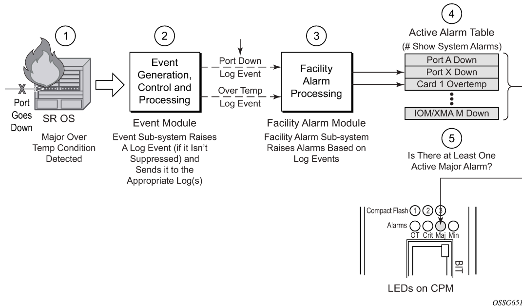
Figure 47: Log events, facility alarms and LEDs
