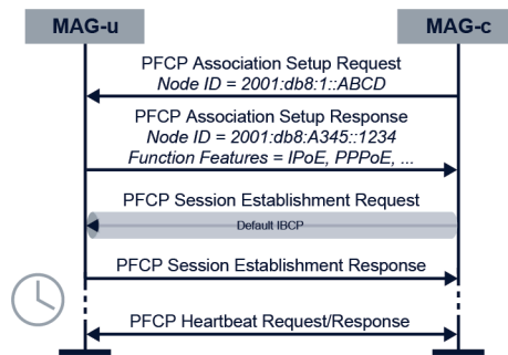
Figure 1: MAG-u PFCP association setup flow
