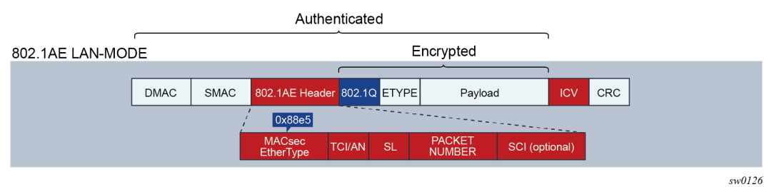
Figure 5: 802.1 AE LAN-MODE
