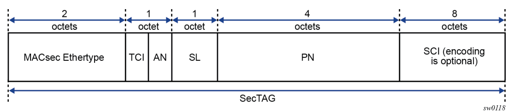
Figure 6: SecTAG format
