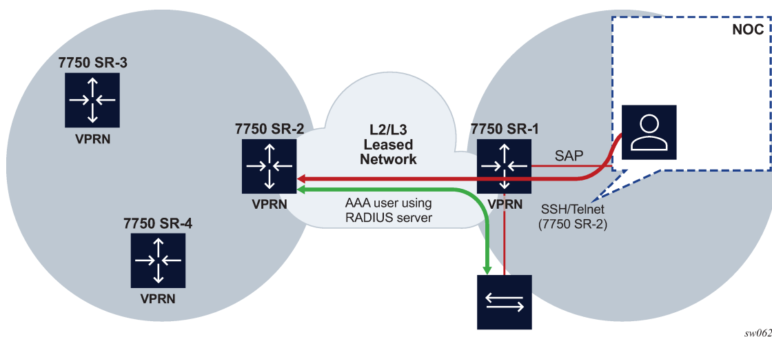
Figure 26: VPRN network example
