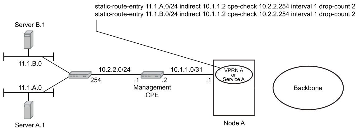
Figure 16: Multiple hops to IP target (classic CLI)
