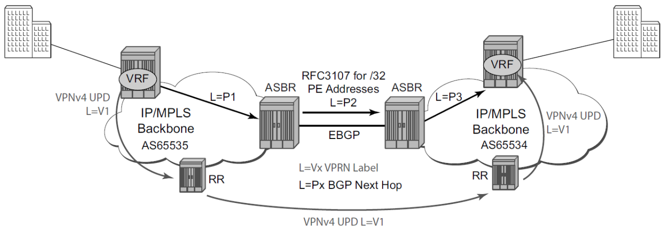
Figure 24: Inter-AS option-C
