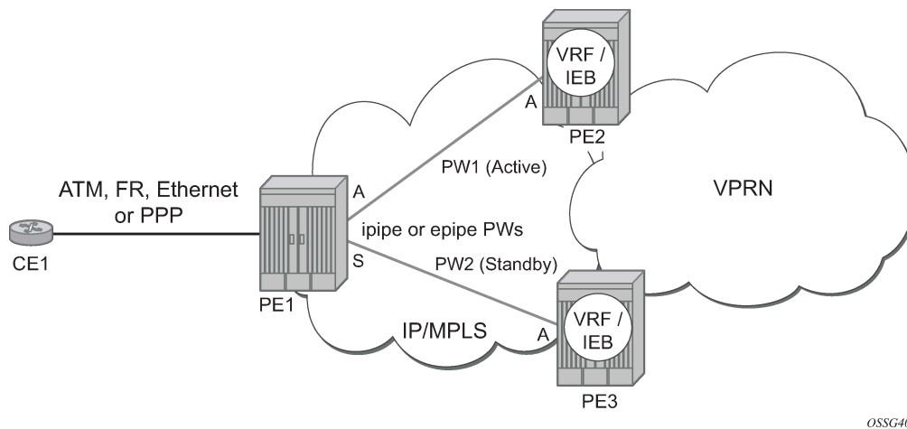
Figure 19: Active/standby VRF using resilient Layer 2 circuits
