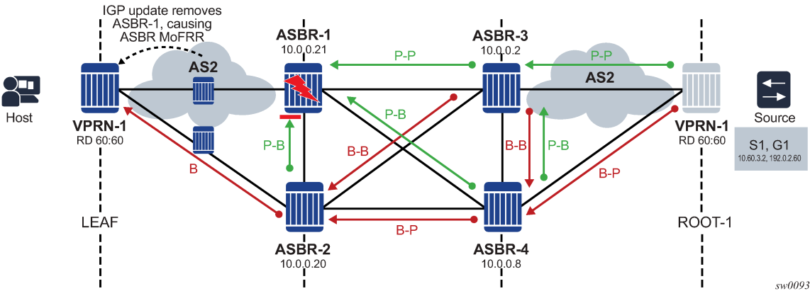
Figure 74: Failure scenario 2
