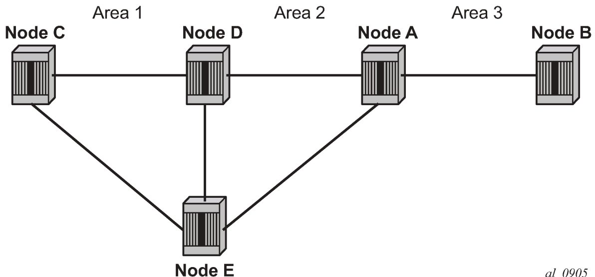
Figure 33: CSPF for an inter-area LSP
