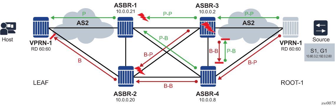
Figure 76: ASBR-3 failure
