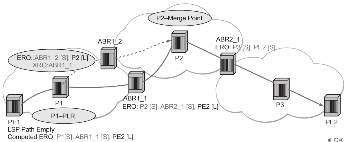
Figure 34: ABR node protection using dynamic bypass LSP
