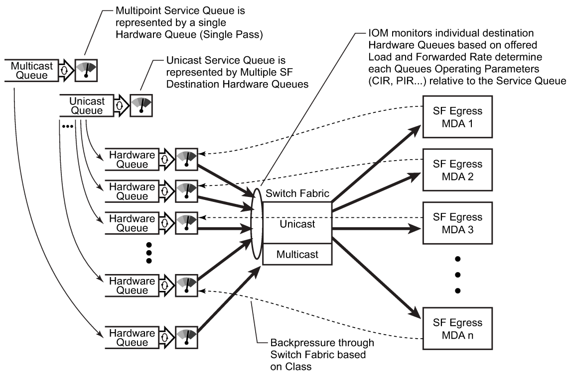
Figure 39: Unicast service queue mapping to multiple destination-based hardware queues
