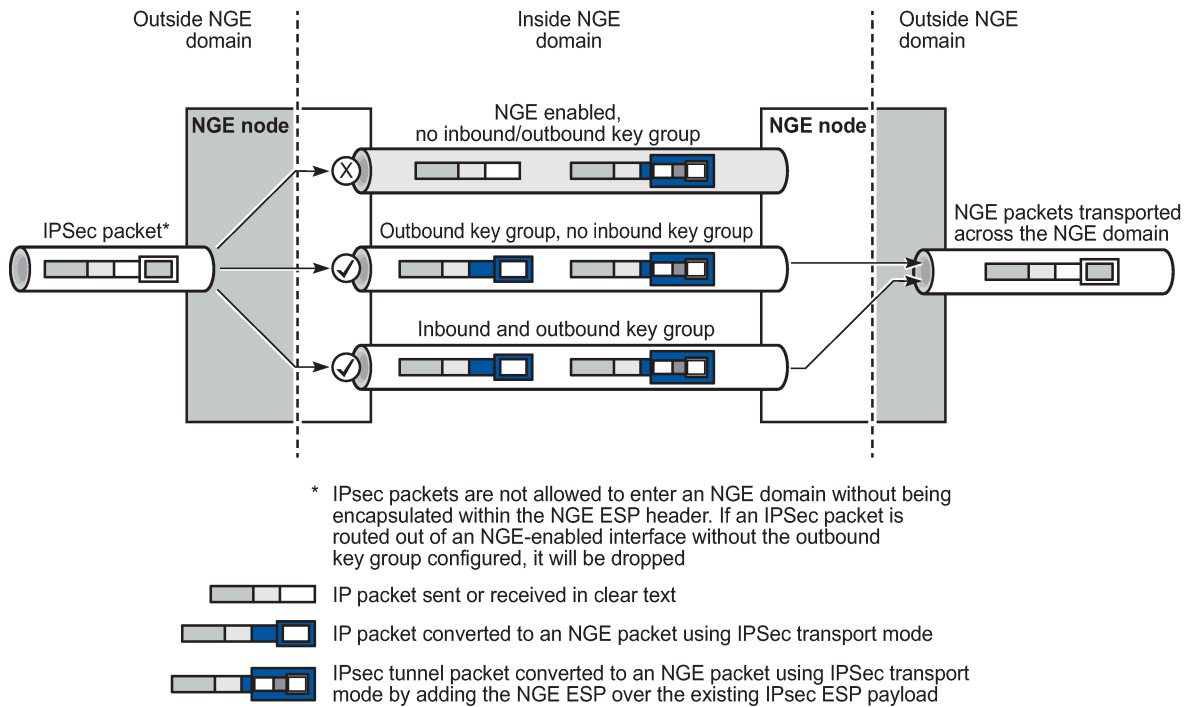
Figure 19: IPsec packets transiting an NGE domain
