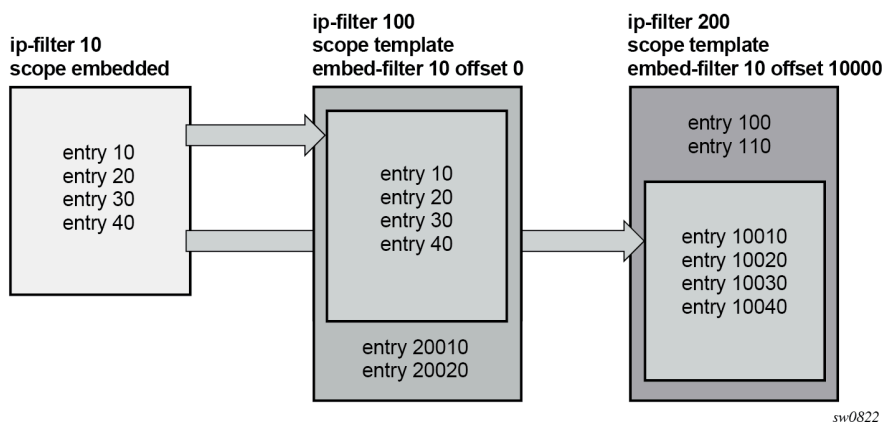
Figure 23: Embedded Filter Policy
