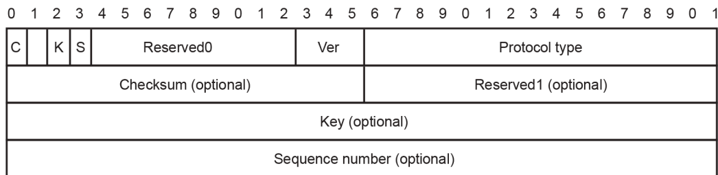
Figure 11: GRE header format
