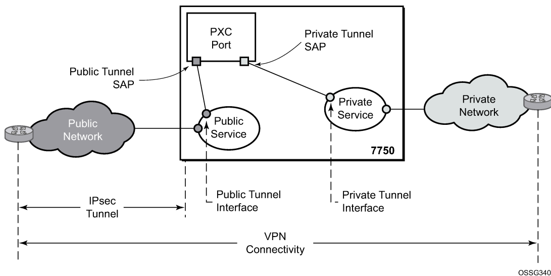
Figure 12: GRE deployment using a PXC port example
