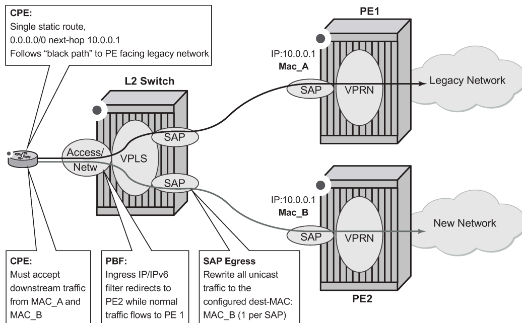
Figure 24: Layer 2 policy-based forwarding (PBF) redirect action
