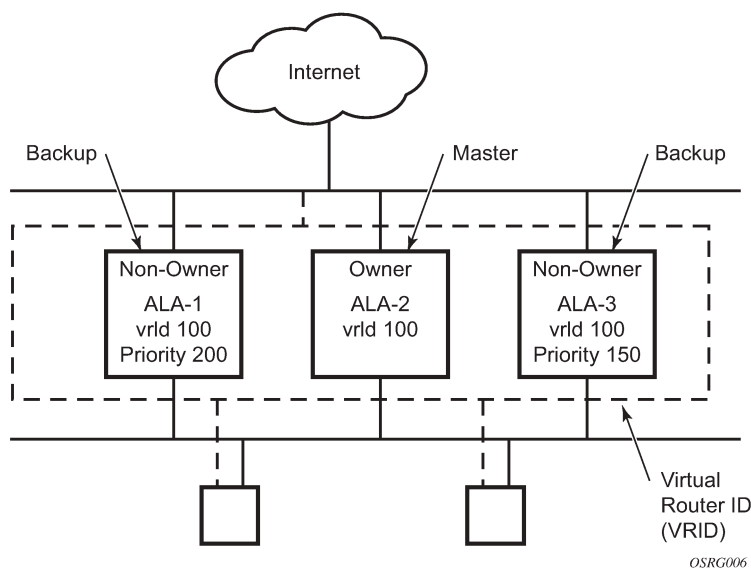
Figure 21: VRRP configuration
