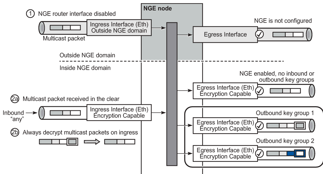
Figure 20: Processing multicast packets
