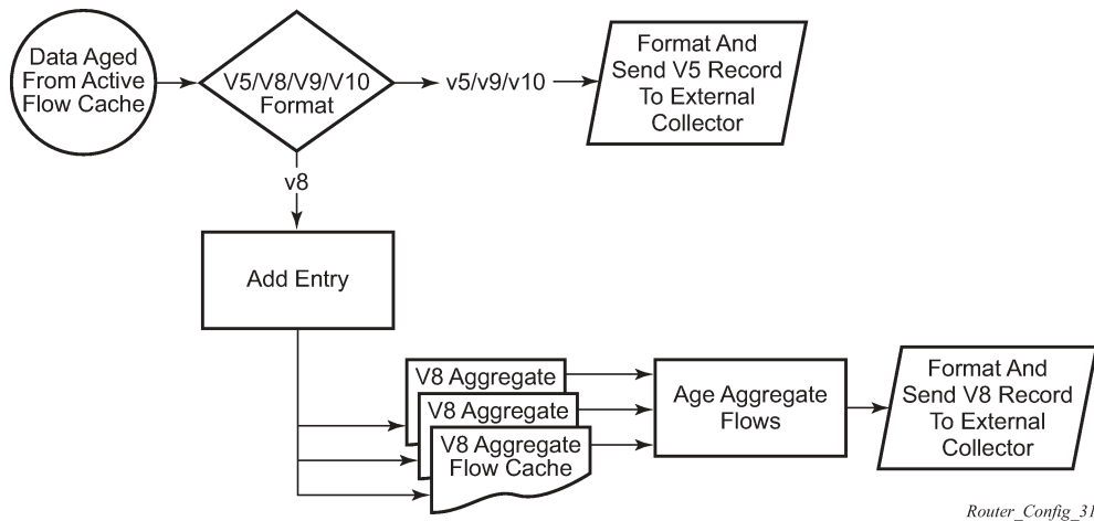
Figure 33: V5, V8, V9, V10, and flow processing
