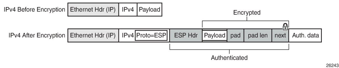
Figure 13: Router Interface Encryption Packet Format (IPsec Transport Mode)
