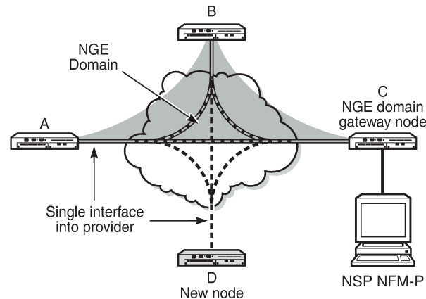
Figure 16: Private over intermediary network NGE domain
