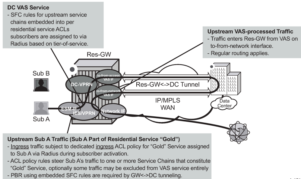
Figure 29: Upstream ESM ACL policy-based service chaining
