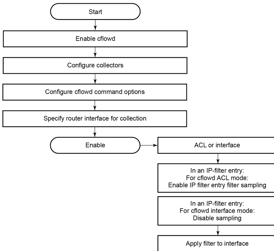
Figure 34: Cflowd configuration and implementation flow
