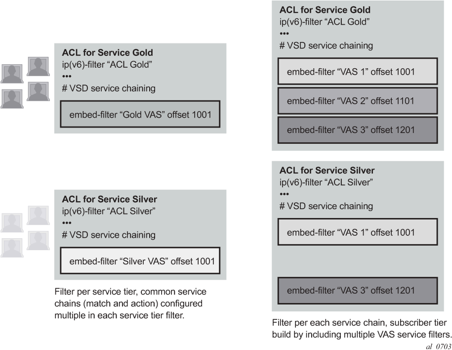
Figure 28: ACL filter modeling for ESM service chaining
