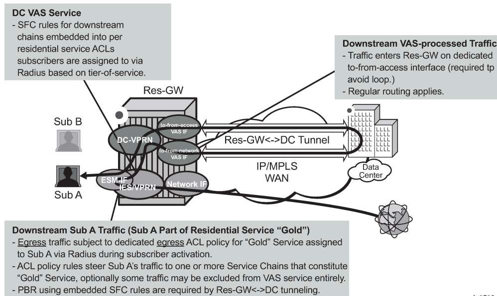
Figure 30: Downstream ESM ACL-policy based service chaining
