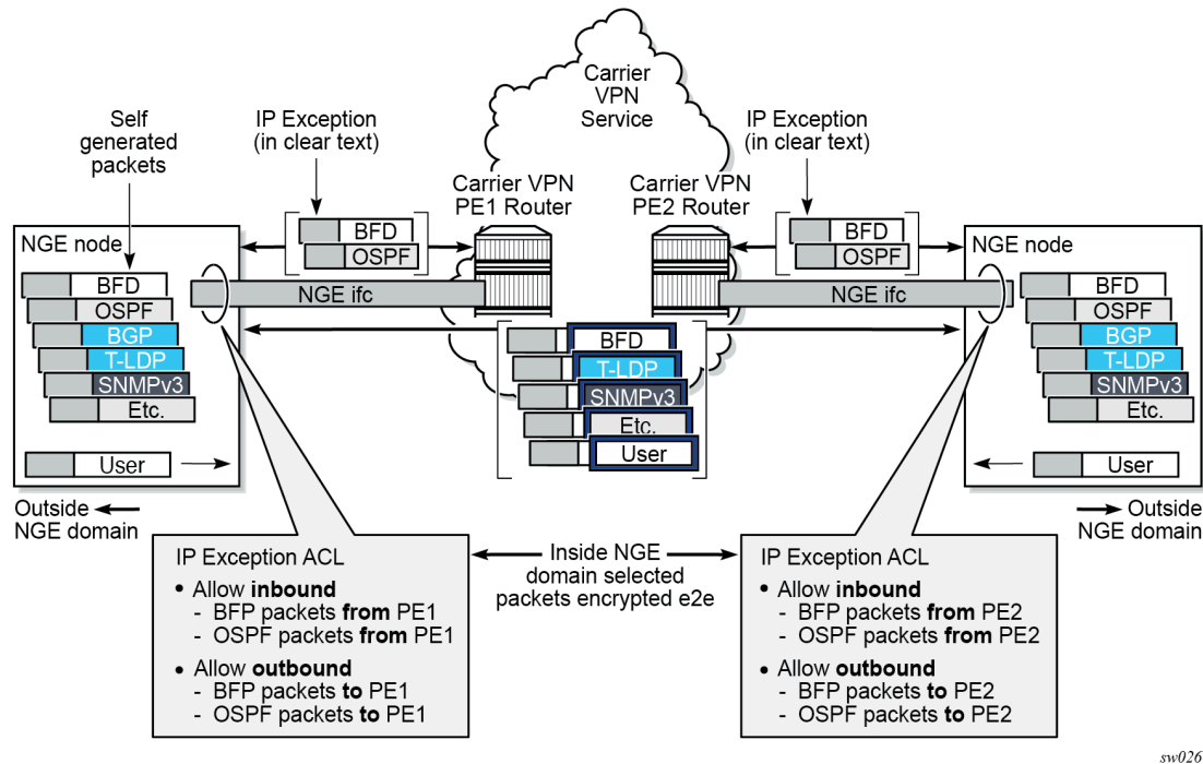
Figure 18: Router interface NGE exception filter example
