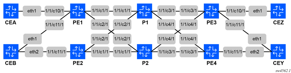
Figure 2: Topology used for configuration examples
