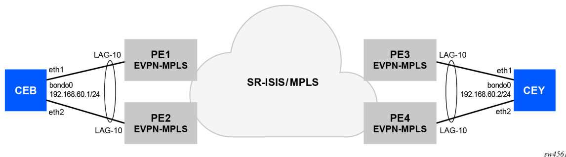
Figure 9: EVPN-MPLS topology used in this example
