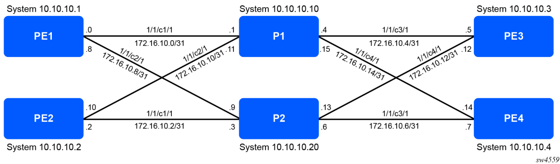
Figure 3: IPv4 addressing used for configuration examples
