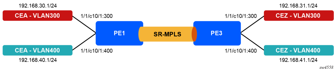
Figure 6: VPRN topology used in this example
