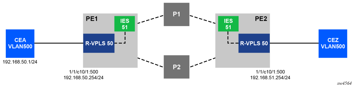
Figure 7: IES topology used in this example
