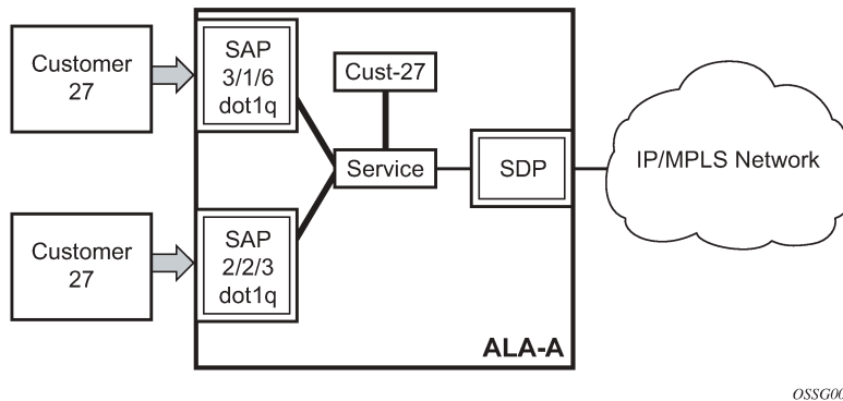
Figure 6: 7750 SR/7950 XRS service access point (SAP)
