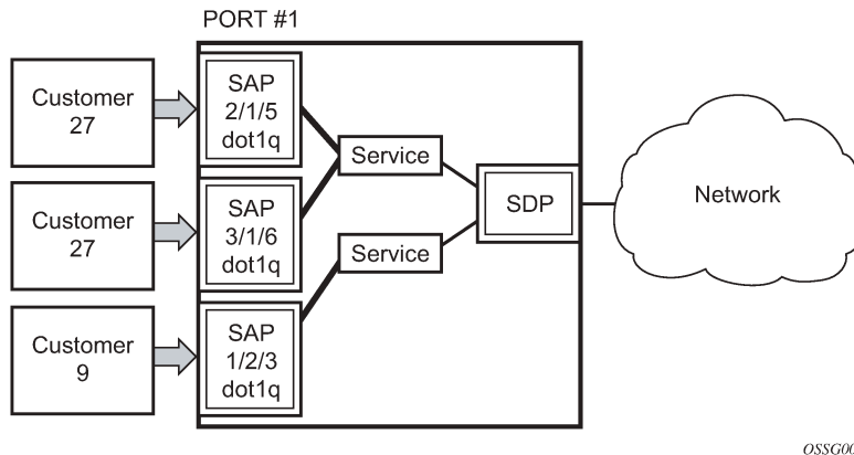
Figure 7: 7750 SR/7950 XRS and 7450 ESS multiple SAPs on a single port/channel
