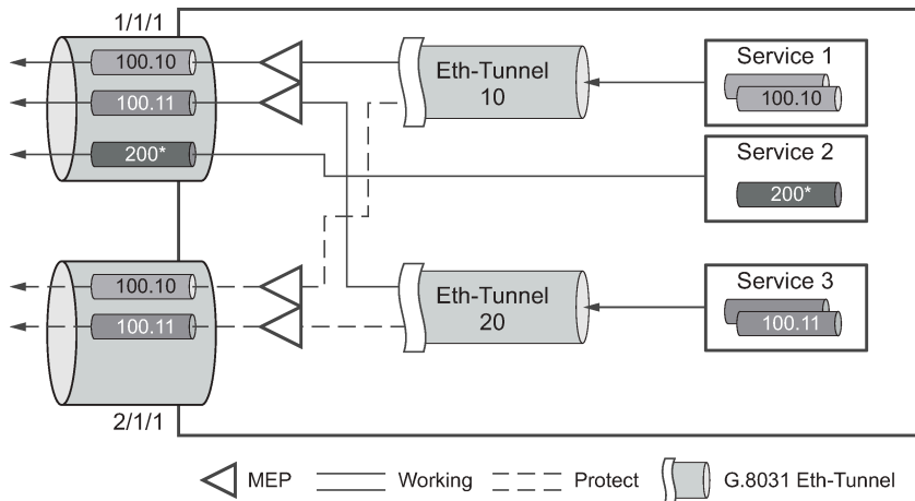
Figure 20: PBB fate-independent Ethernet tunnels
