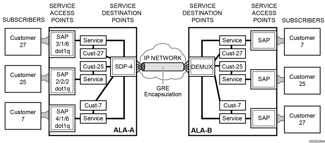
Figure 11: GRE SDP pointing from ALA-A to ALA-B
