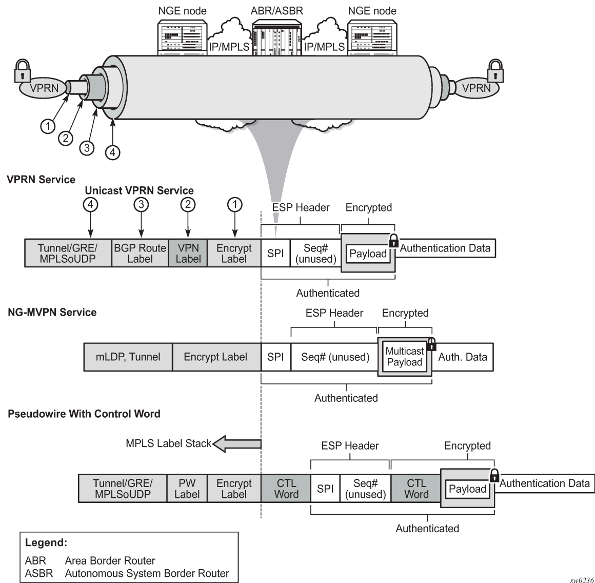
Figure 33: NGE and packet formats
