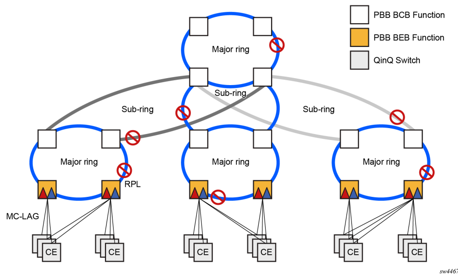
Figure 25: 0-4 G.8032 sub-ring
