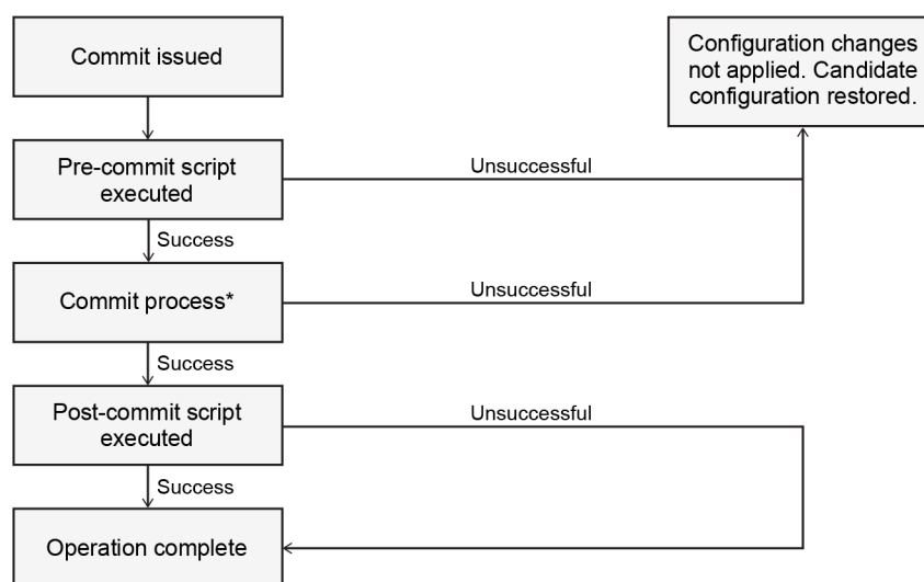
Figure 22: Commit operation
