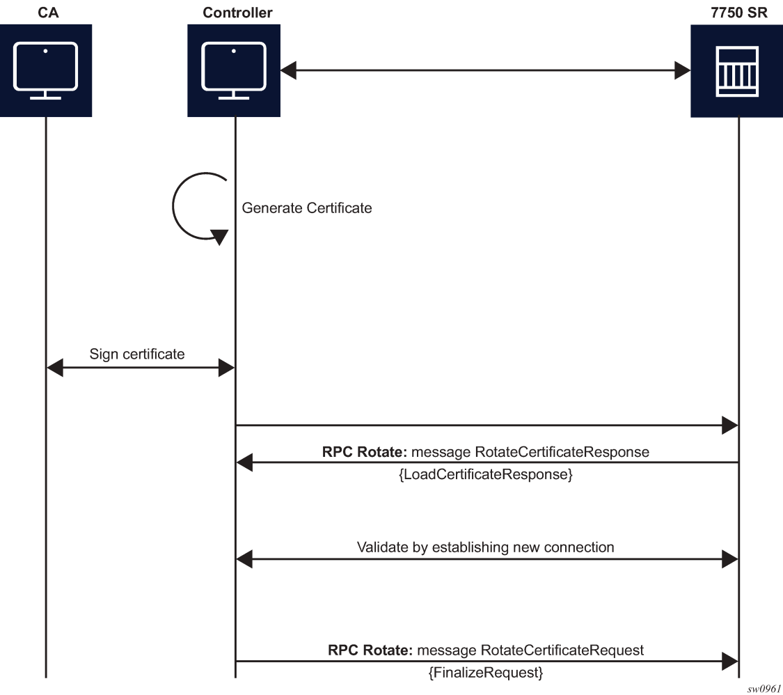
Figure 37: RPC Rotate message flow when CSRs are not generated on the SR OS node
