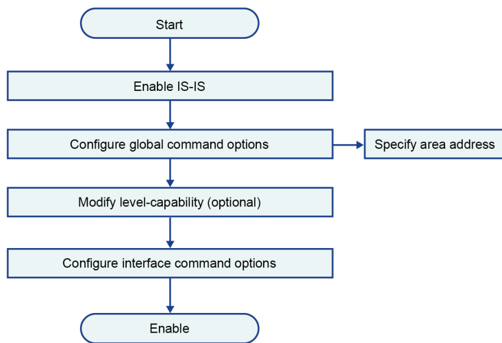
Figure 16: IS-IS configuration and implementation flow
