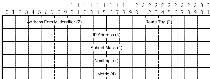
Figure 3: RIPv2 packet format
