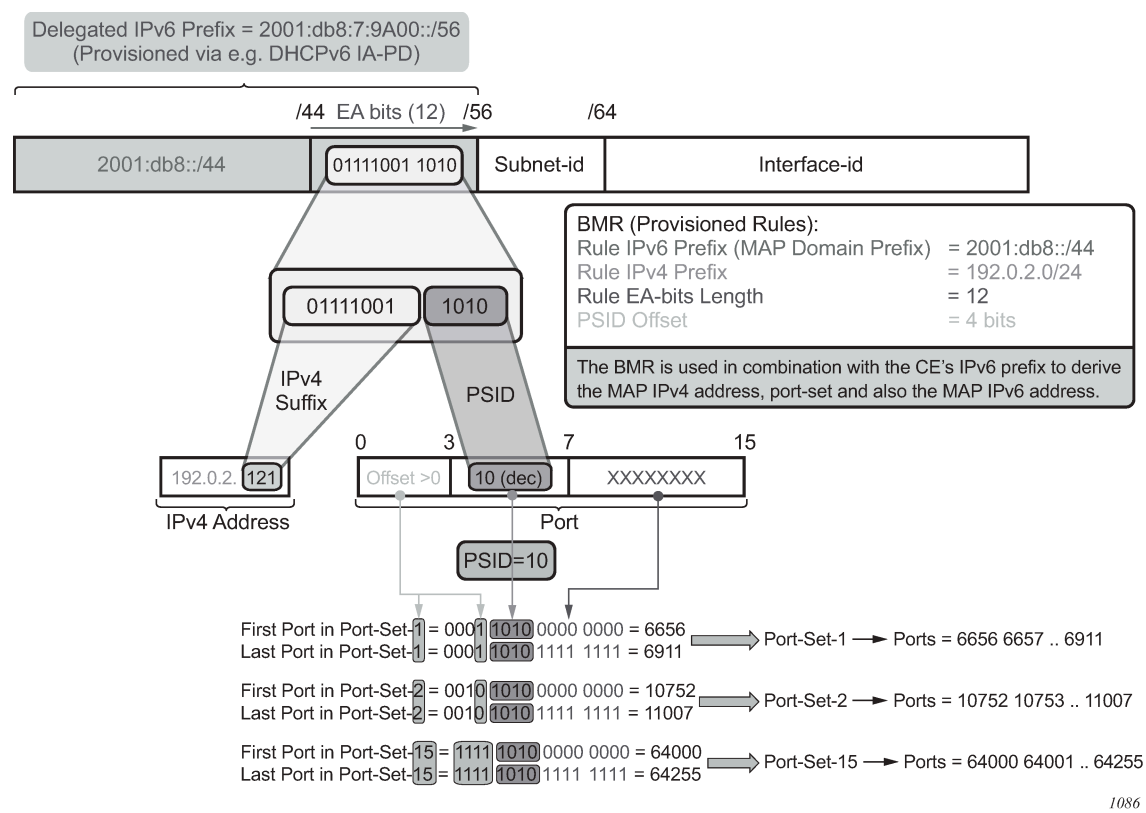
Figure 116: A+P mapping
