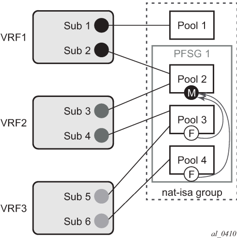
Figure 104: Consistency check
