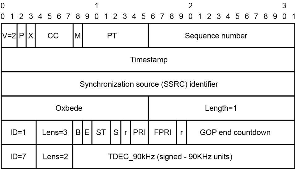
Figure 53: RTP header
