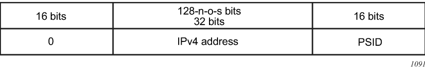
Figure 119: Node interface
