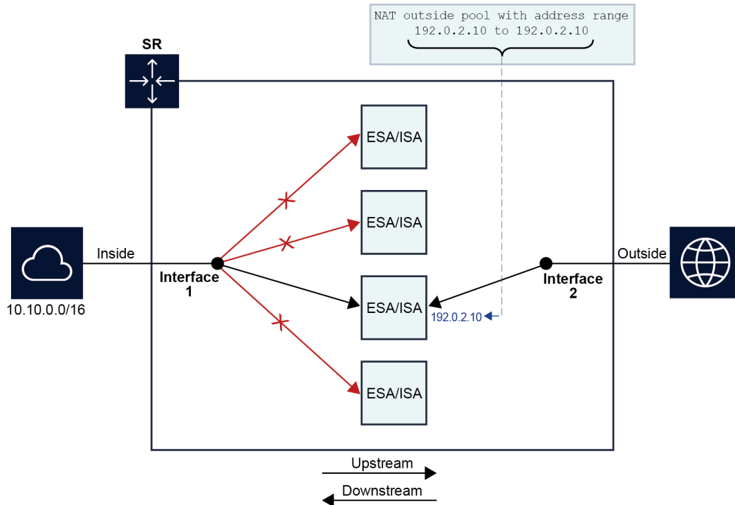
Figure 61: Traffic blackholing
