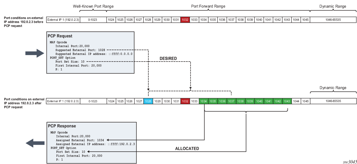
Figure 89: PORT_SET example
