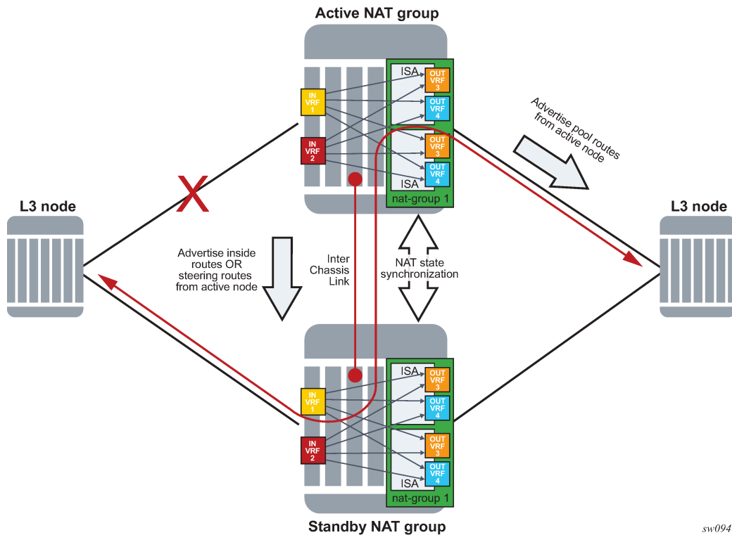
Figure 109: Asymmetric traffic
