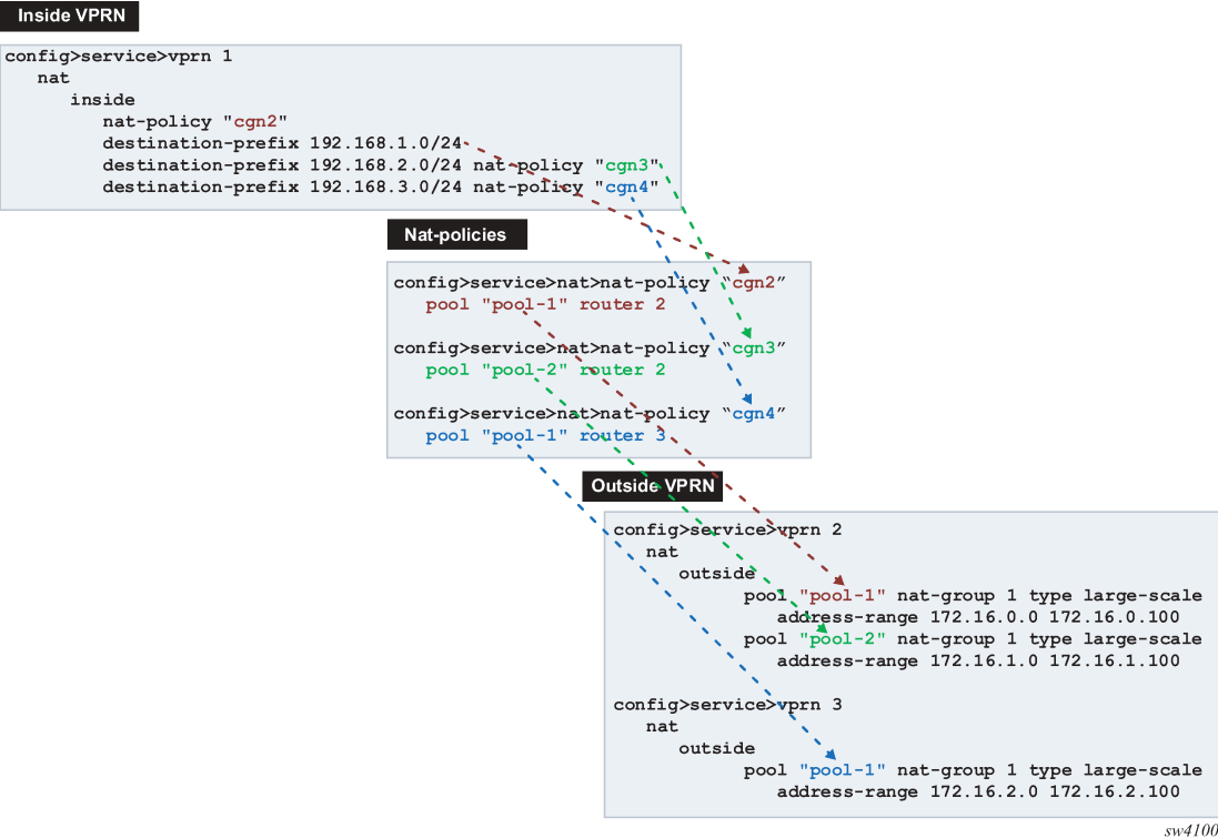
Figure 72: Logical representation of NAT routing through SR displays the logical configuration.
