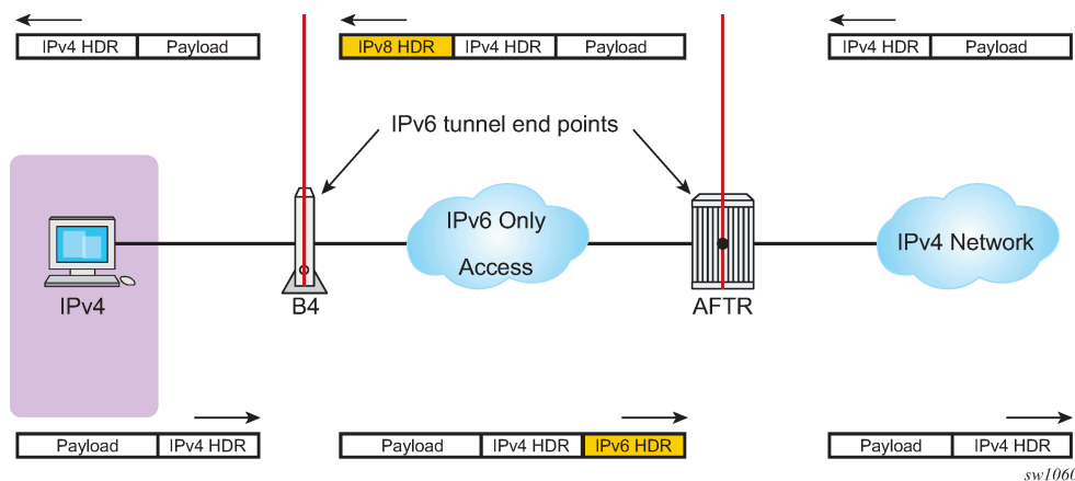
Figure 100: DS-Lite
