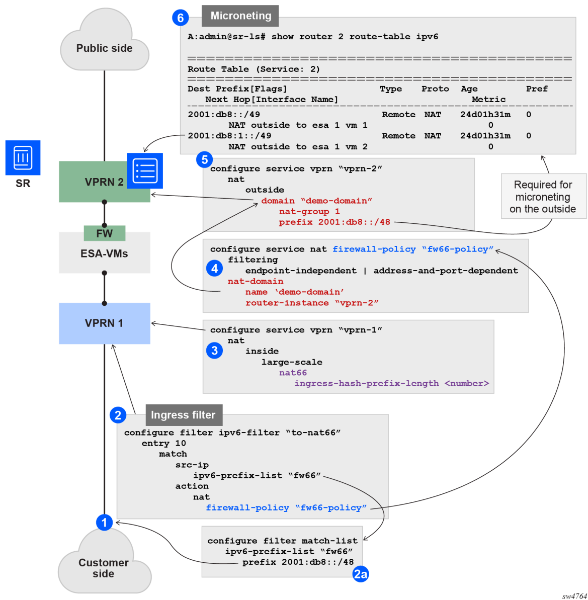
Figure 124: Pass-through NAT
