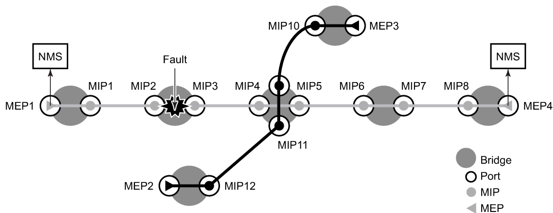
Figure 47: CFM CC failure scenario
