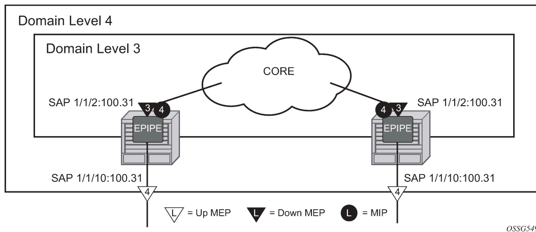
Figure 41: MIP creation example (NODE1)
