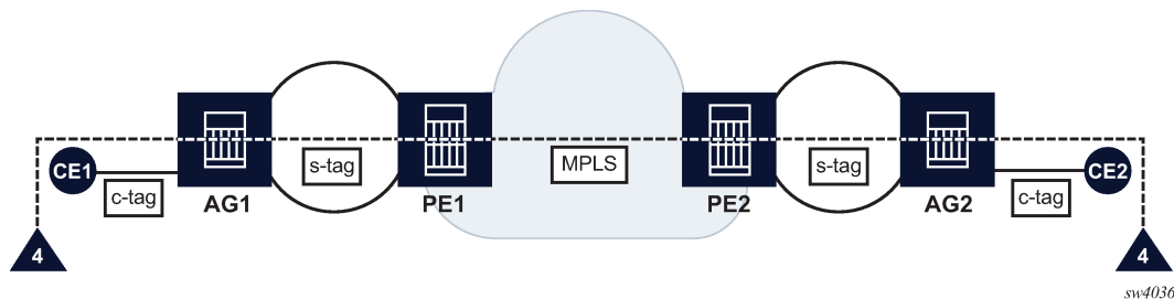
Figure 50: ETH-CFM CPE to CPE
