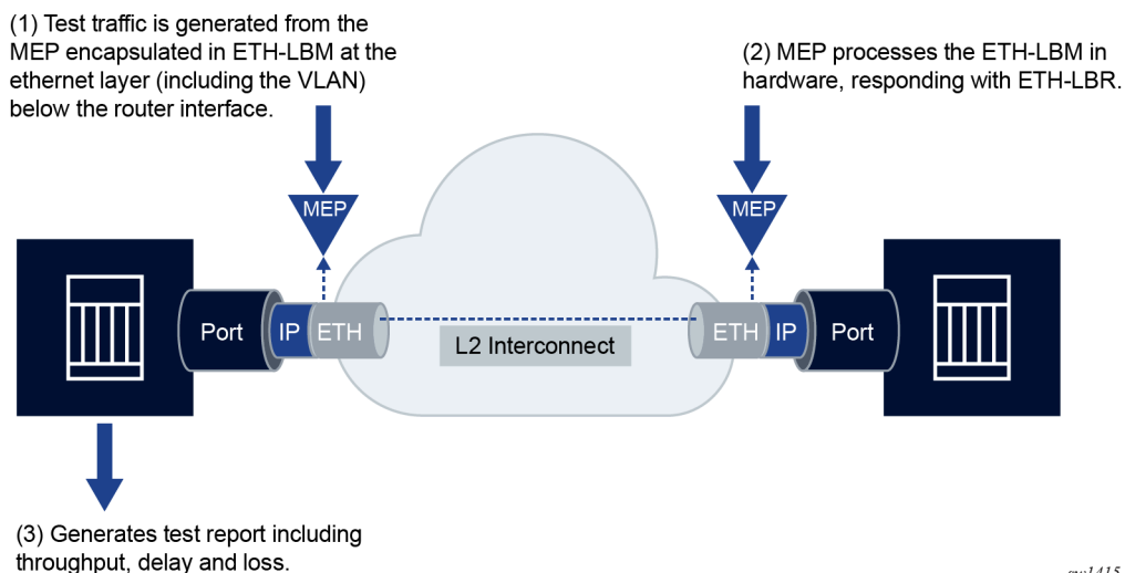
Figure 57: SAT generation and reflection on routed interfaces
