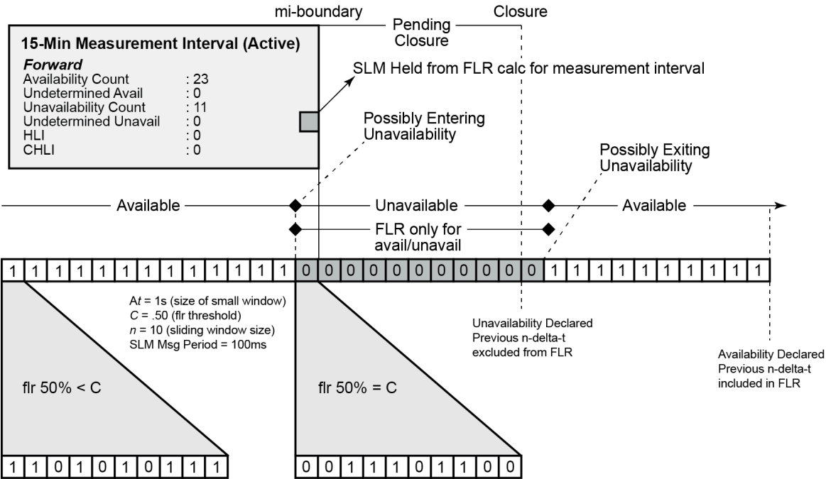
Figure 63: Evaluating and computing loss and availability
