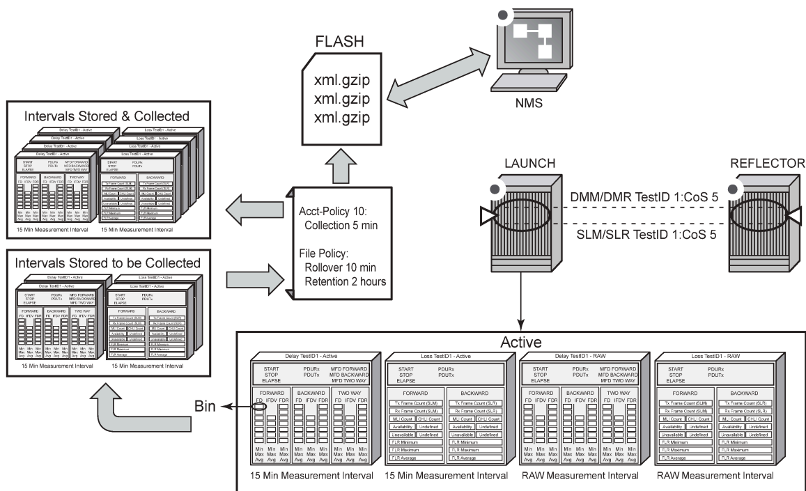
Figure 64: Relating OAM-PM components
