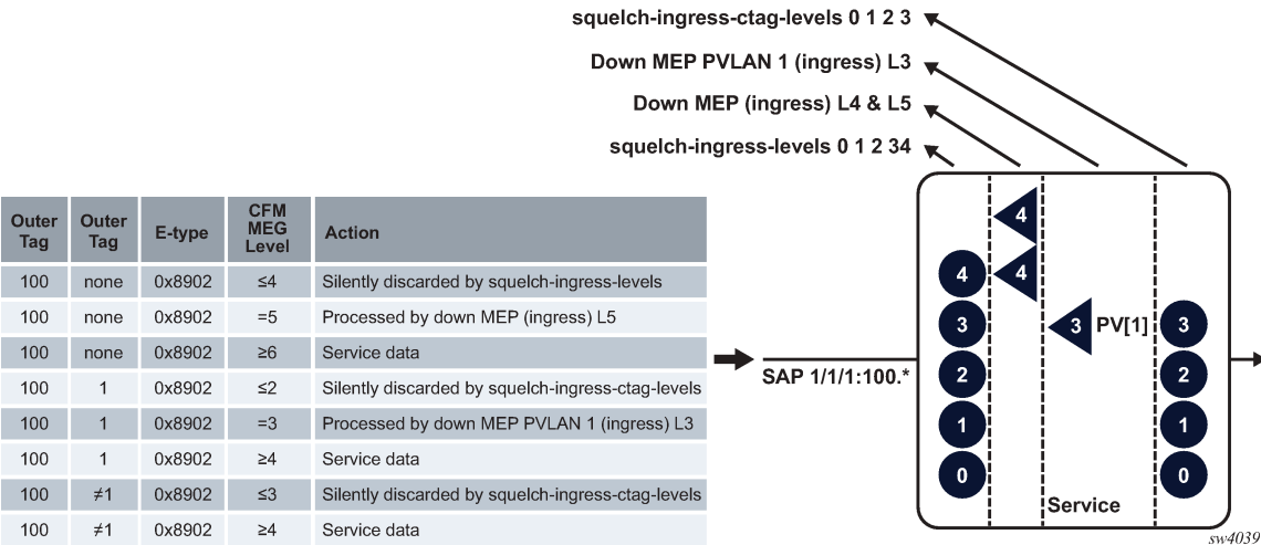
Figure 53: Logical processing chain and interaction
