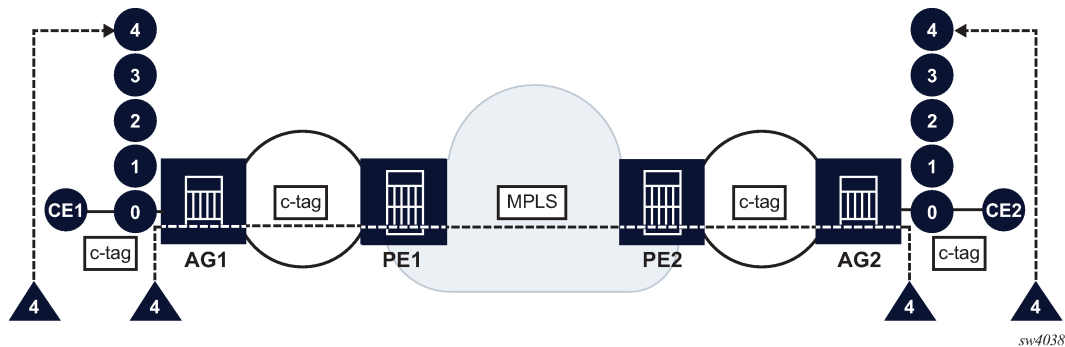
Figure 52: Enforcement of the CFM level agreement using squelching
