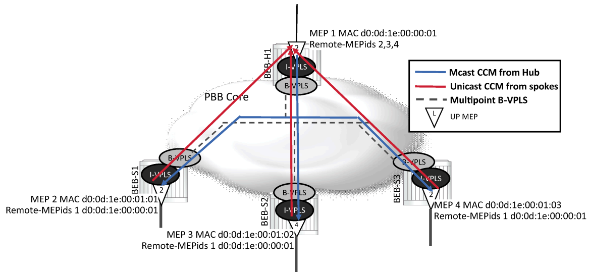
Figure 48: Unicast CCM in hub and spoke environments
