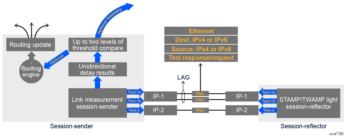
Figure 61: Link measurement with LAG micro sessions
