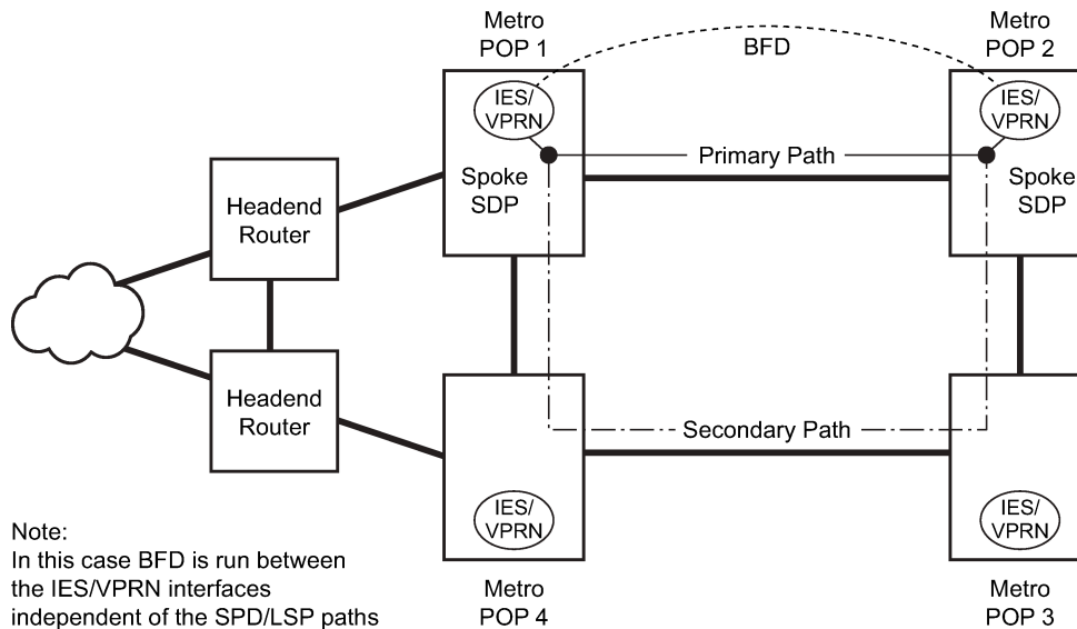
Figure 55: BFD for IES/VP RN over spoke SDP
