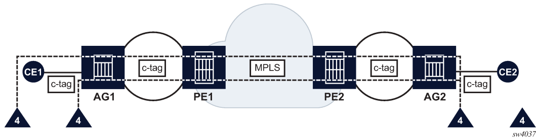
Figure 51: ETH-CFM collision between OAM domains
