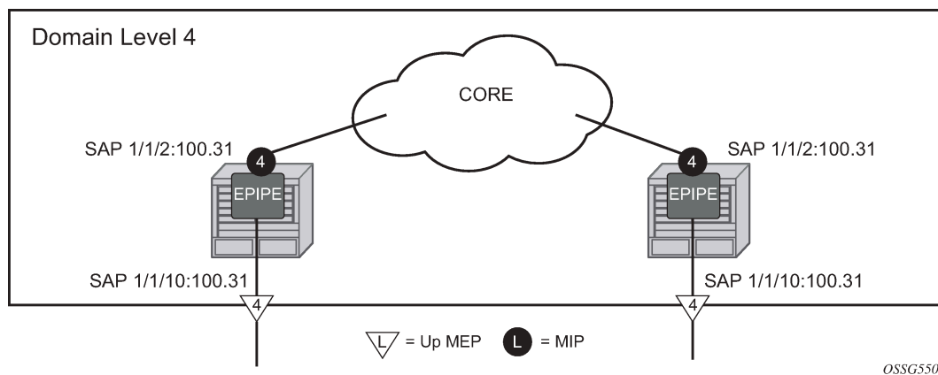
Figure 42: MIP creation default
