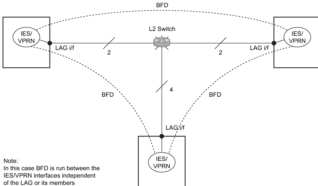
Figure 56: BFD over LAG and VSM interfaces
