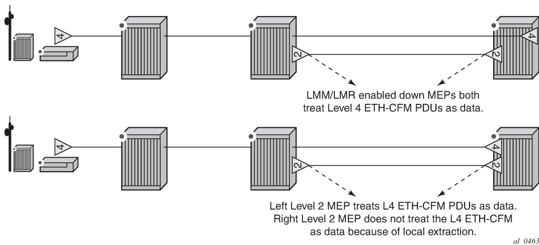
Figure 49: Mismatched LMM statistical counters
