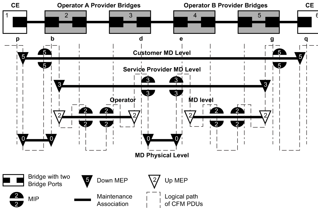
Figure 43: MEP, MIP, and MD levels
