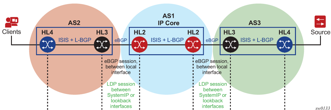
Figure 57: ASBR and EBGP
