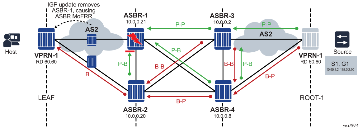
Figure 74: Failure scenario 2
