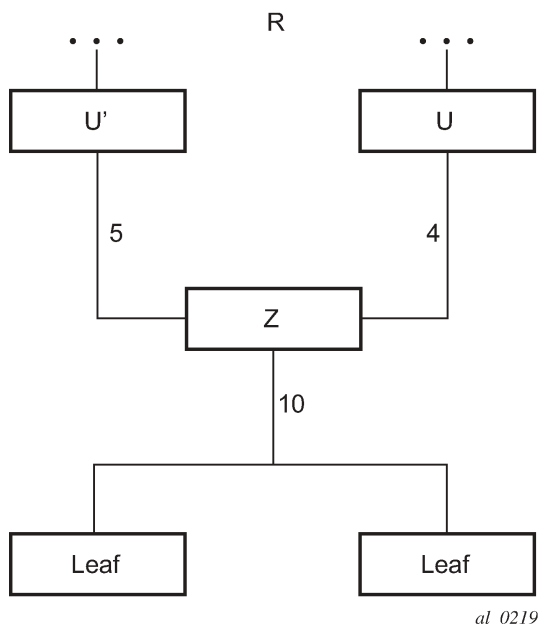
Figure 77: mLDP LSP with backup upstream LSR nodes
