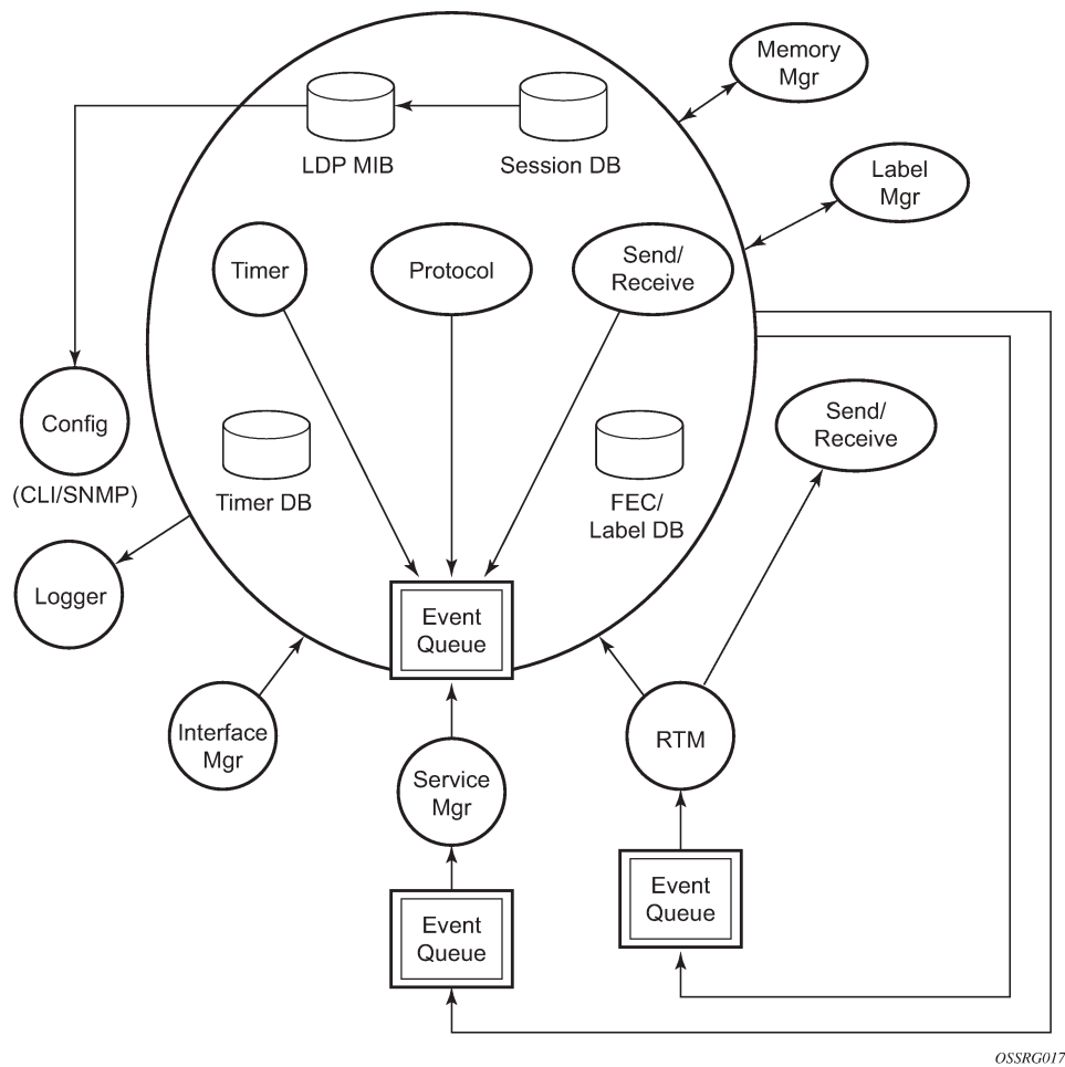
Figure 39: Subsystem interrelationships
