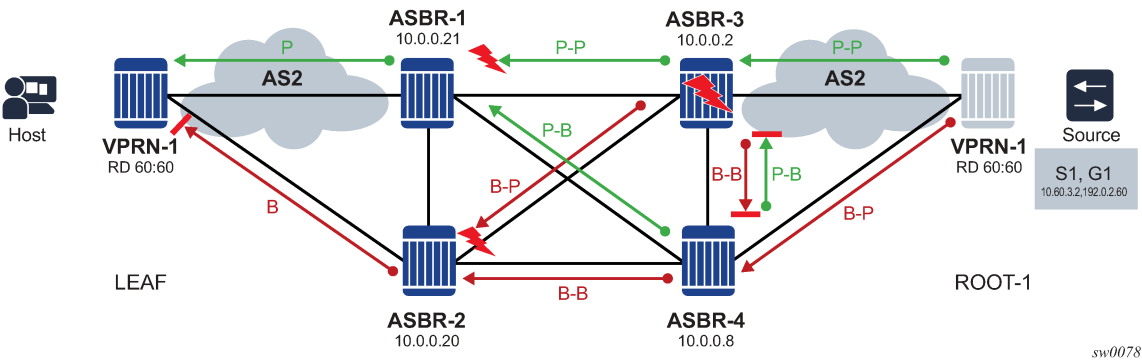
Figure 76: ASBR-3 failure
