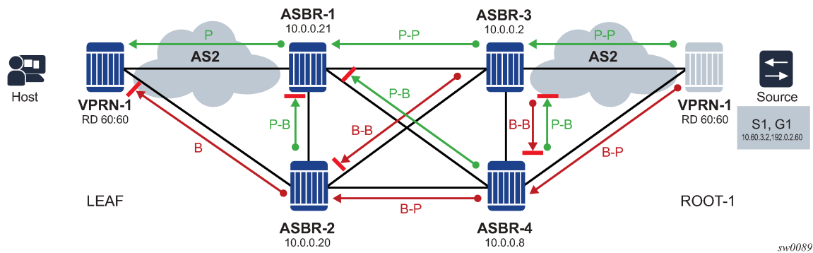
Figure 72: Traffic flow
