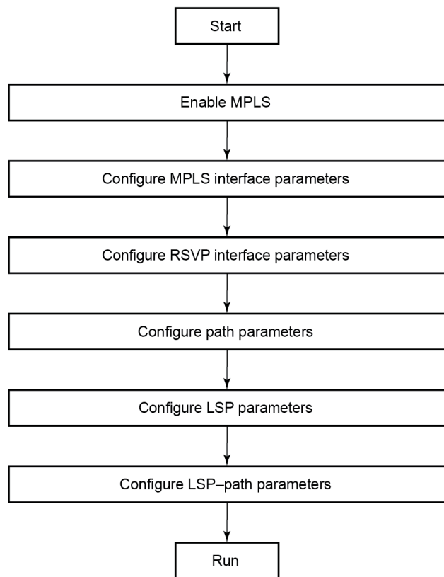
Figure 38: MPLS and RSVP configuration and implementation flow
