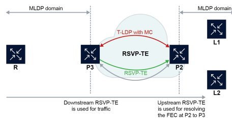
Figure 15: FEC T-LDP session selection
