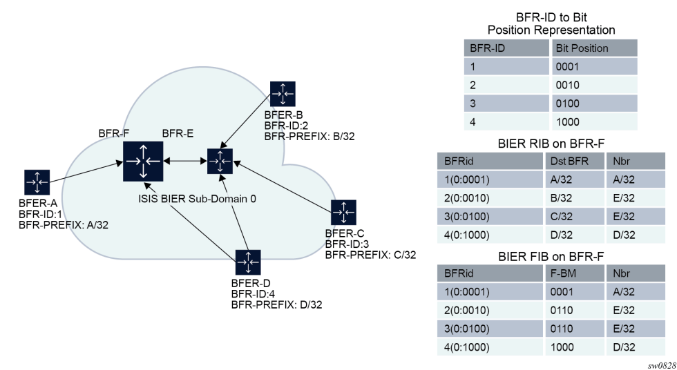
Figure 31: BIER forwarding
