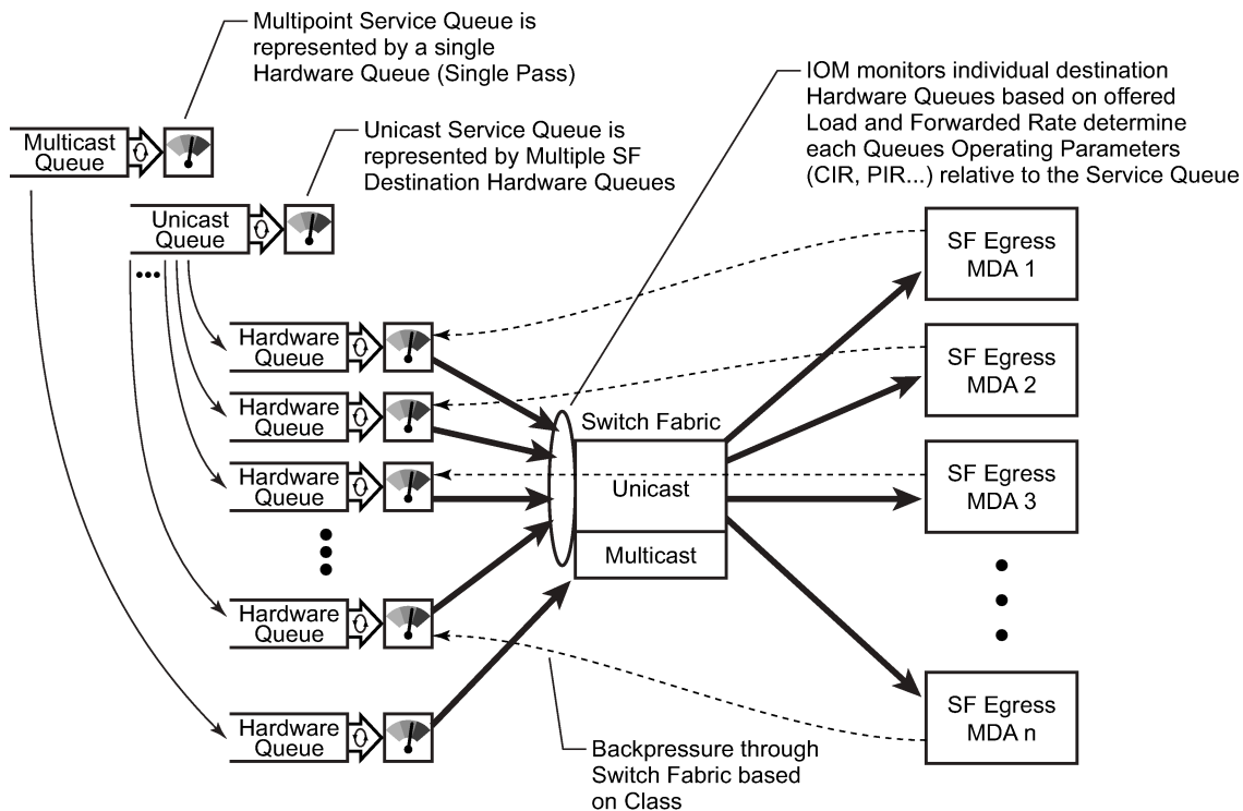
Figure 39: Unicast service queue mapping to multiple destination-based hardware queues
