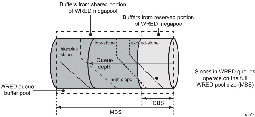
Figure 3: WRED queue: pool-per-queue mode
