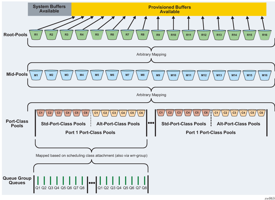
Figure 44: HSQ buffer pool hierarchy
