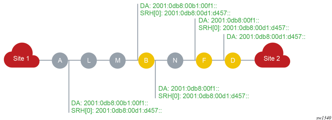
Figure 56: Transit routers in micro-segment SRv6
