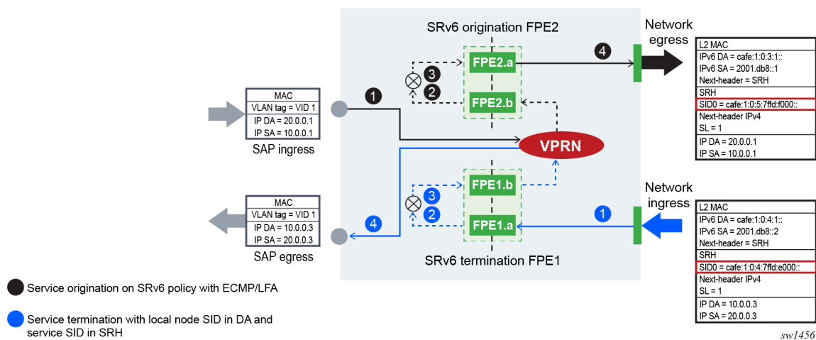
Figure 47: Packet walk-through showing service origination and termination with SRv6 FPE
