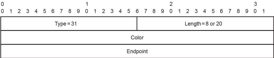
Figure 64: Extended Association ID TLV format
