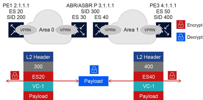
Figure 98: Services Option A
