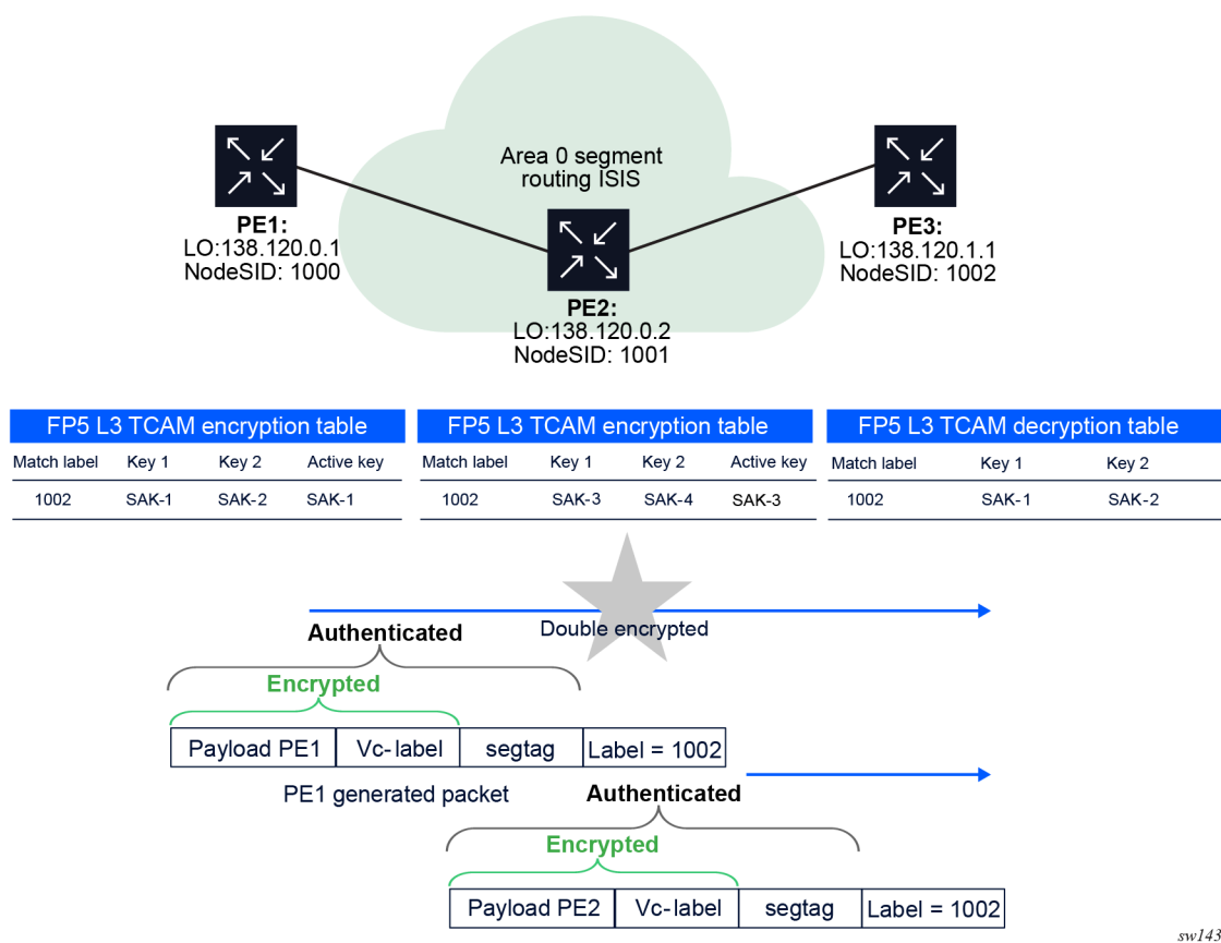
Figure 93: ANYsec double-encryption scenario
