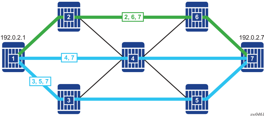
Figure 30: Network example with two SR policies
