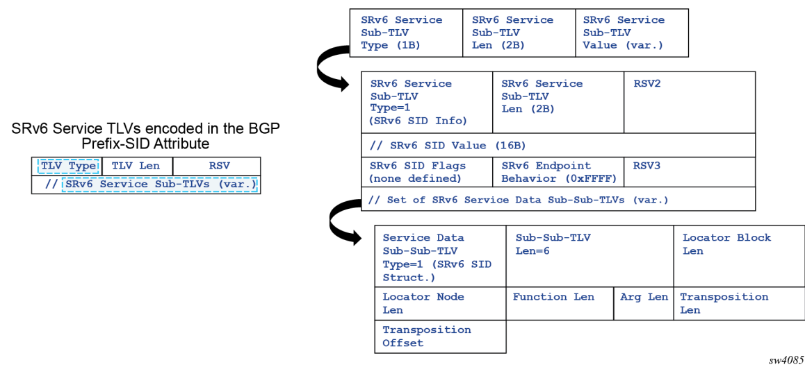
Figure 43: SRv6 service TLV format
