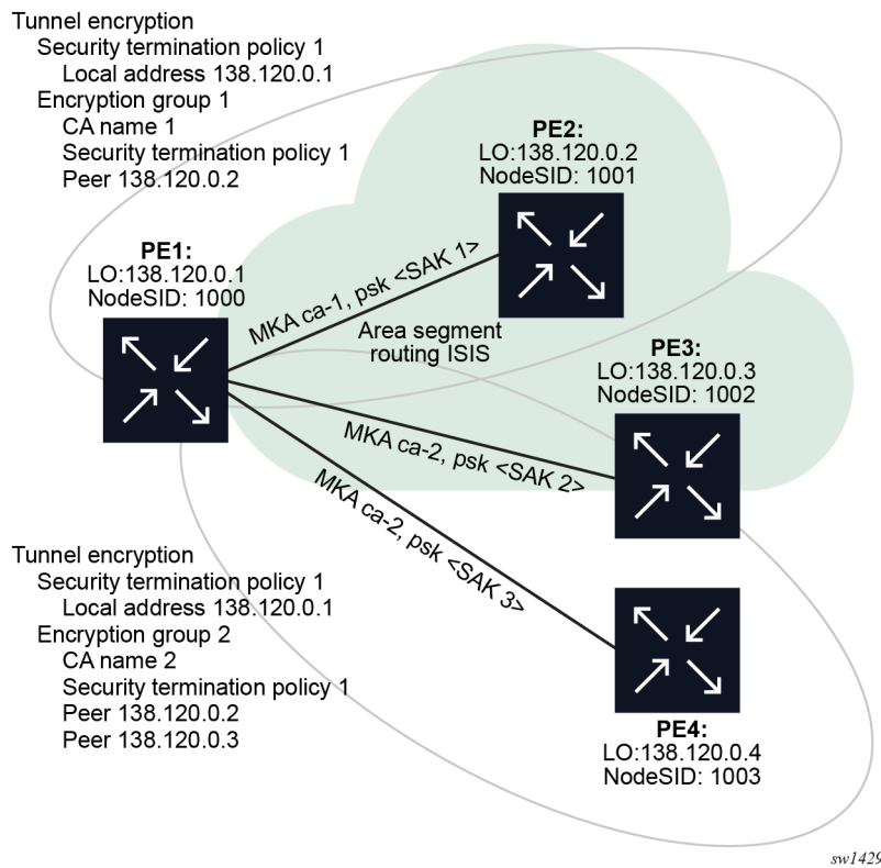
Figure 91: ANYsec tunnel encryption implementation
