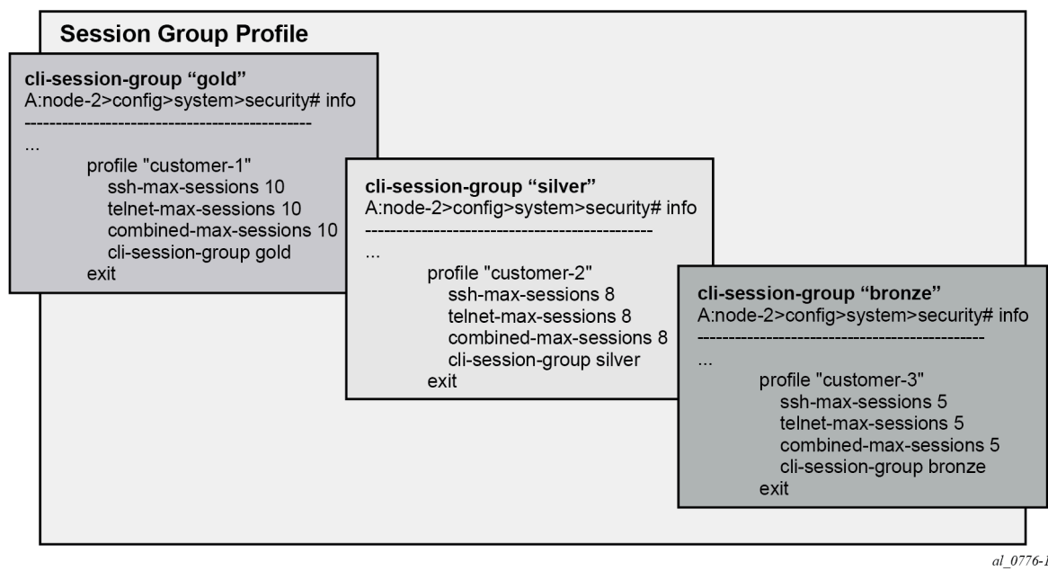
Figure 16: Hierarchy of classic CLI session group profiles
