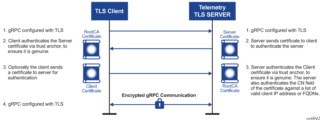
Figure 11: Session authentication using TLS
