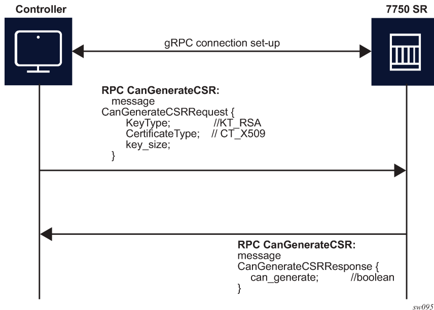
Figure 35: RPC CanGenerateCSR message flow
