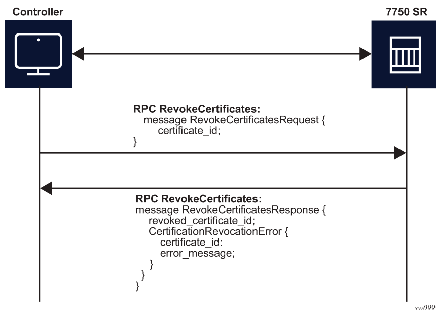
Figure 42: RPC RevokeCertificates message flow
