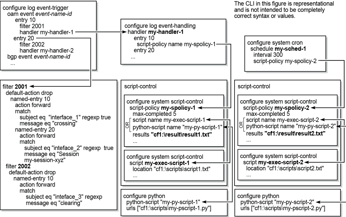
Figure 25: EHS object handling (MD-CLI)
