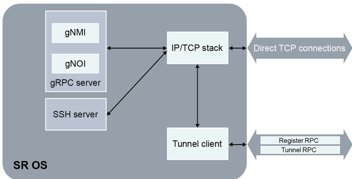
Figure 45: Internal SR OS architecture
