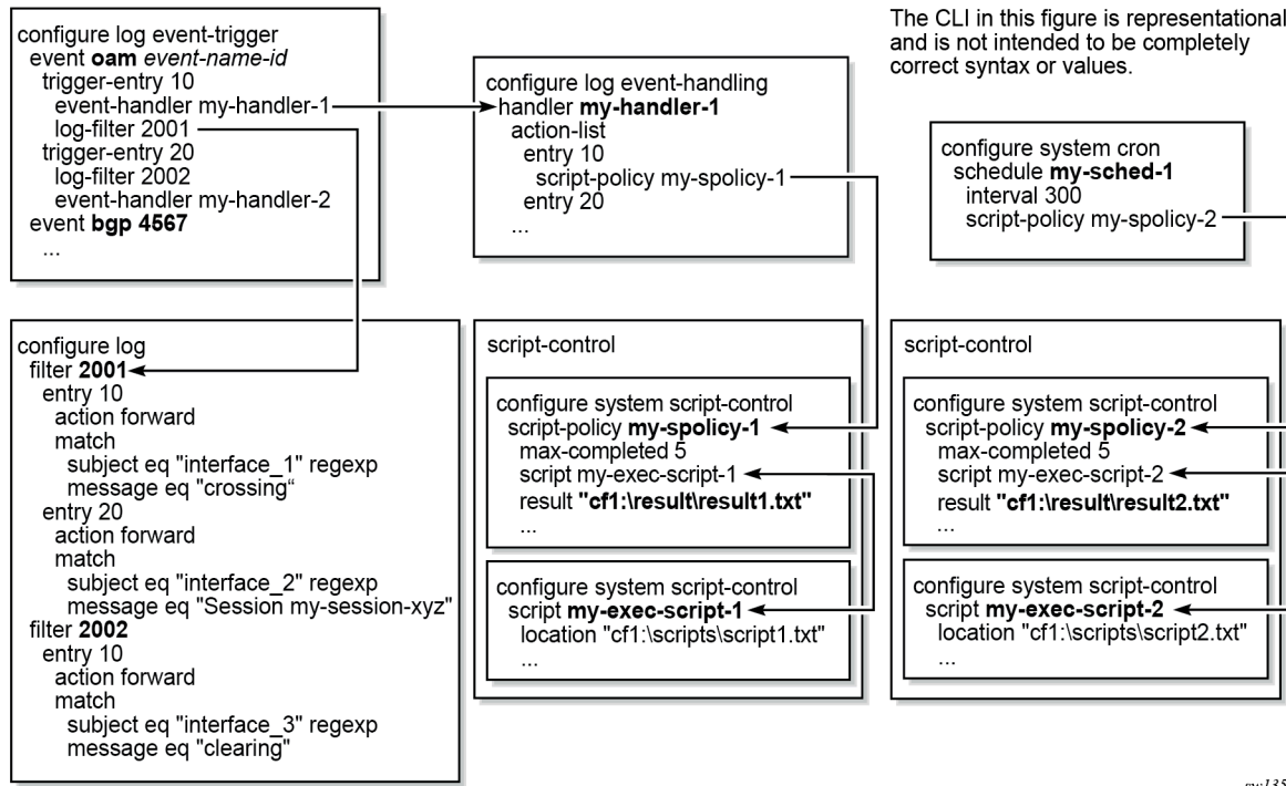
Figure 26: EHS object handling (classic CLI)
