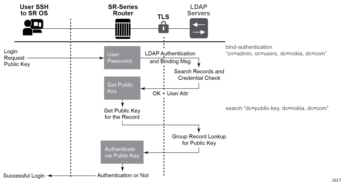
Figure 3: LDAP server and SR OS interaction for retrieving the public key
