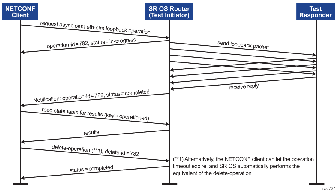
Figure 17: Asynchronous operation flow
