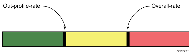
Figure 7: Profile marking
