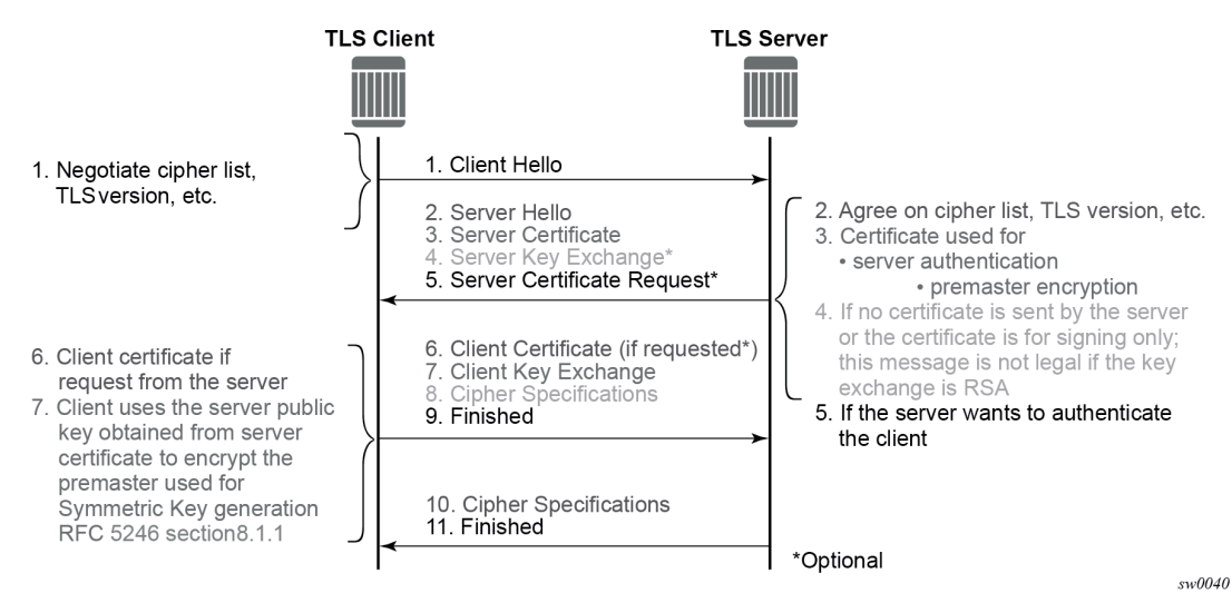
Figure 46: TLS handshake
