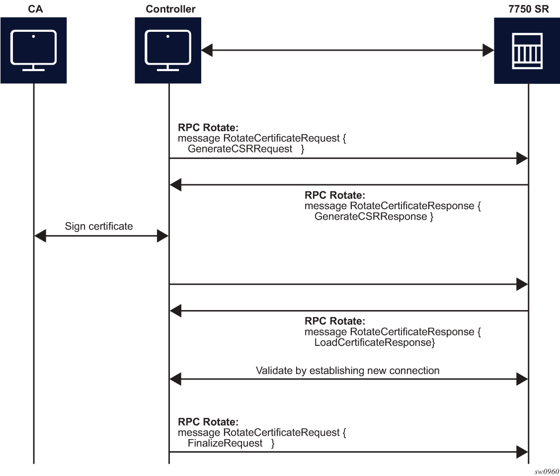
Figure 36: RPC Rotate message flow for CSRs generated on the SR OS node
