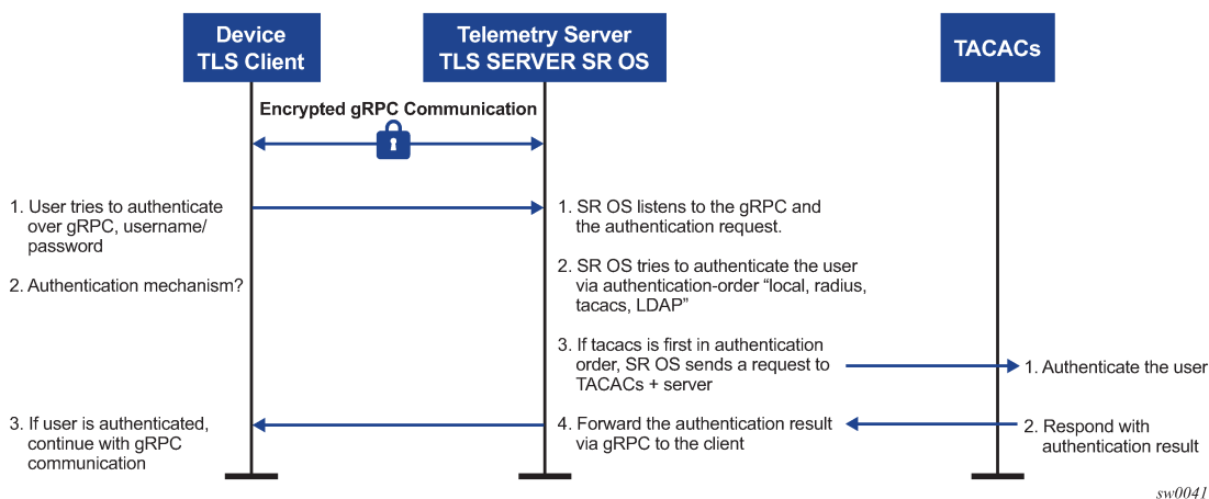
Figure 12: gNMI call authentication using SR OS
