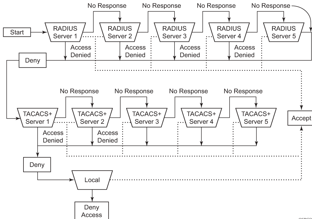
Figure 6: Security flow
