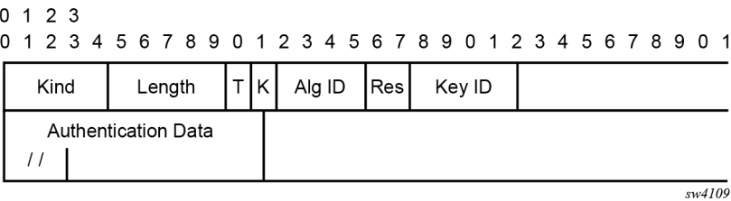
Figure 10: Packet format
