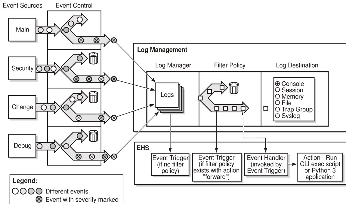
Figure 24: Event logging block diagram
