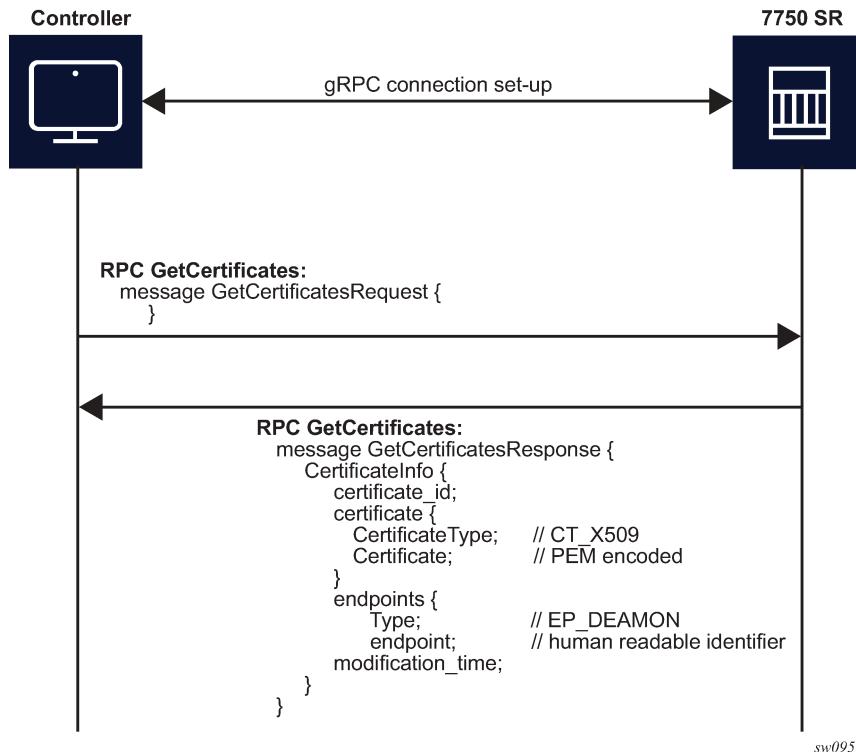
Figure 34: RPC GetCertificates message flow
