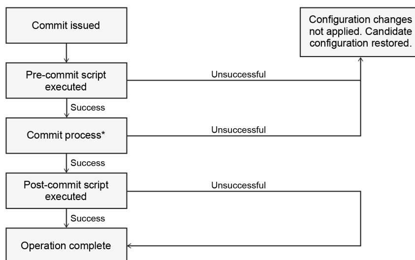
Figure 22: Commit operation
