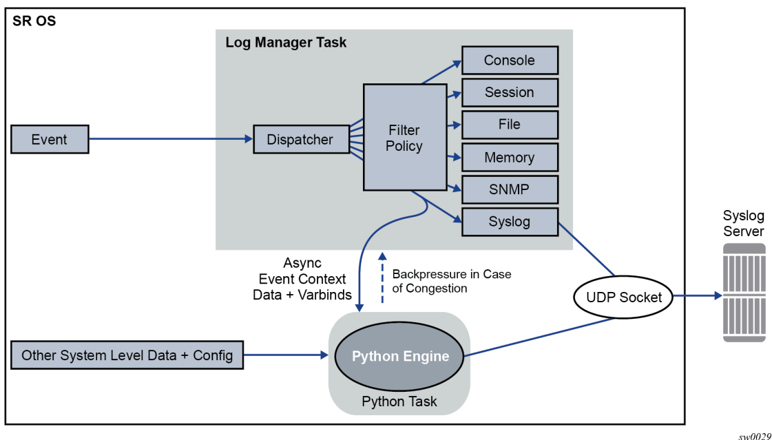
Figure 27: Interaction between the logger and the Python engine
