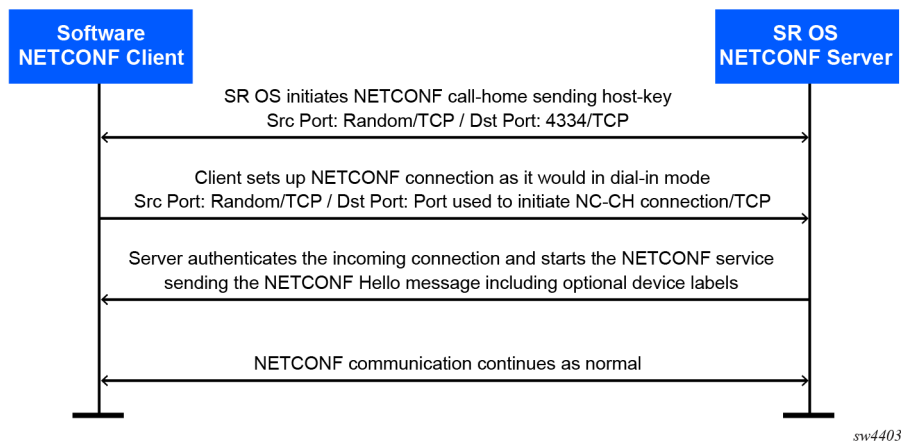
Figure 21: NETCONF call-home call flow
