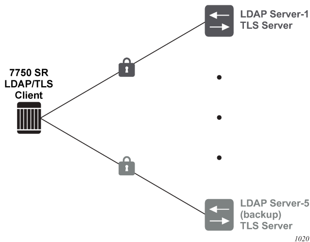
Figure 47: LDAP and TLS redundancy
