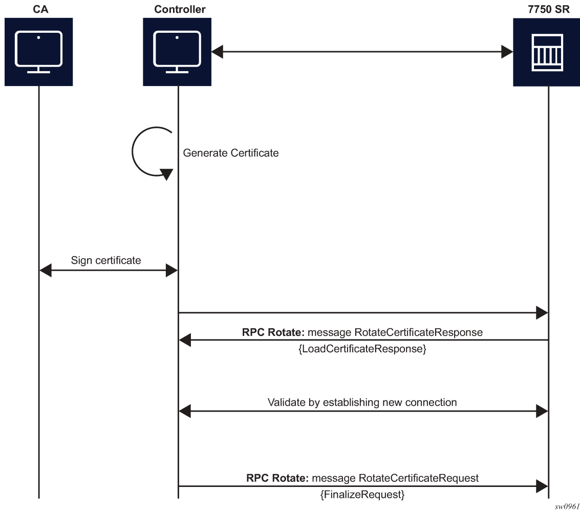
Figure 37: RPC Rotate message flow when CSRs are not generated on the SR OS node
