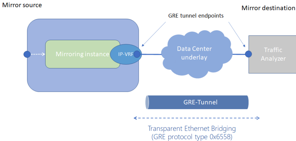
Figure 4: Mirroring to underlay
