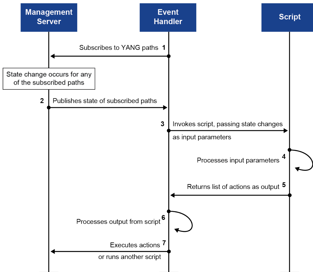
Figure 1: Event handler framework
